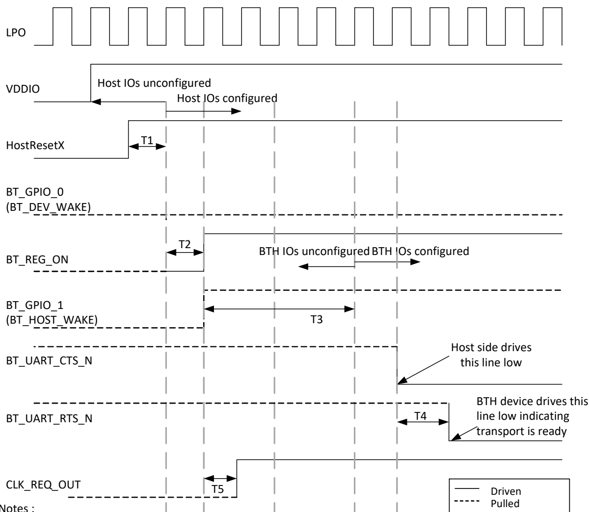
Figure 19. Startup Signaling Sequence
