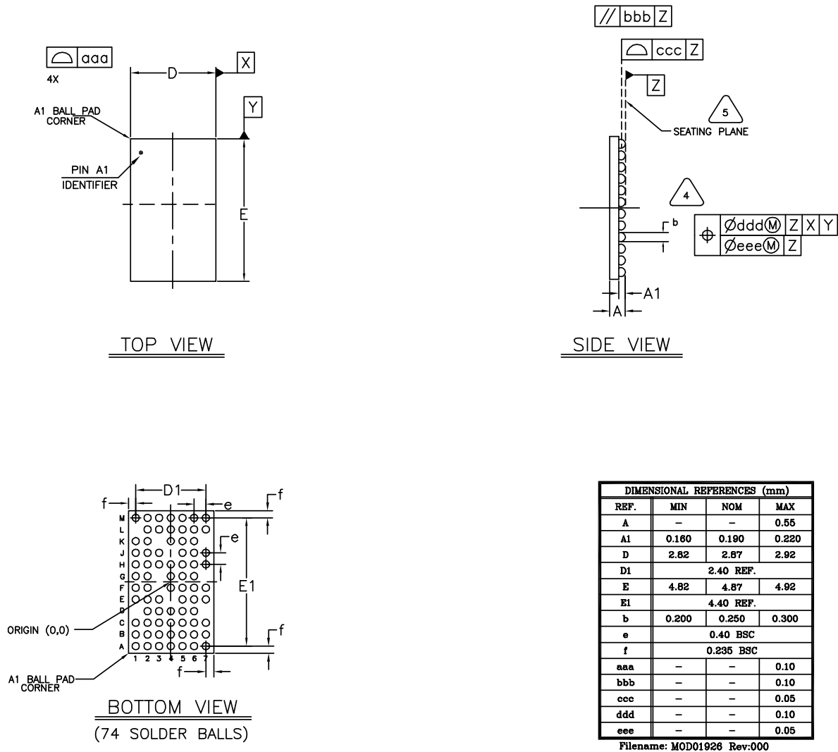
Figure 42. 74-Ball WLBGA Mechanical Information
