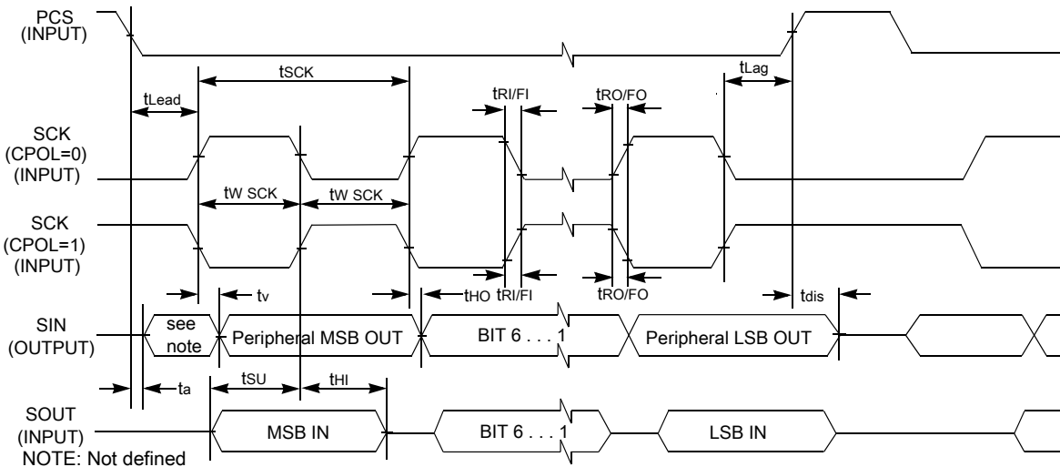
Figure 38. LPSPI Peripheral mode timing (CPHA = 1)
