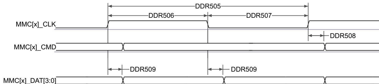
Figure 7-100. MMCSD1 – UHS-I DDR50 – Transmit Mode
