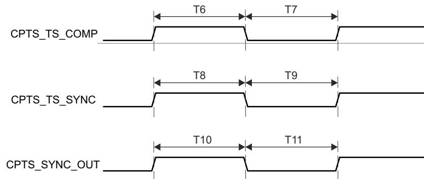
Figure 7-103. CPTS Output Switching Characteristics
