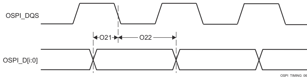
Figure 7-109. OSPI Timing Requirements – SDR, External Loopback Clock
