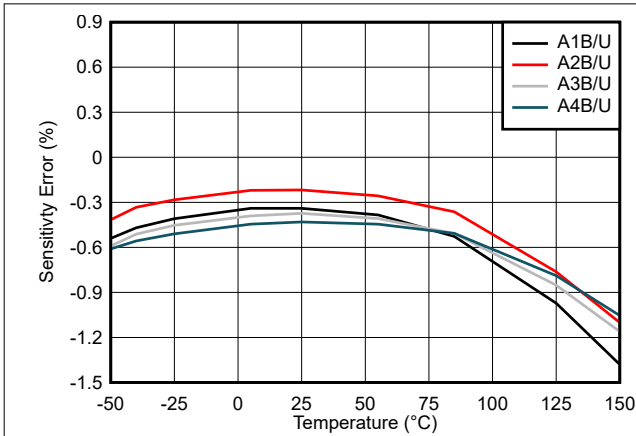
Figure 7-1. TMCS1108-Q1 Sensitivity Error vs. Temperature
