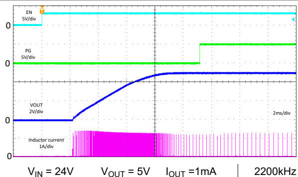
Figure 8-67. Start-up - Auto
