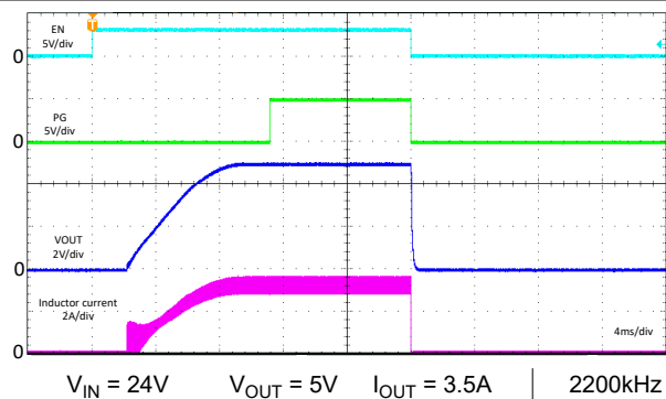
Figure 8-68. Start-up/Shutdown - FPWM
