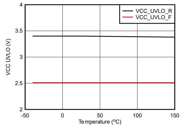
Figure 6-4. V_{CC} UVLO
