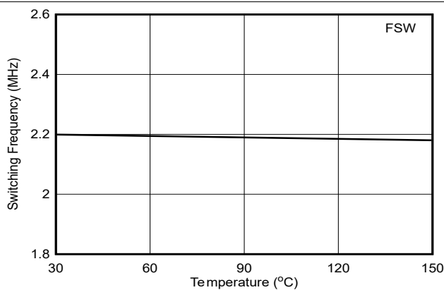
Figure 6-5. f_{SW} 2.2MHz
