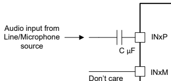
Figure 7-17. Single-ended AC-Coupled Input Connection (ADC_CHx_INSRC set to 2'b01 and ADC_CHx_CM_TOL set to 2'b00 or 2'b01 or 2'10)
