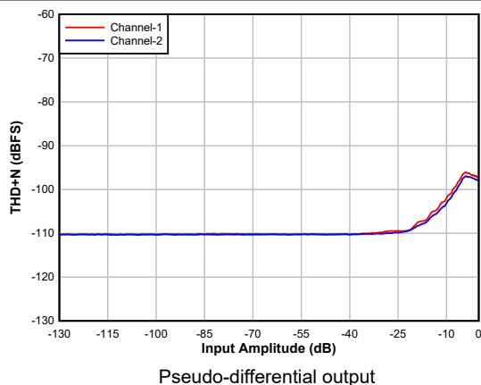
Figure 6-21. DAC THD+N Level vs Input
