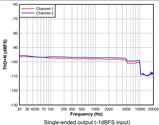
Figure 6-26. DAC THD+N Level vs Frequency
