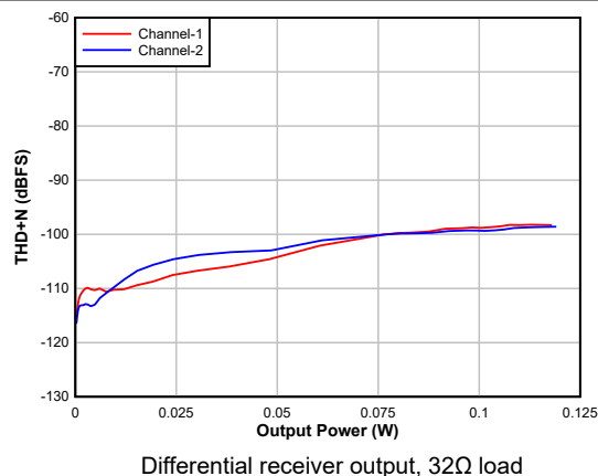
Figure 6-22. DAC THD+N Level vs output power
