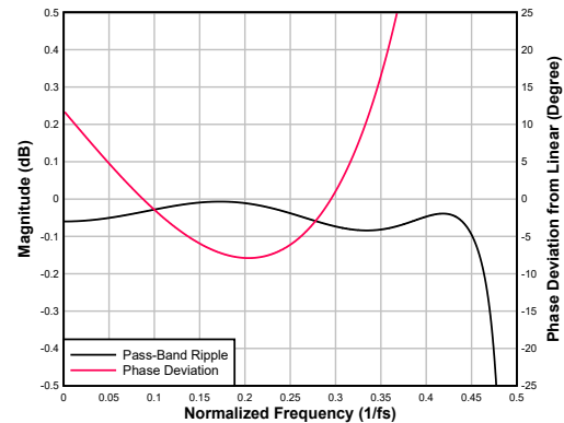
Figure 7-104. Ultra-Low-Latency interpolation Filter Pass-Band Ripple and Phase Deviation
