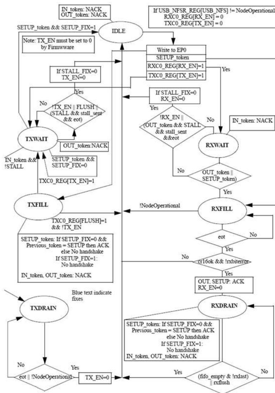
Figure 104: Endpoint 0 Operation
