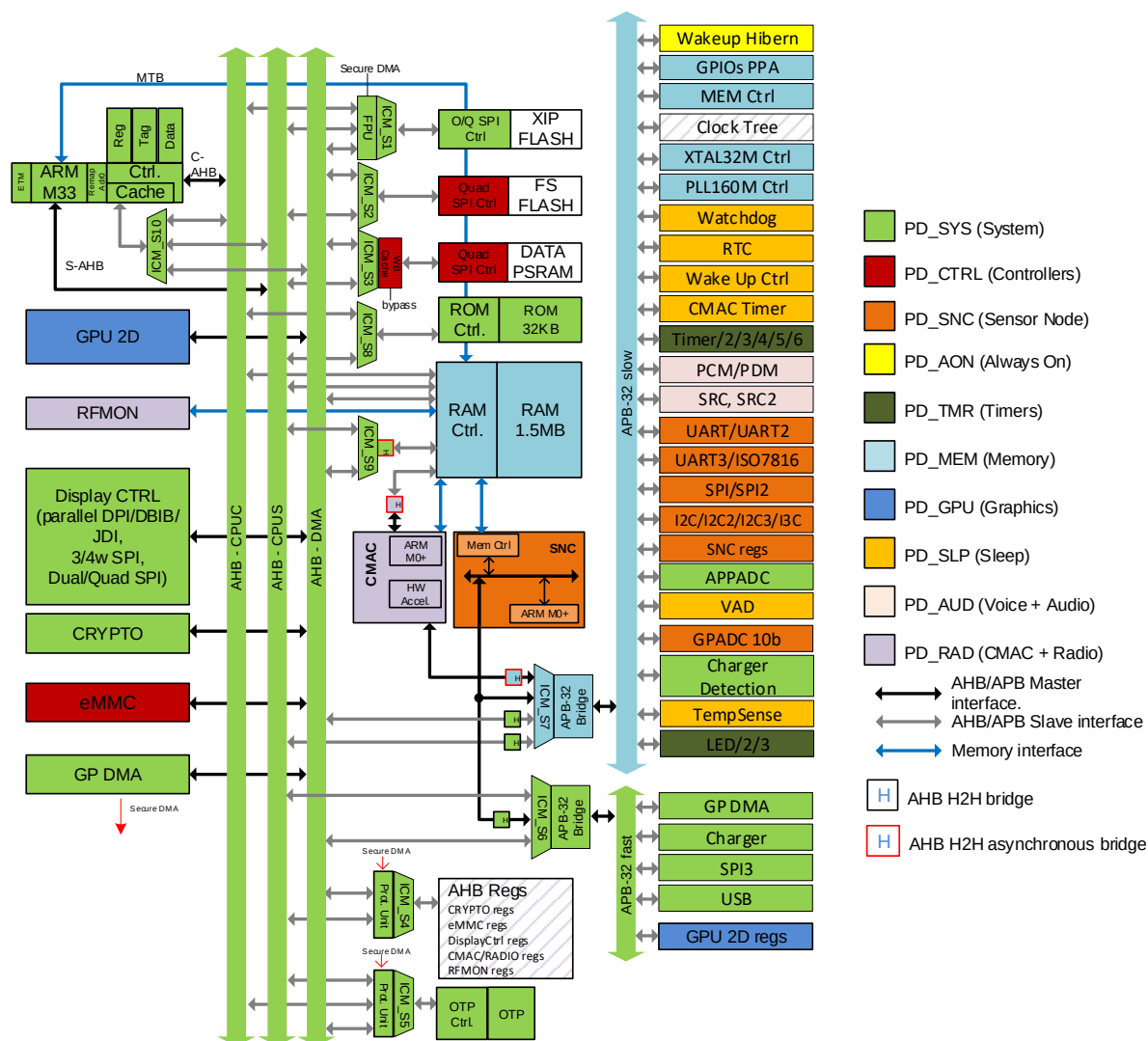
Figure 33: Bus Architecture
