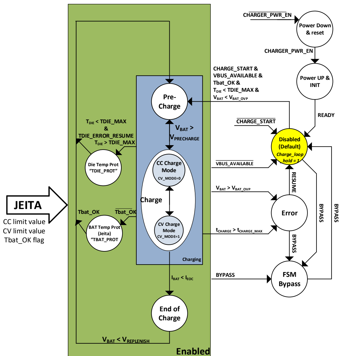
Figure 18: Charger FSM
