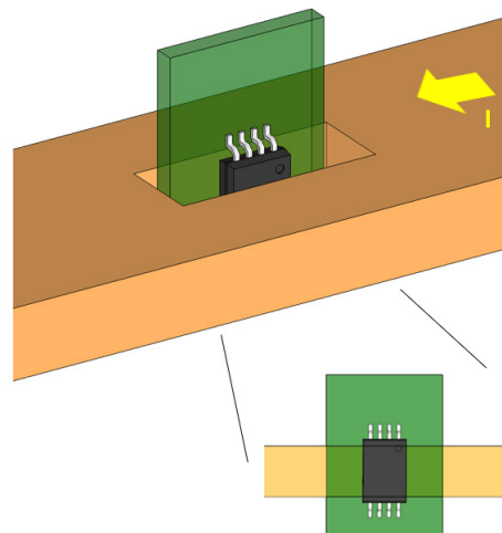
Figure 23: Vertical Slit Busbar Design
