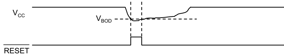
Figure 42-3. BOD33 Hysteresis OFF
