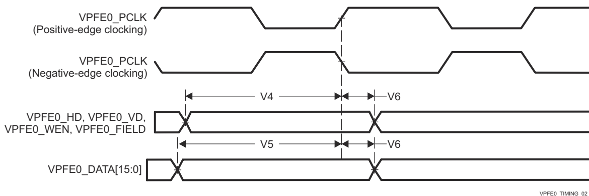
Figure 6-40. VPFE0 Timing Requirements
