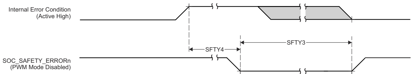
Figure 6-19. SOC_SAFETY_ERRORn Switching Characteristics
