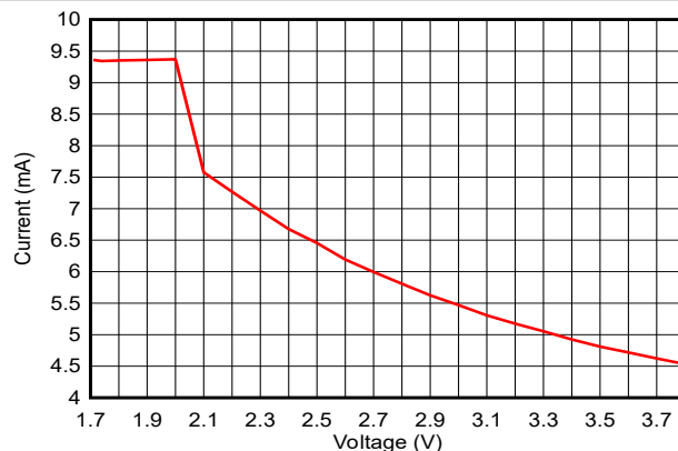
Figure 7-9. RX Current vs. Supply Voltage (VDD) (Bluetooth LE 1Mbps, 2.44GHz)
