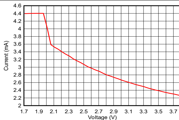
Figure 7-6. Active Mode (MCU) Current vs. Supply Voltage ( V_{DD} ) (Running CoreMark)
