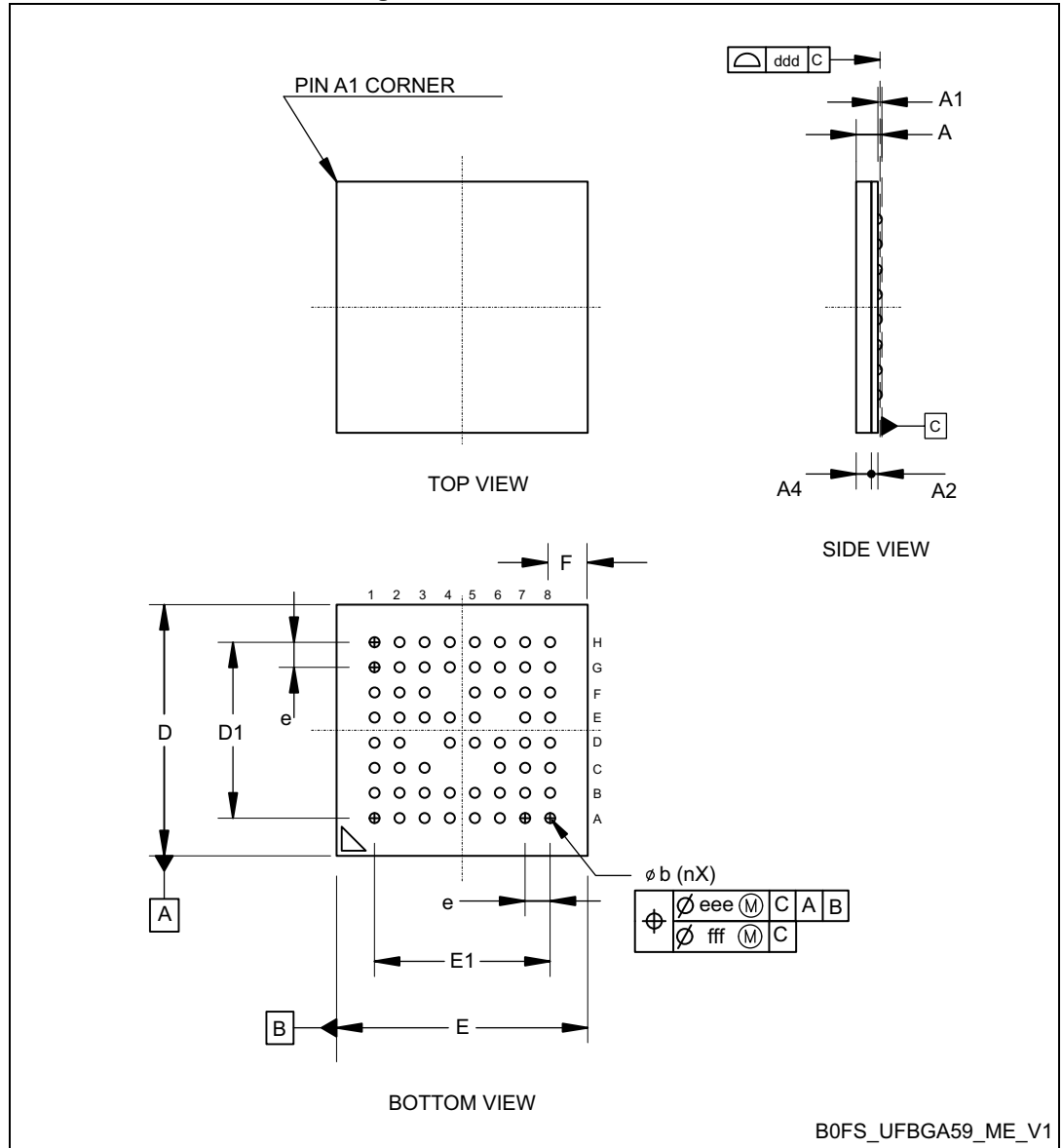
Figure 42. UFBGA59 - Outline
