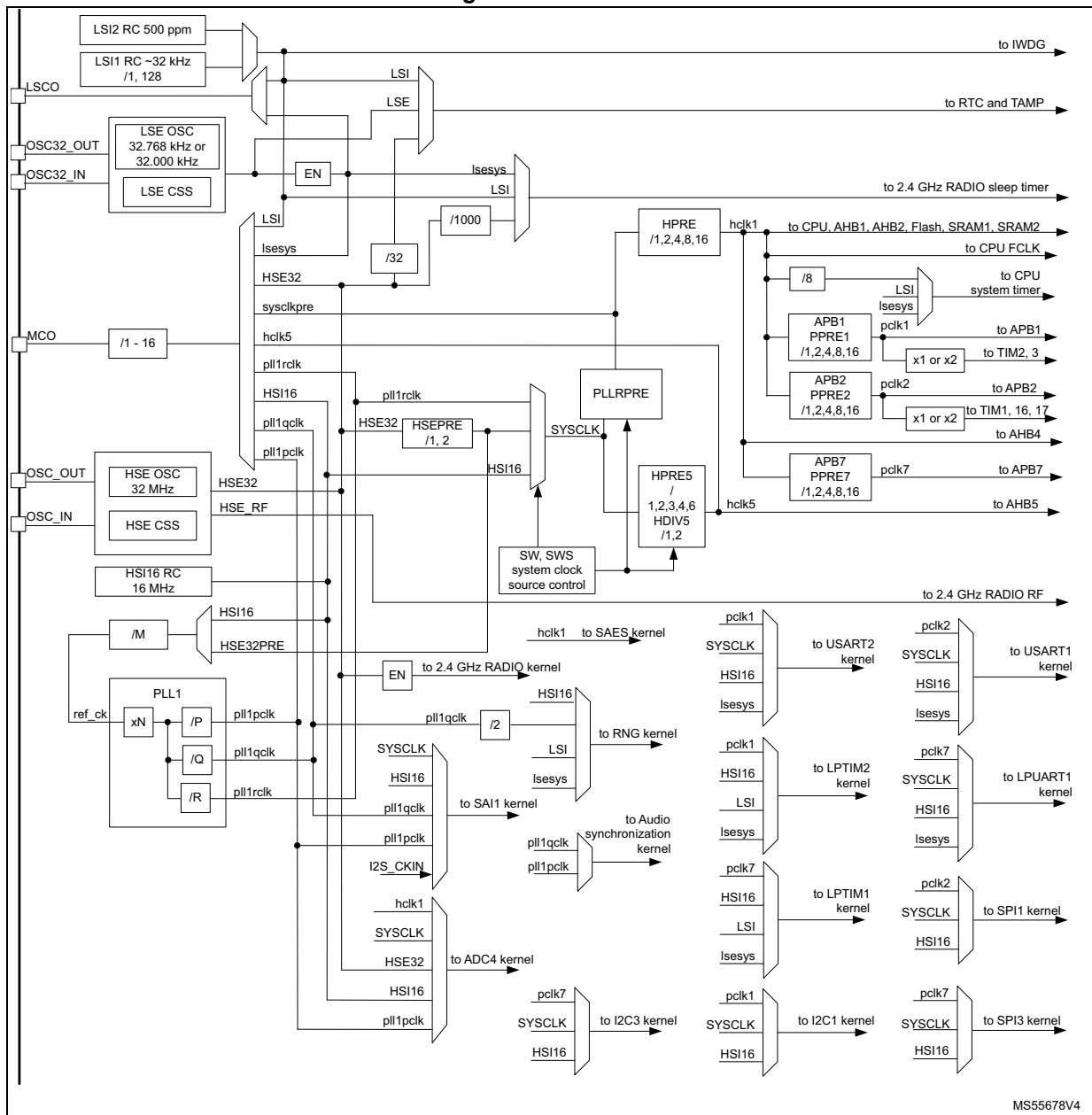
Figure 6. Clock tree
