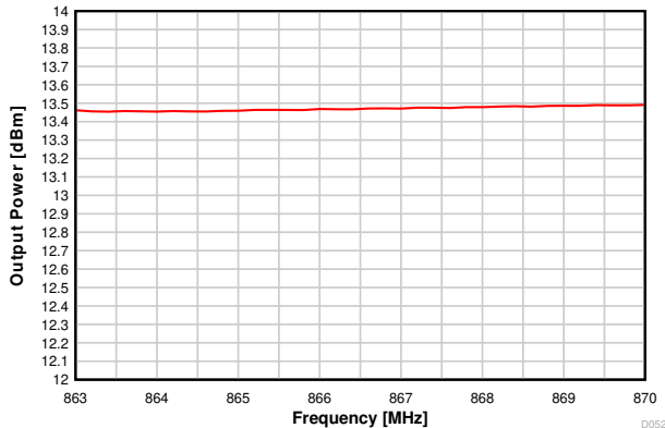
Figure 7-21. Output Power vs Frequency (50kbps, 868MHz)
