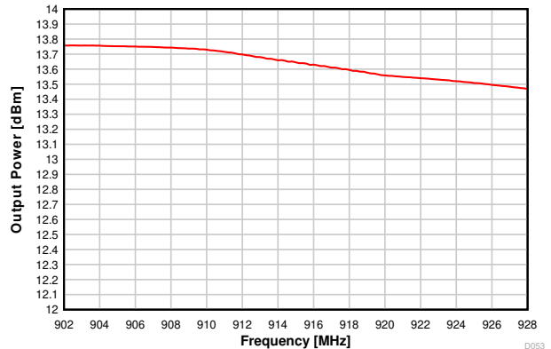
Figure 7-22. Output Power vs Frequency (50kbps, 915MHz)
