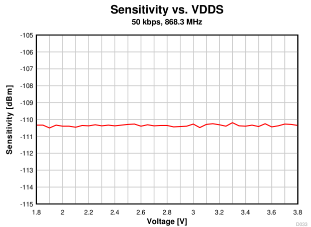
Figure 7-14. Sensitivity vs Supply Voltage (VDD5) (50kbps, 868.3MHz)
