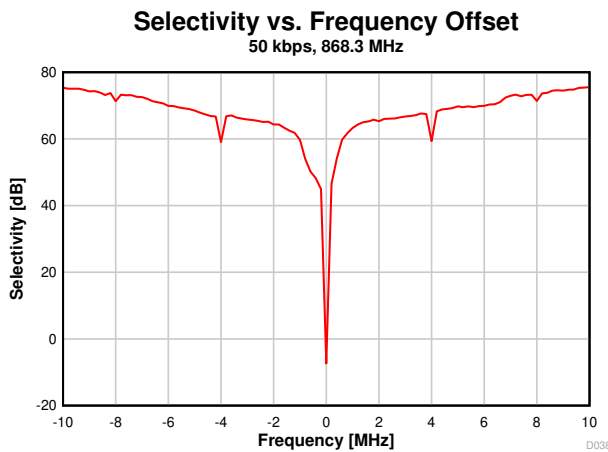
Figure 7-15. Selectivity vs Frequency Offset (50kbps, 868.3MHz)
