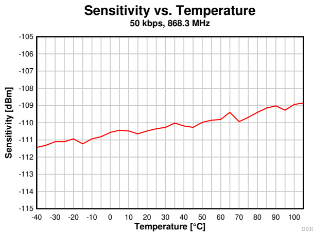
Figure 7-13. Sensitivity vs Temperature (50kbps, 868.3MHz)
