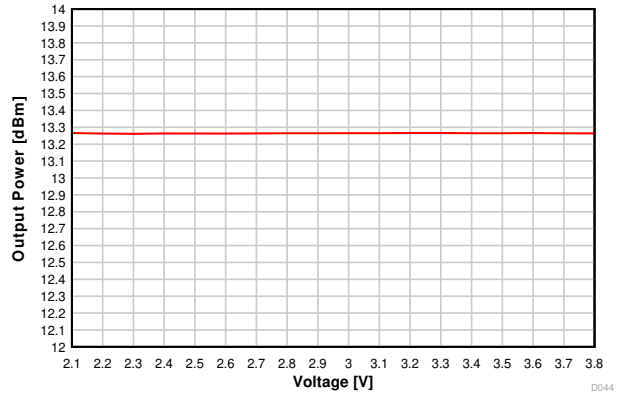
Figure 7-20. Output Power vs Supply Voltage (VDD5) (50kbps, 868.3MHz)
