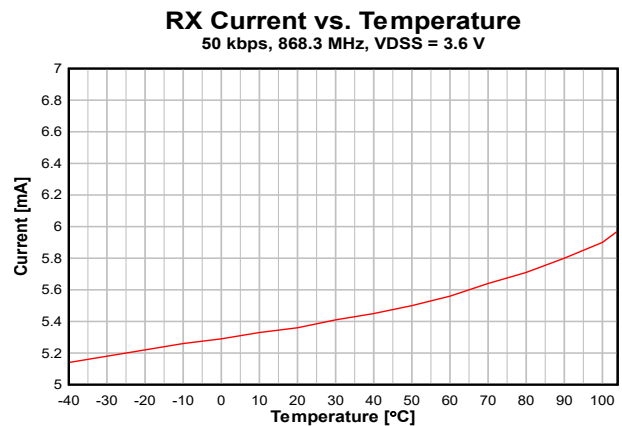
Figure 7-7. RX Current vs Temperature (50kbps, 868.3MHz, VDD5 = 3.6V)
