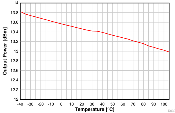
Figure 7-19. Output Power vs Temperature (50kbps, 868.3MHz)
