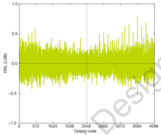
2.5 V Reference
