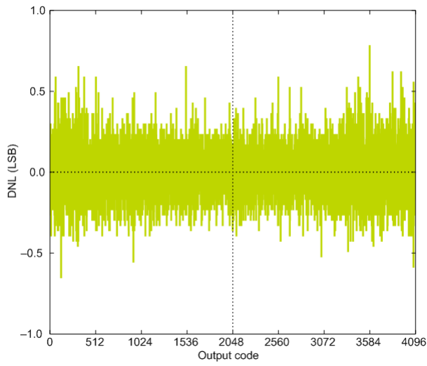
1.25 V Reference
