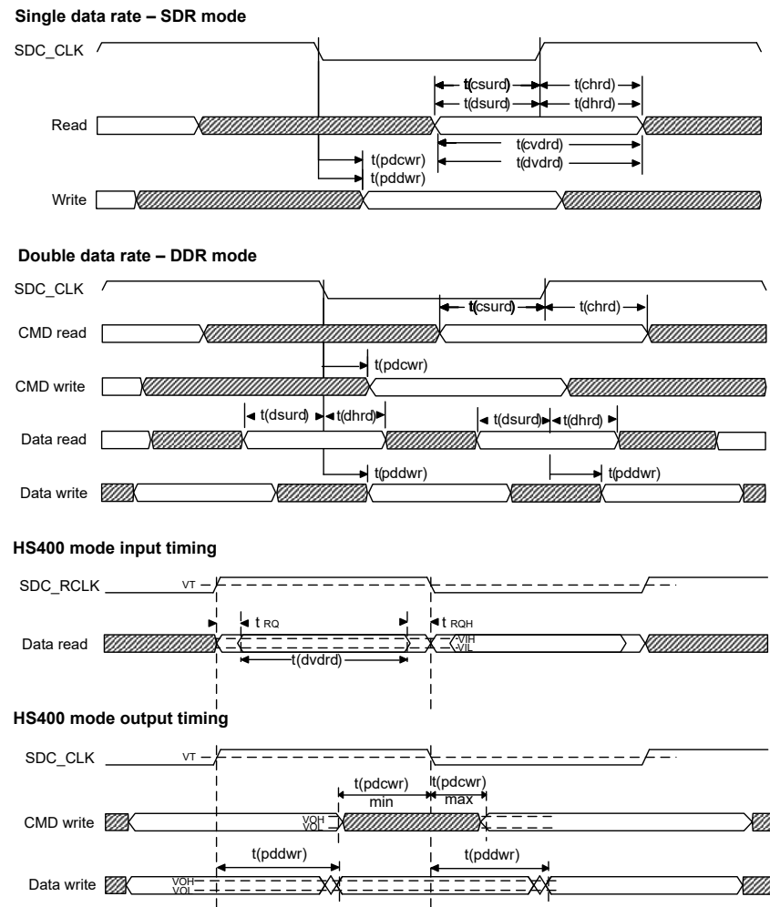
Figure 3-5 SD interface timing
