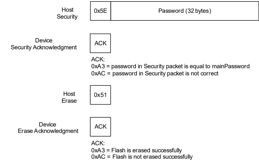
Figure 26: Security/Erase and Acknowledgment Packets
