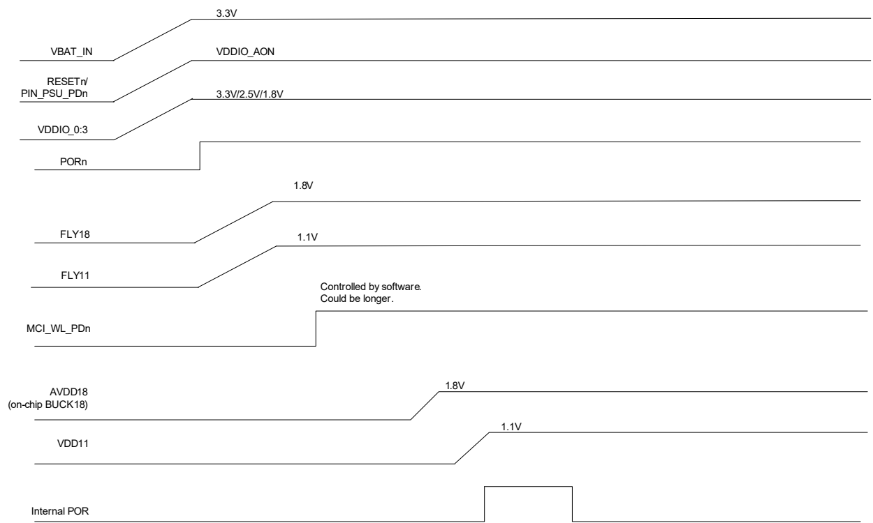
Figure 11: Power-Up Sequence
