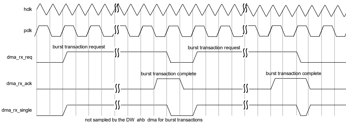
Figure 76: Burst Transaction, hclk = 2 \cdot pclk
