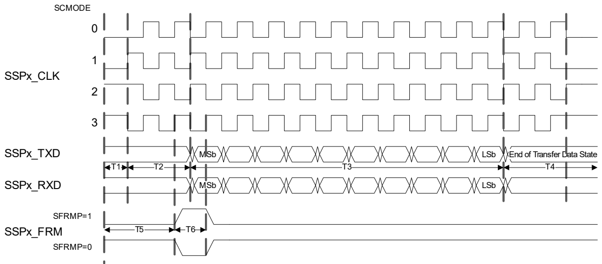
Figure 84: Programmable Serial Protocol Format
