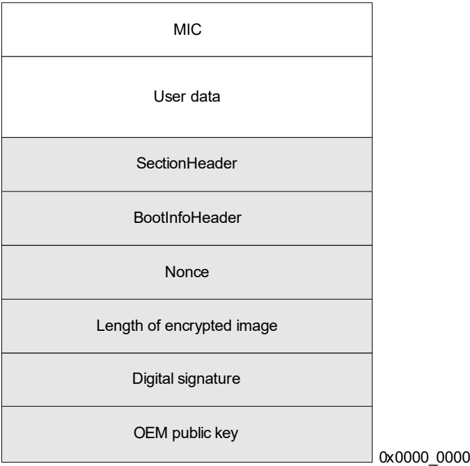
Figure 24: Code Image Memory Mapping
