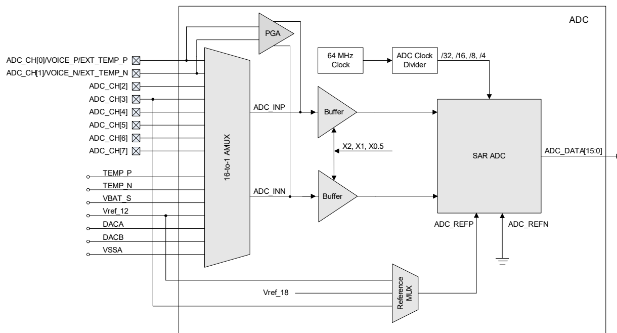
Figure 104:ADC Block Diagram
