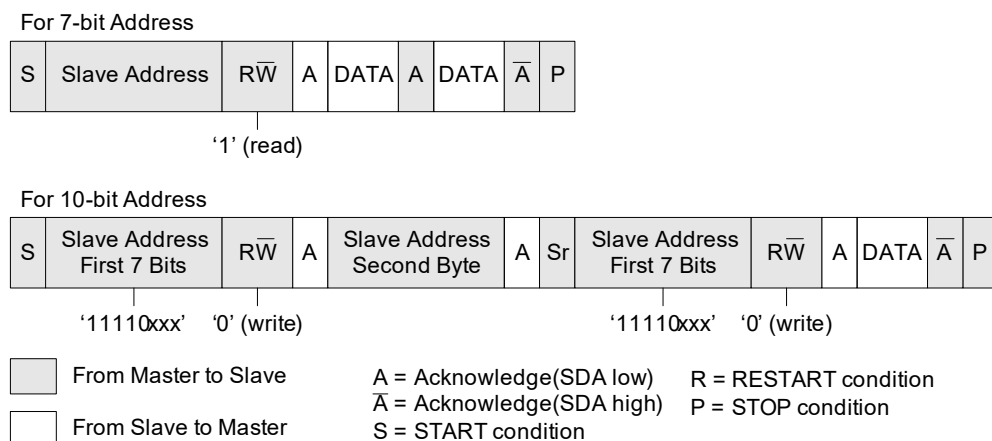
Figure 72: Master-Receive Protocol
