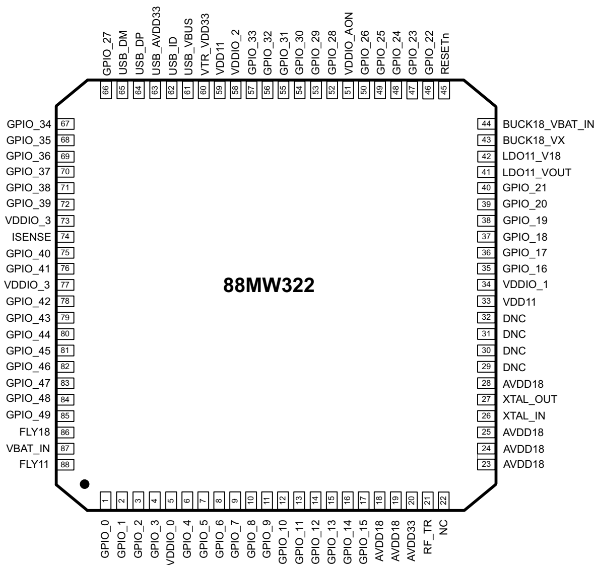
Figure 4: Pinout—88-Pin QFN 1
