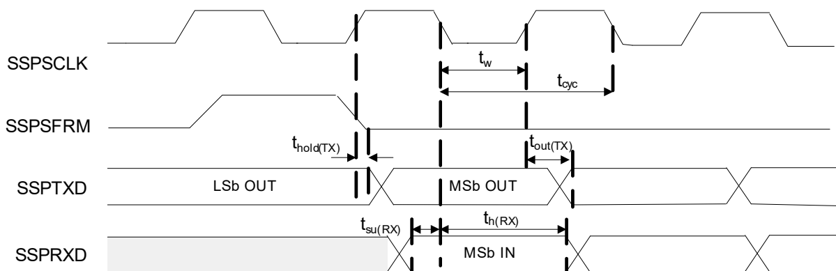
Figure 114: SSP Serial Frame Format Timing Diagram
