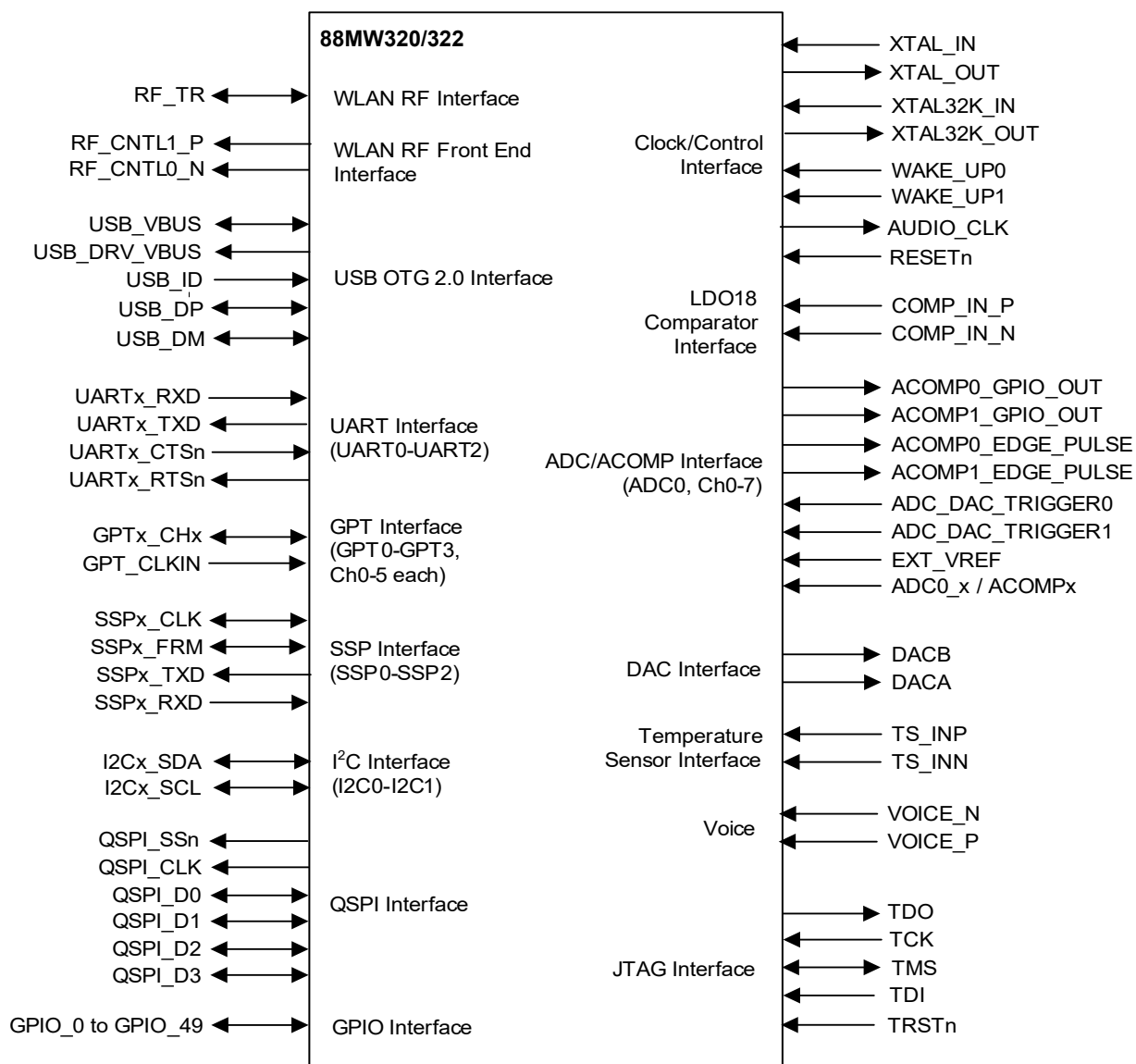
Figure 2: Signal Diagram 1 2 3 4
