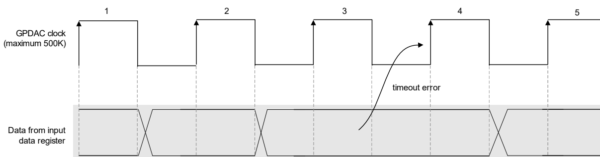
Figure 106: Synchronous Mode
