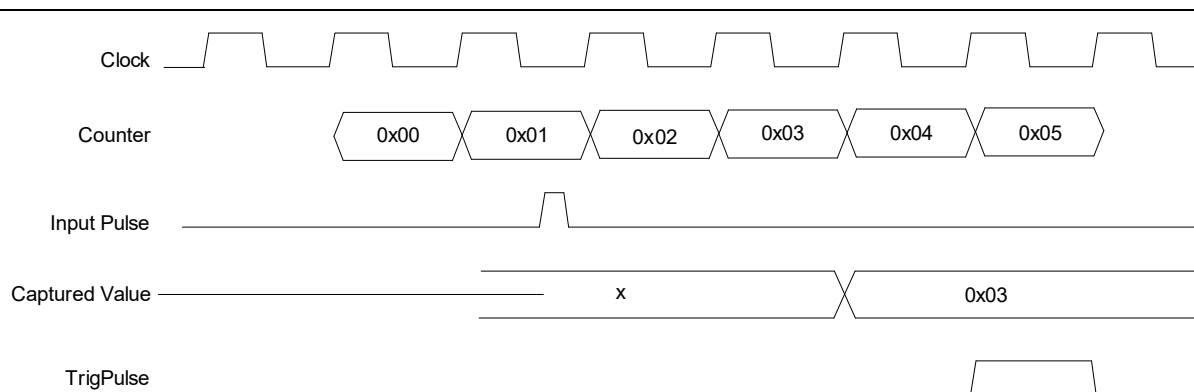
Figure 48: Input Capture Timing
