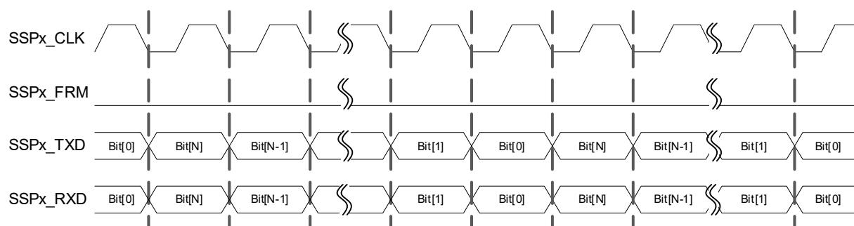
Figure 81: Motorola SPI Frame Protocol (Multiple Transfers)
