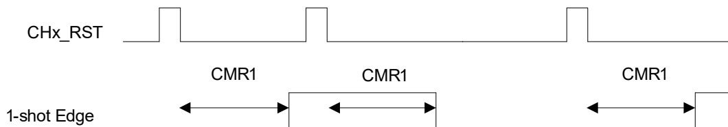
Figure 50: 1-Shot Edge Timing
