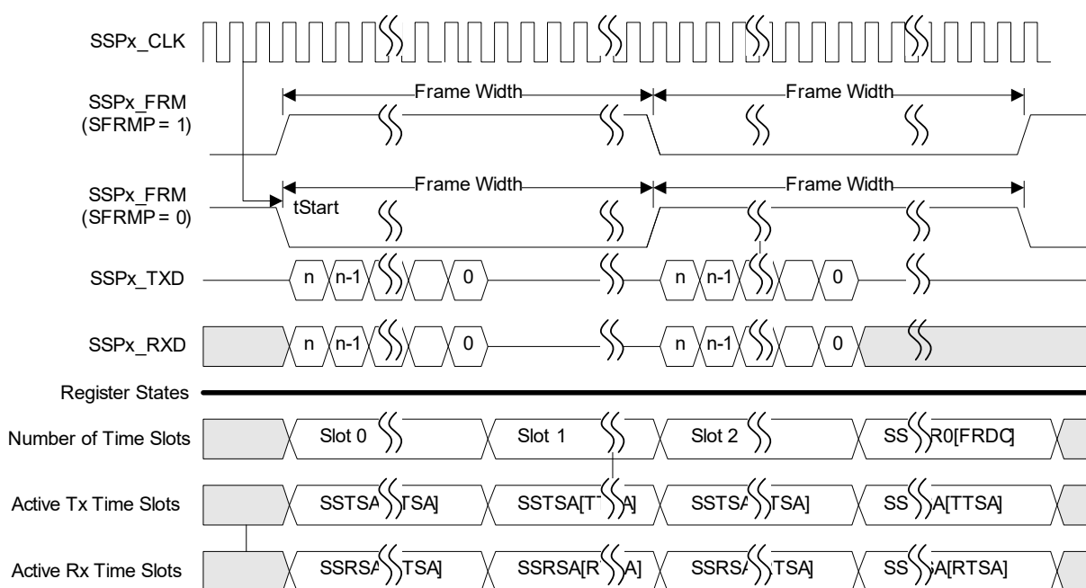
Figure 92: Network Mode and PSP Frame Format
