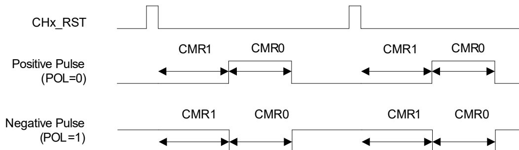
Figure 49: 1-Shot Pulse
