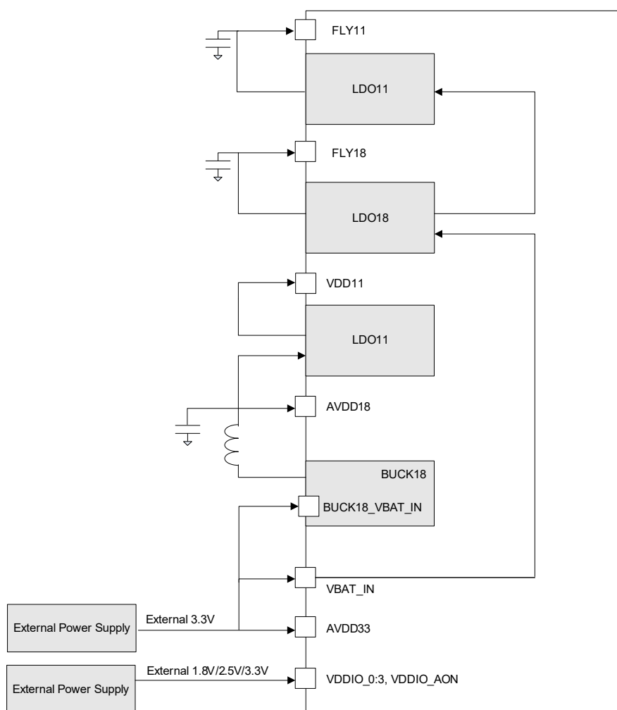
Figure 10: Power Option
