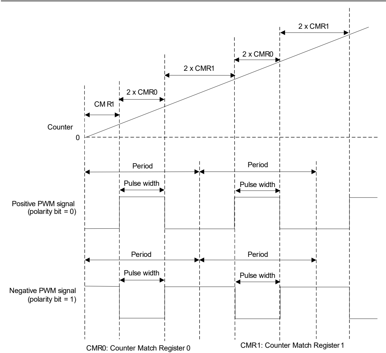
Figure 52: PWM Center-Aligned
