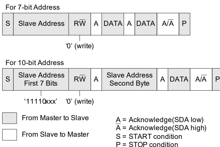
Figure 71: Master-Transmitter Protocol
