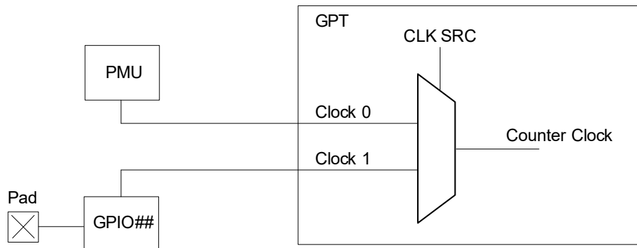
Figure 46: Clock Source Selection
