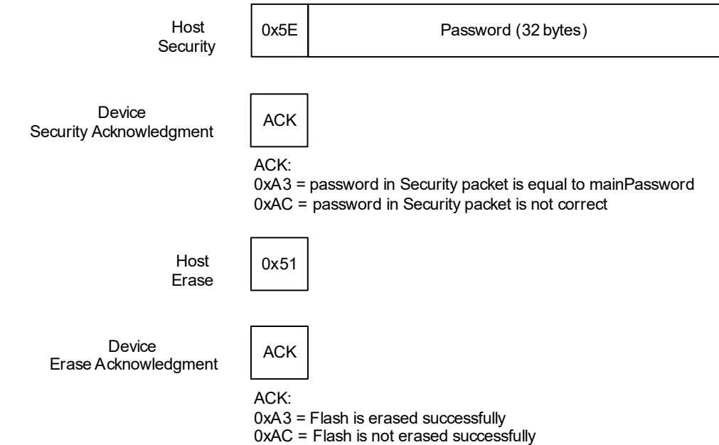
Figure 26: Security/Erase and Acknowledgment Packets
