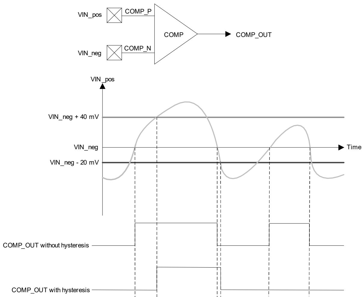
Figure 110: Comparator Hysteresis
