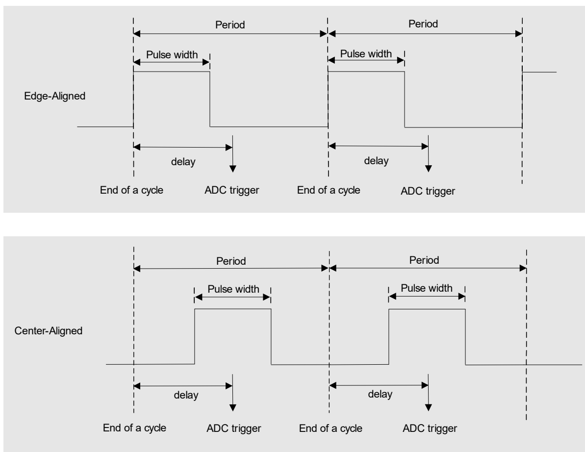
Figure 53: ADC Trigger for PWM Edge-Aligned and Center-Aligned
