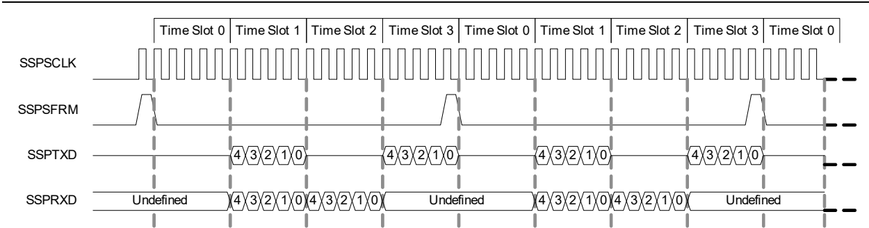
Figure 91: Network Mode (Example Using 4 Time Slots)
