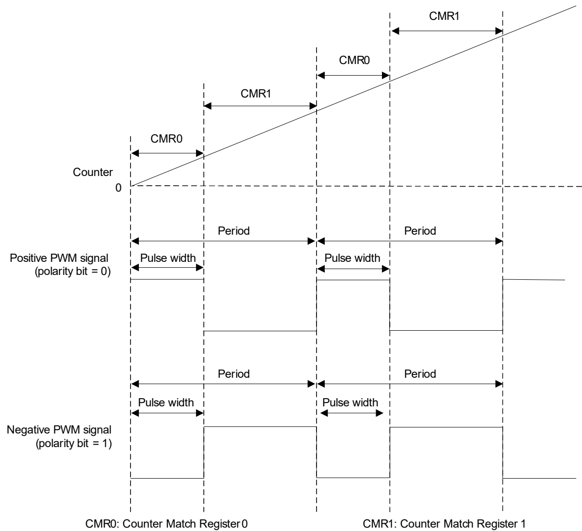
Figure 51: PWM Edge-Aligned
