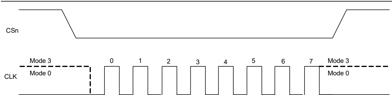
Figure 31: Flash Boot Mode, Timing
