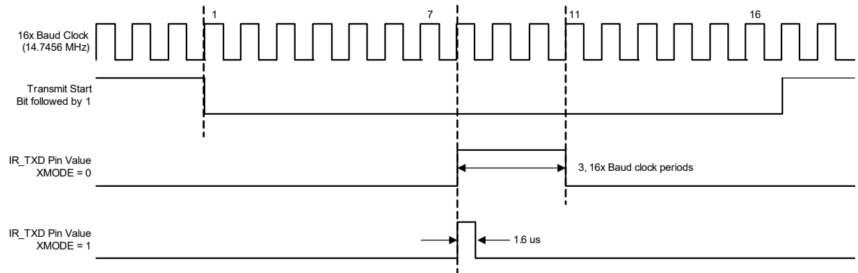
Figure 60: XMODE Example
