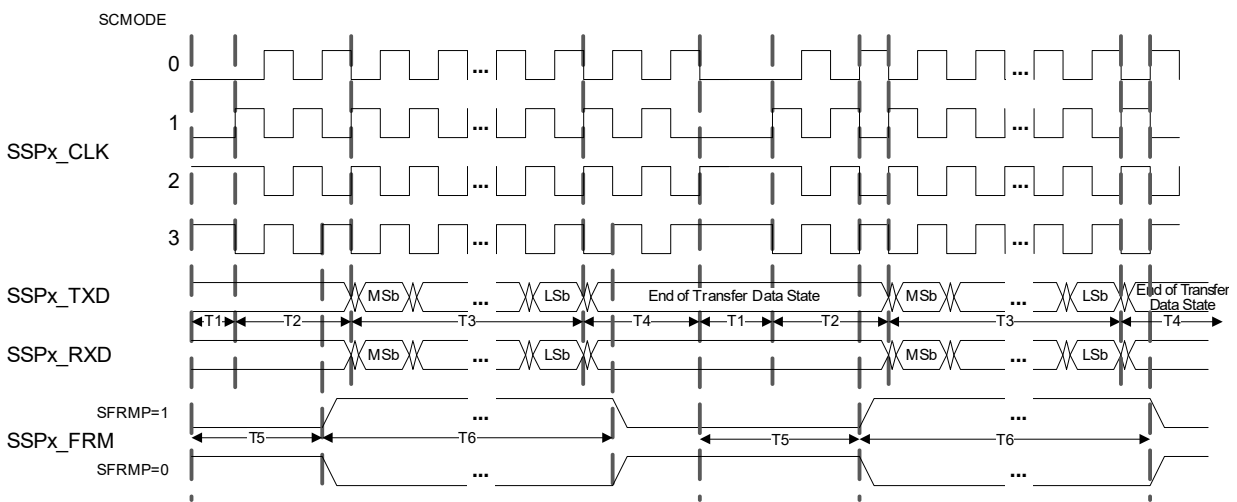
Figure 85: Programmable Protocol Format (Consecutive Transfers)
