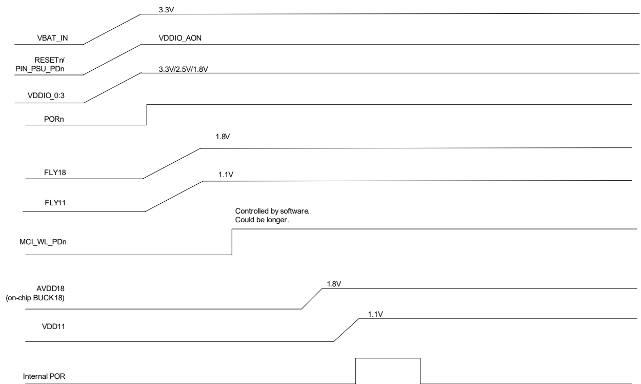
Figure 11: Power-Up Sequence
