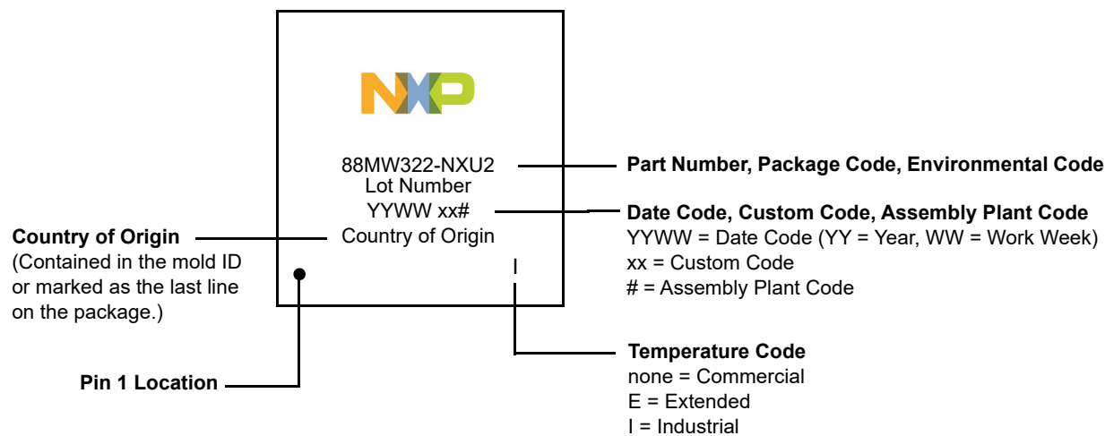
Figure 120:Package Marking and Pin 1 Location—88MW322
