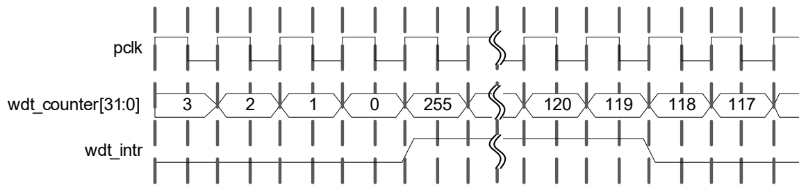
Figure 43: Interrupt Generation
