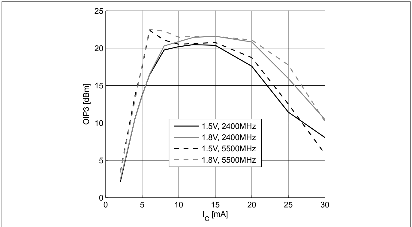
Figure 9 3rd order intercept point at output OIP_3 = f(I_C) , Z_S = Z_L = 50 \Omega , V_{CE} , f = parameter
