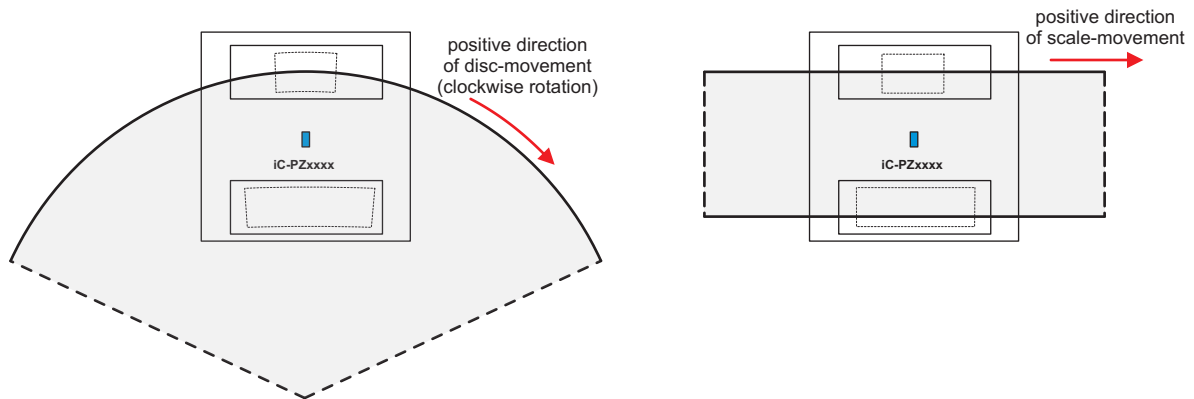
Figure 9: Definition of positive direction of movement
