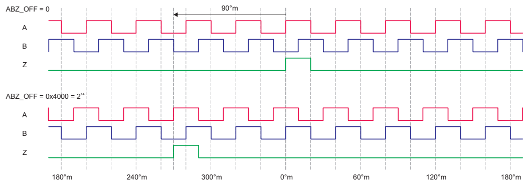
Figure 20: ABZ offset for a system with 9 periods
