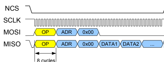
Figure 33: Read Registers
