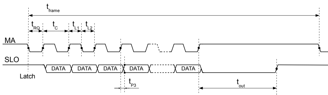
Figure 5: SSI timing
