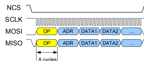
Figure 34: Write Registers
