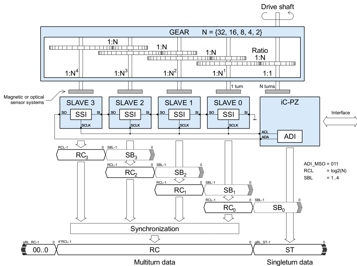
Figure 47: Multi-slave operation – application example with 4 slaves
