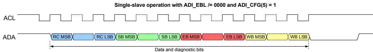
Figure 45: Single-slave operation – exemplary SSI protocol format
