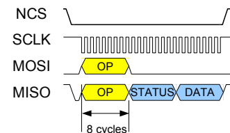
Figure 40: Get Transaction Info
