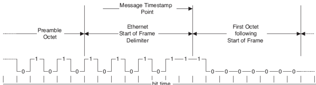
Figure 7-21. Timestamp Point
