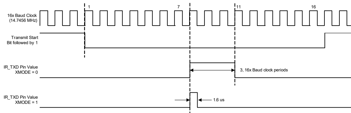
Figure 59: XMODE Example
