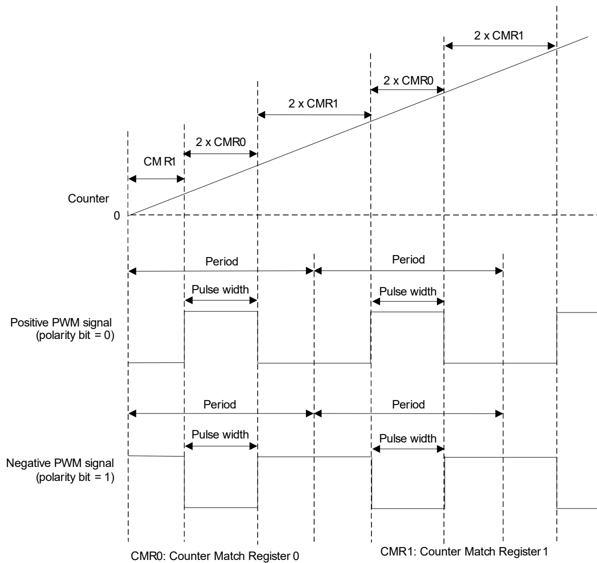
Figure 51: PWM Center-Aligned
