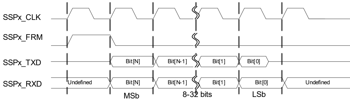
Figure 86: TI SSP with SSP_SSCR1[TTE] = 1 and SSP_SSCR1[TTELP] = 1
