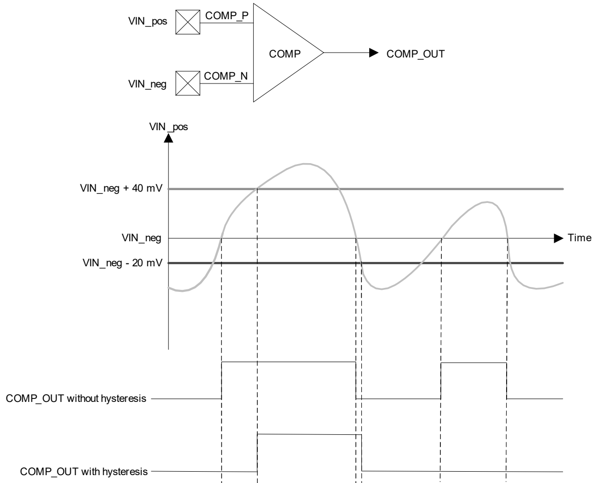
Figure 109: Comparator Hysteresis
