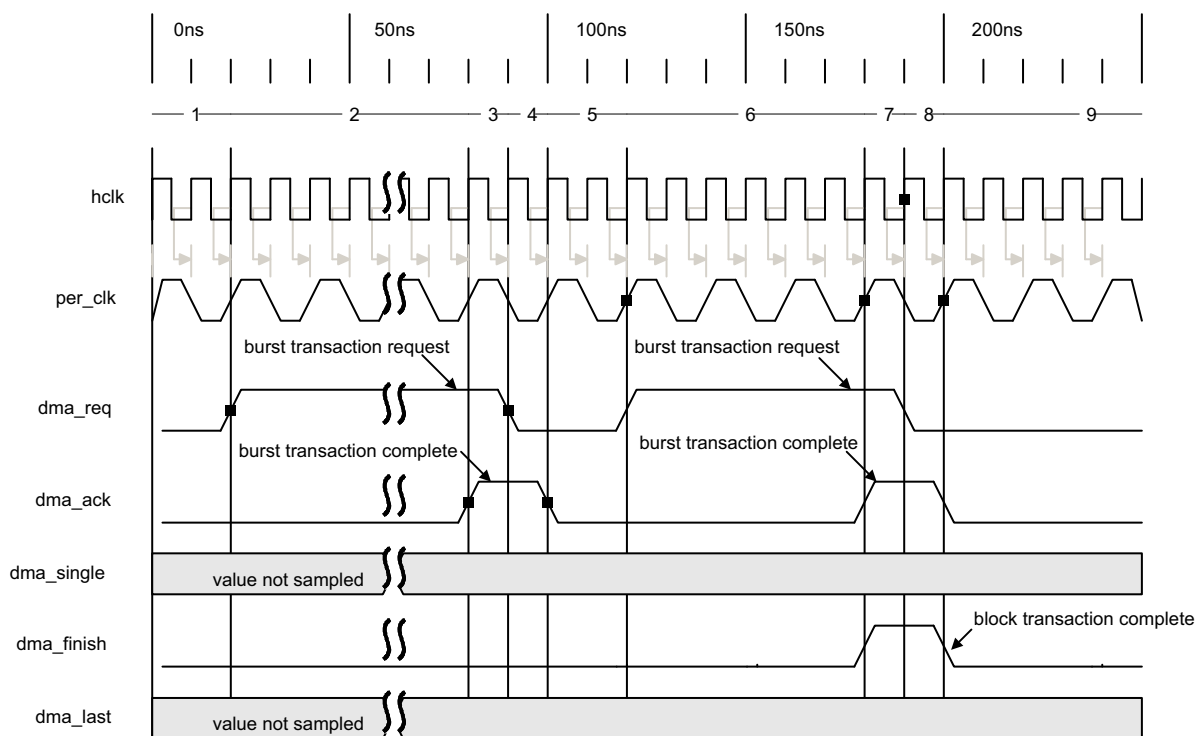
Figure 37: Back-to-Back Burst Transaction – hclk=2 \times per\_clk
