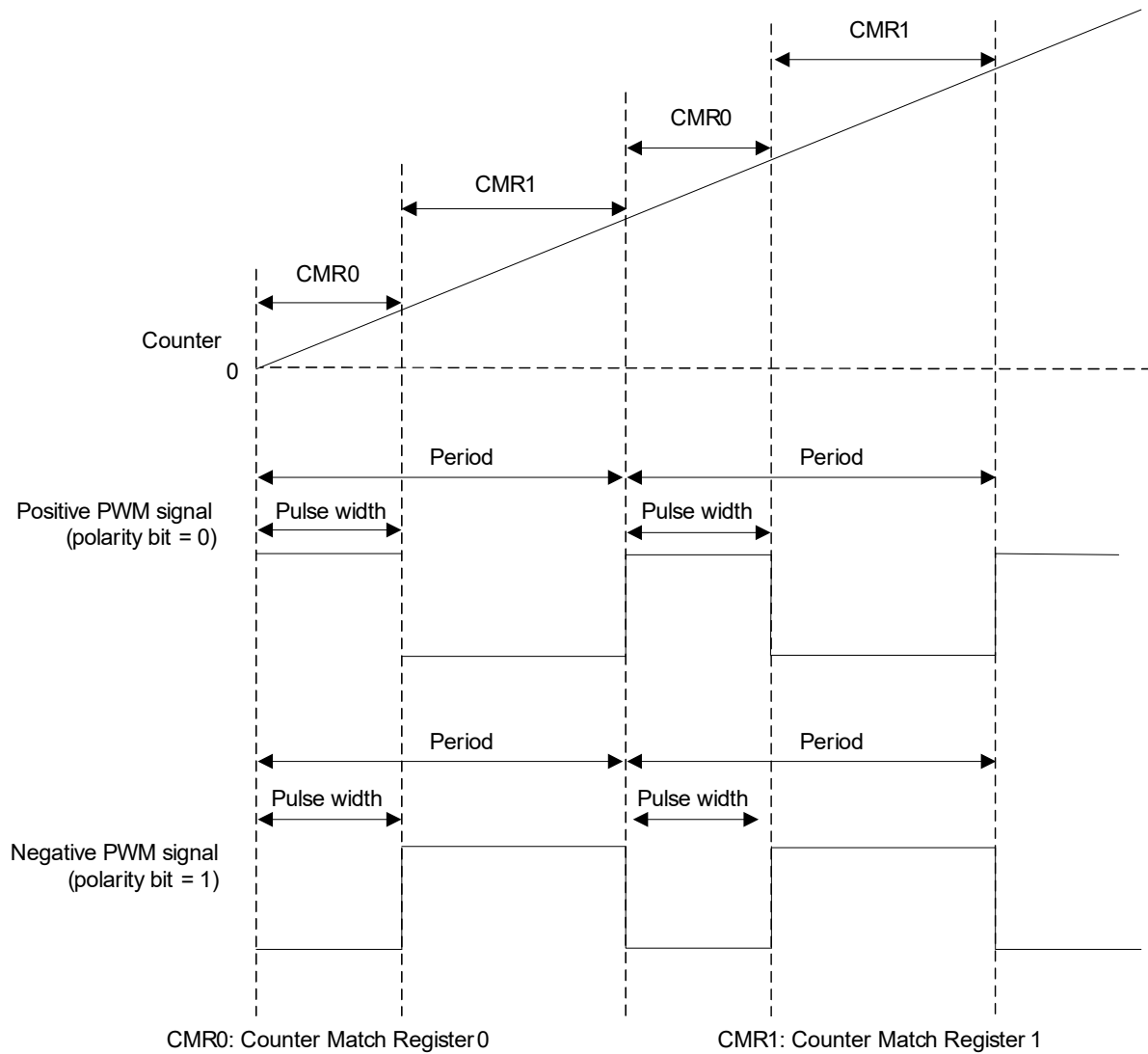
Figure 50: PWM Edge-Aligned
