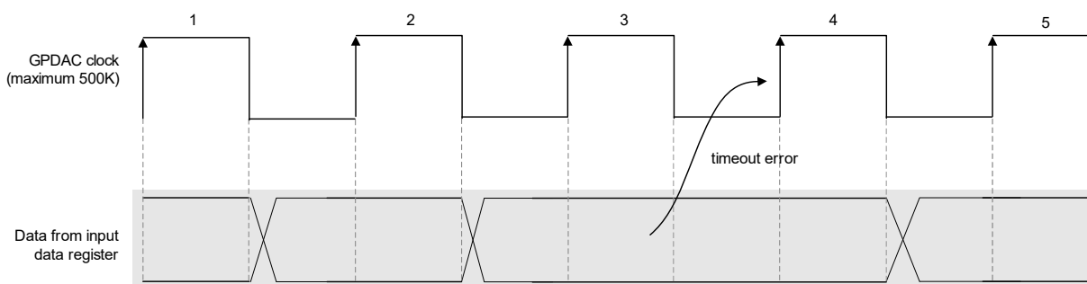
Figure 105: Synchronous Mode
