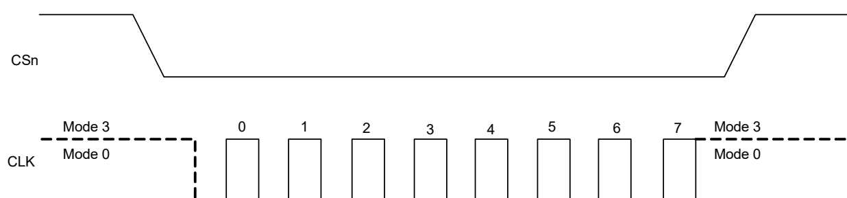
Figure 30: Flash Boot Mode, Timing
