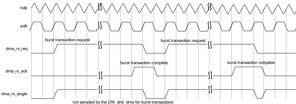
Figure 75: Burst Transaction, hclk = 2 \cdot pclk
