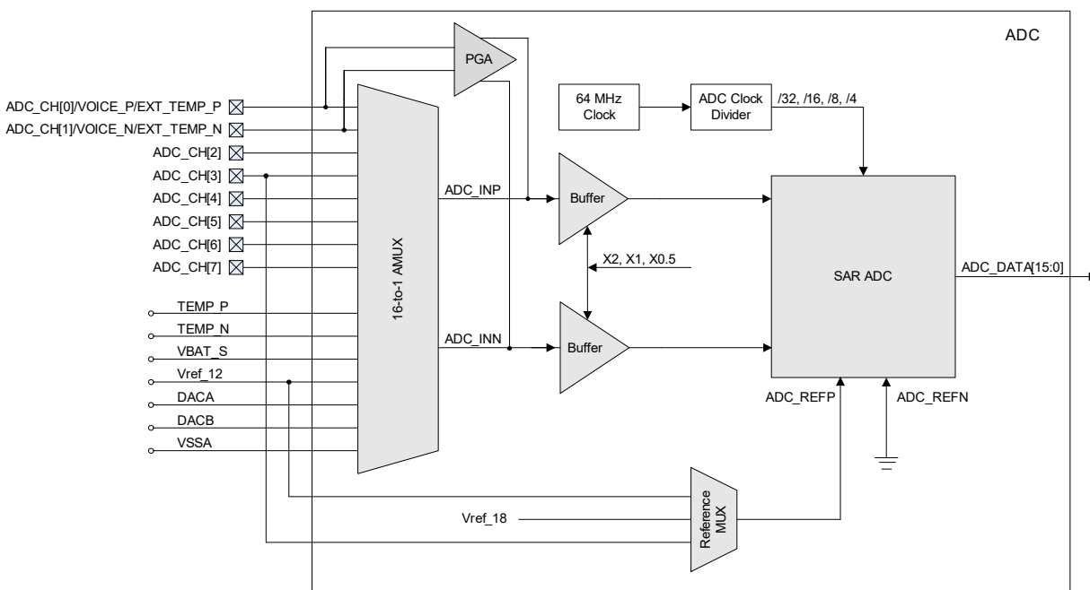
Figure 103:ADC Block Diagram
