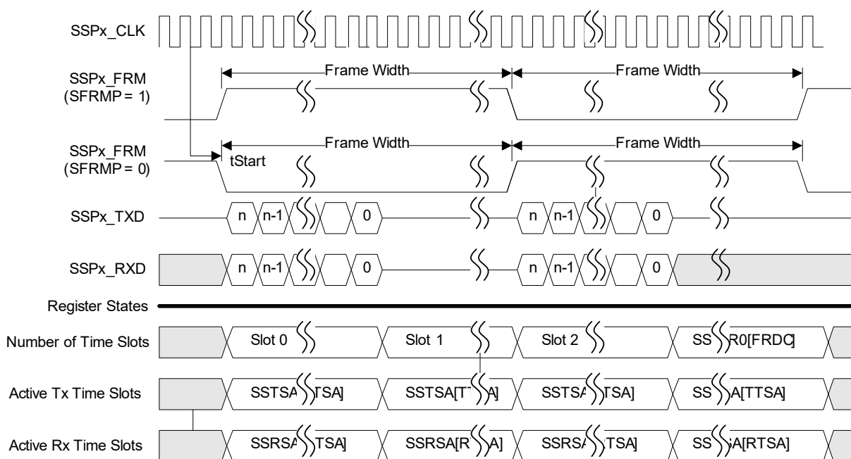
Figure 91: Network Mode and PSP Frame Format
