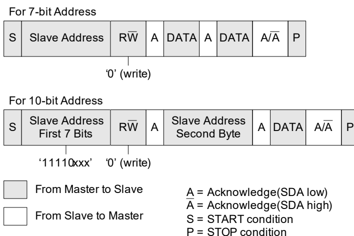
Figure 70: Master-Transmitter Protocol
