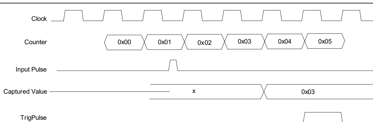
Figure 47: Input Capture Timing
