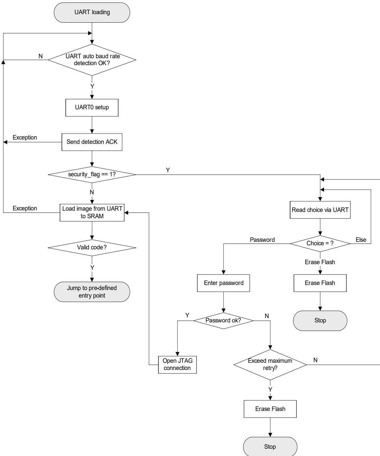
Figure 20: Boot ROM Flow, UART Loading
