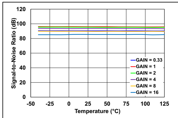
FIGURE 2-31: SNR vs. Temperature, Internal V_{REF} .
