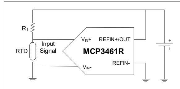
FIGURE 7-3: Wheatstone Bridge Ratiometric Connection.
