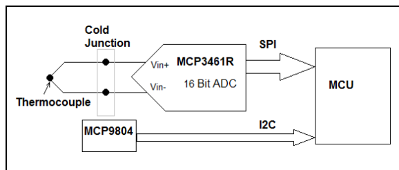
FIGURE 7-2: Thermocouple Connection to MCP3461R.
