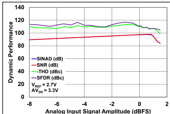
FIGURE 2-34: Dynamic Performance vs. Input Signal Amplitude.
