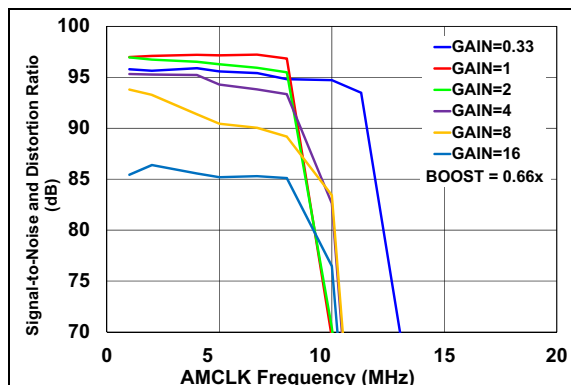
FIGURE 2-36: SINAD vs. AMCLK (Boost = 0.66x , External V_{REF} ).
