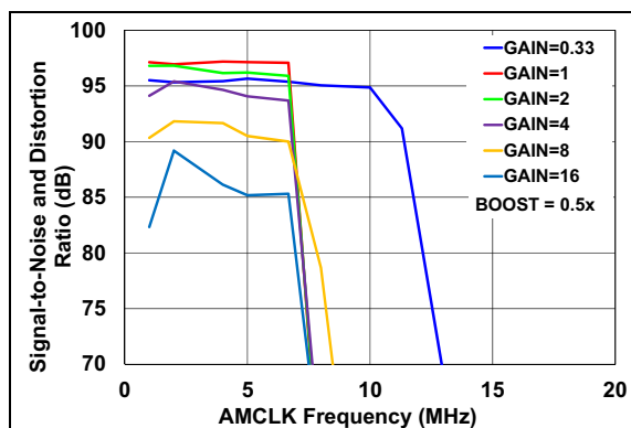
FIGURE 2-35: SINAD vs. AMCLK (Boost = 0.5x , External V_{REF} ).
