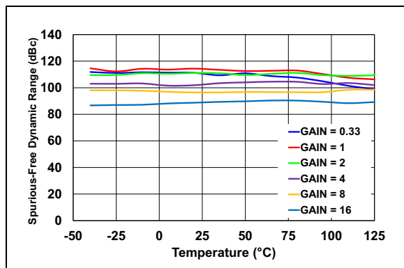
FIGURE 2-33: SFDR vs. Temperature, Internal V_{REF} .
