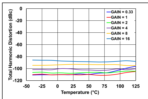
FIGURE 2-32: THD vs. Temperature, Internal V_{REF} .
