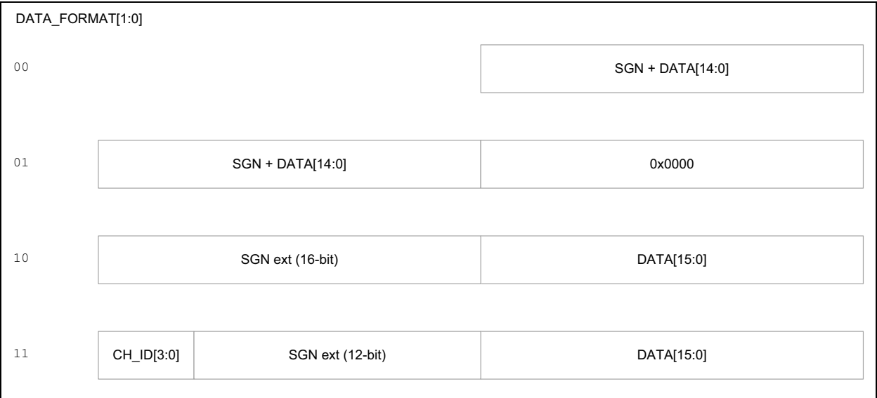
FIGURE 5-8: ADC Output Format Selection.
