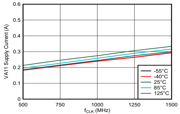
Figure 5-173. VA11 Supply Current vs Clock Rate
