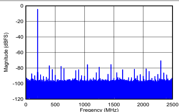
Figure 7-5. 200MHz, Sine-Wave Frequency Domain (FFT) for 5GSPS, Single-Channel Oscilloscope
