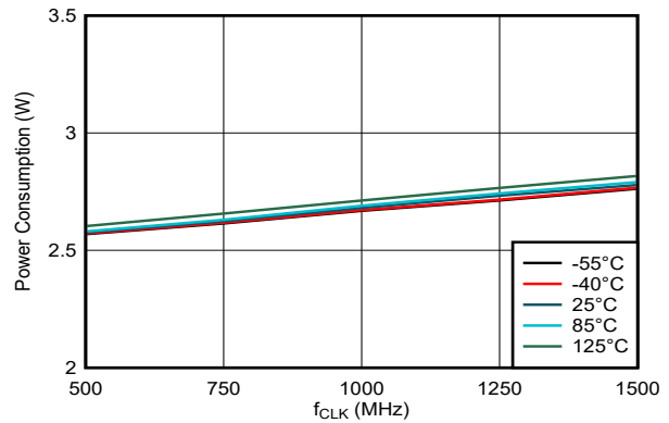
Figure 5-179. Power Consumption vs Clock Rate
