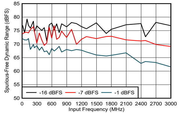
Figure 5-105. SFDR vs Input Frequency
