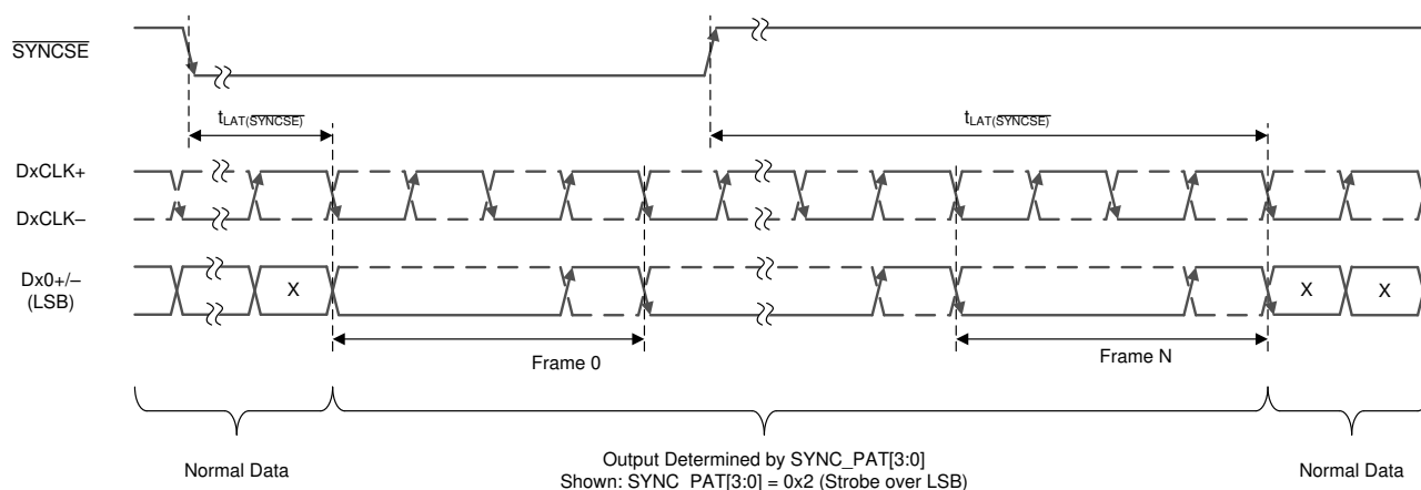
Figure 5-8. SYNCSE Timing Diagram
