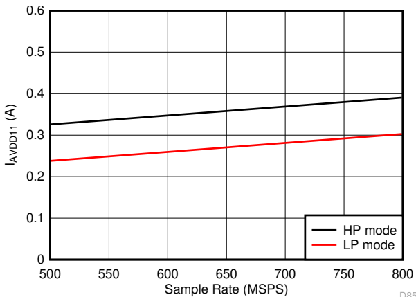
Figure 5-93. Dual Channel, I_{VA11} vs F_S
