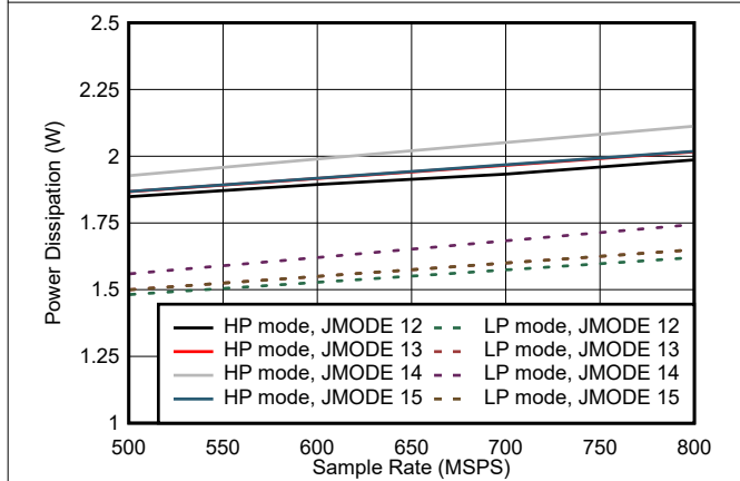
Figure 5-77. Quad Channel, Power Dissipation vs F_S for JMODES 12 - 15
