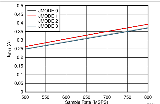
Figure 5-80. Quad Channel, I_{VD11} vs F_S for JMODES 0 - 3 Independent of Power Mode
