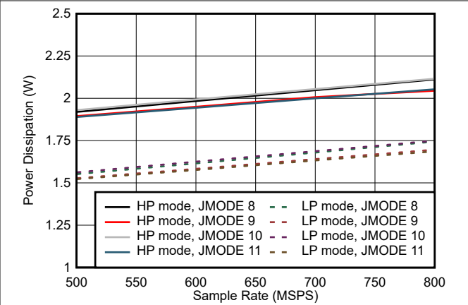
Figure 5-76. Quad Channel, Power Dissipation vs F_S for JMODES 8 - 11
