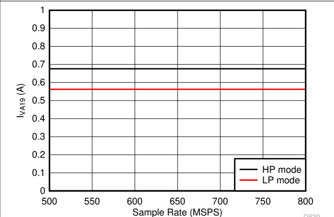
Figure 5-78. Quad Channel, I_{VA19} vs F_S Independent of JMODE
