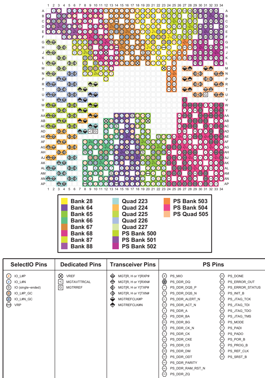
Figure 4-41: FFVC1156 Package—I/O Bank Diagram
