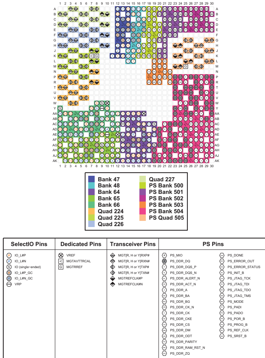
Figure 4-33: FBVB900 Package—XCZU7CG and XCZU7EG I/O Bank Diagram
