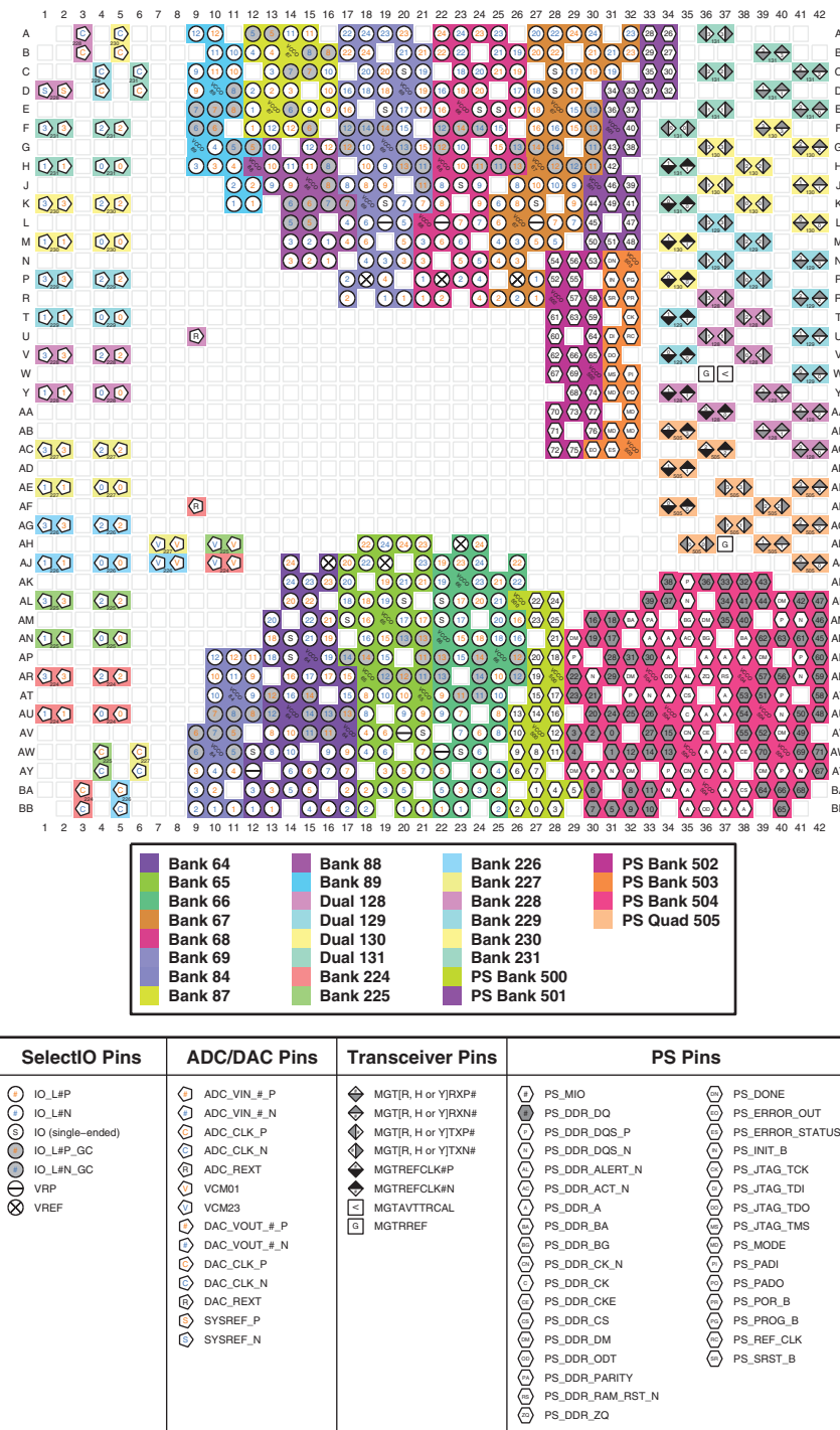
Figure 4-97: FFVF1760, FSVF1760, FSRF1760 Packages—XCZU49DR, XQZU49DR I/O Bank Diagram
