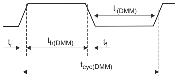
Figure 7-22. DMMCLK Timing
