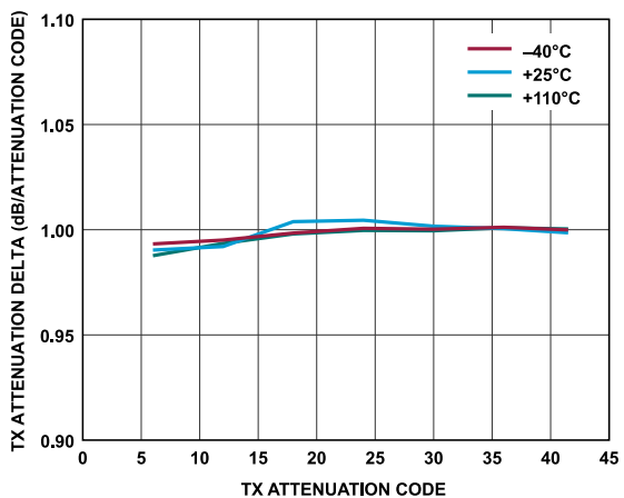
Figure 44. Transmitter Attenuation Delta vs. Transmitter Attenuation Code, Baseband Frequency = 18 MHz, Backoff = 0.2 dBFS
