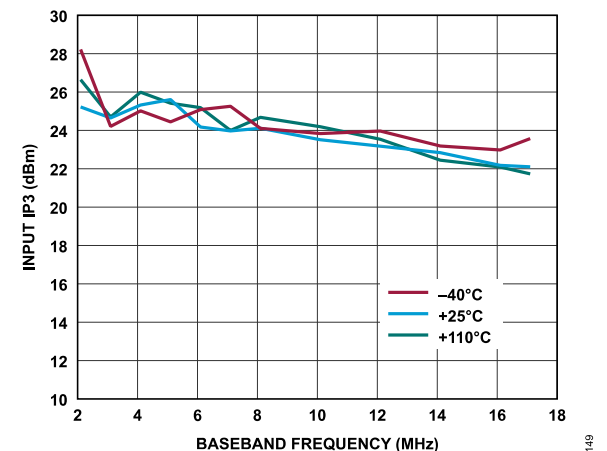
Figure 41. Receiver Input IP3 vs. Baseband Frequency, ADC = Low Power, f_1 = Baseband Frequency, f_2 = Baseband Frequency + 1 MHz, Gain Index = 255
