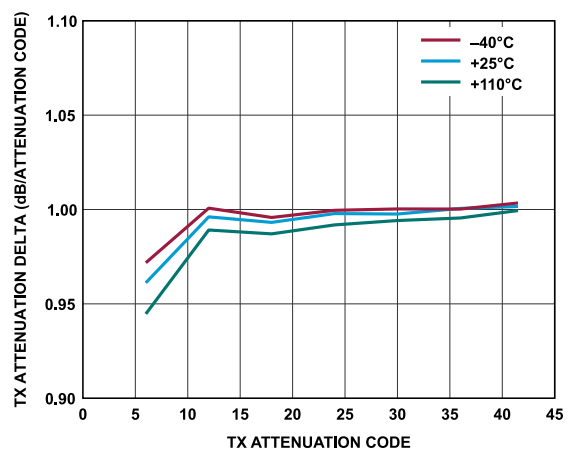
Figure 246. Transmitter Attenuation Delta vs. Transmitter Attenuation Code, Baseband Frequency = 2.1 kHz, Backoff = 0.2 dBFS
