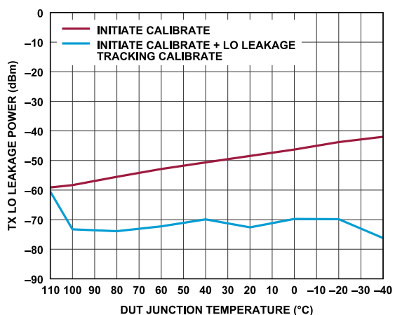
Figure 28. Transmitter LO Leakage Power vs. DUT Junction Temperature (High to Low), Baseband Frequency = 4 MHz, Backoff = 0.5 dBFS, Attenuation Code = 0
