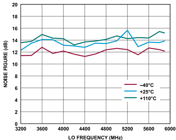
Figure 106. Receiver Noise Figure vs. LO Frequency, Baseband Frequency = 5.6 MHz, ADC = Low Power
