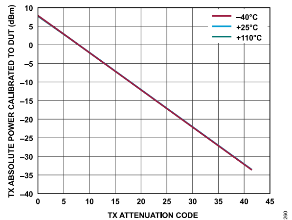
Figure 118. Transmitter Absolute Power Calibrated to DUT vs. Transmitter Attenuation Code, Baseband Frequency = 18 MHz, Backoff = 0.2 dBFS
