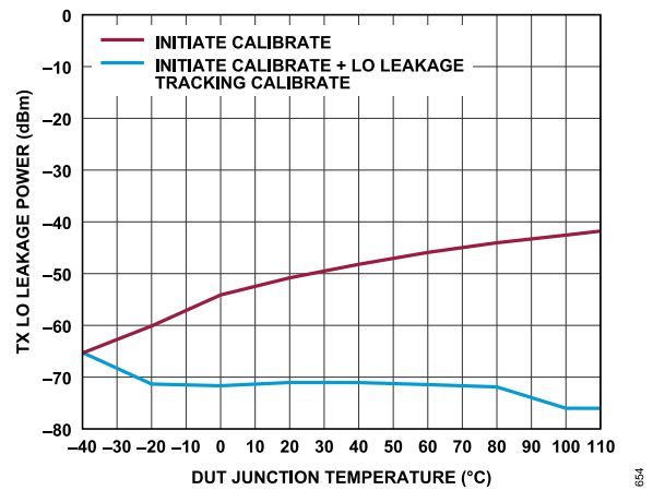
Figure 75. Transmitter LO Leakage Power vs. DUT Junction Temperature (Low to High), Baseband Frequency = 4 MHz, Backoff = 0.5 dBFS, Attenuation Code = 0
