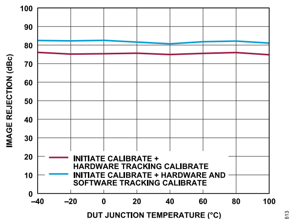
Figure 82. Receiver Image Rejection vs. DUT Junction Temperature (Low to High), Tone 1 Baseband Frequency = -5.1 MHz, Tone 2 Baseband Frequency = 13.9 MHz, ADC = Low Power, P_{OUT} = -11.1 dBFS
