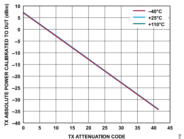
Figure 19. Transmitter Absolute Power Calibrated to DUT vs. Transmitter Attenuation Code, Baseband Frequency = 18 MHz, Backoff = 0.2 dBFS
