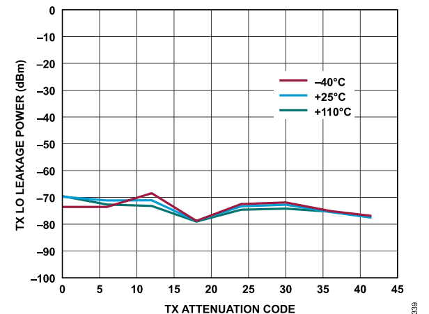
Figure 170. Transmitter LO Leakage Power vs. Transmitter Attenuation Code, Baseband Frequency = 2.1 kHz, Backoff = 6 dBFS, Initialization Calibration Only
