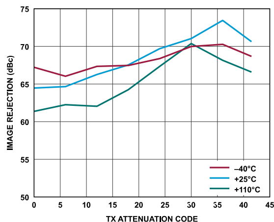
Figure 199. Transmitter Image Rejection vs. Transmitter Attenuation Code, Baseband Frequency = 2.1 kHz, Backoff = 0.2 dBFS, Initialization Calibration Only
