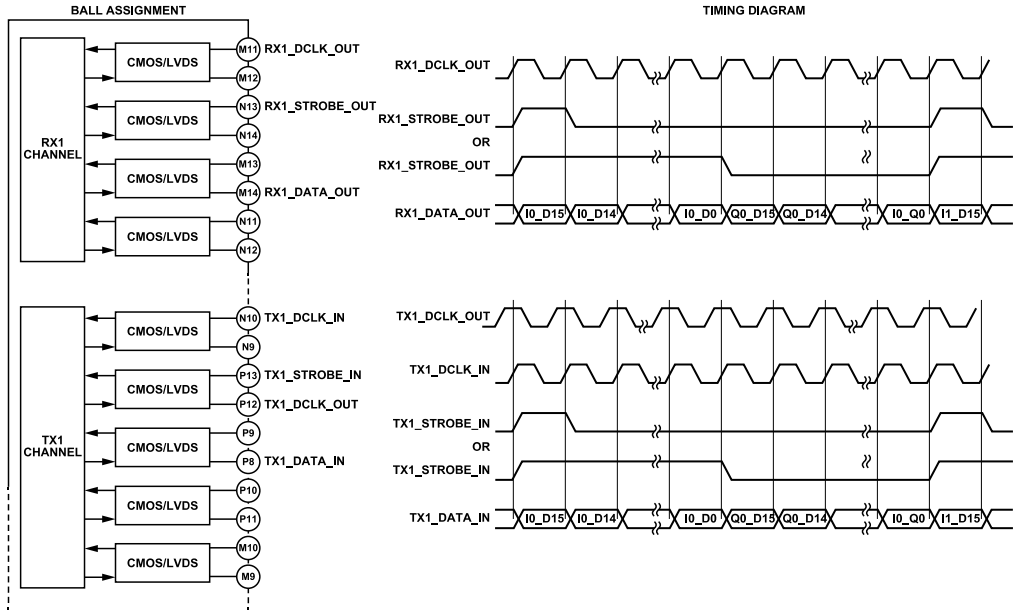
Figure 261. CSSI in 1-Lane Data Mode
