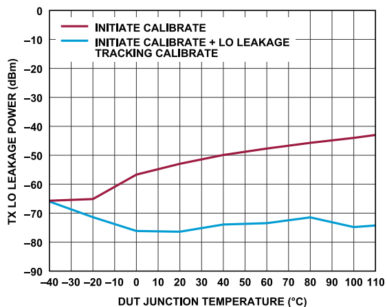
Figure 27. Transmitter LO Leakage Power vs. DUT Junction Temperature (Low to High), Baseband Frequency = 4 MHz, Backoff = 0.5 dBFS, Attenuation Code = 0
