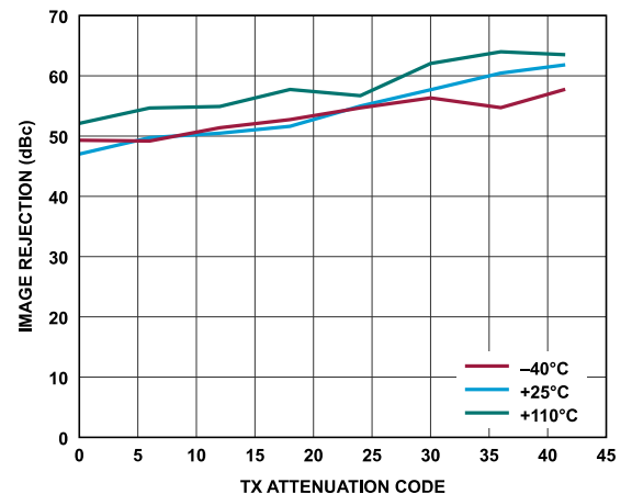
Figure 247. Transmitter Image Rejection vs. Transmitter Attenuation Code, Baseband Frequency = 2.1 kHz, Backoff = 0.2 dBFS, Initialization Calibration Only
