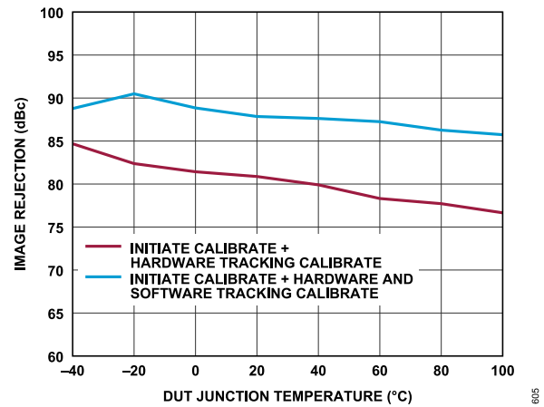
Figure 34. Receiver Image Rejection vs. DUT Junction Temperature (Low to High), Tone 1 Baseband Frequency = -5.1 MHz, Tone 2 Baseband Frequency = 13.9 MHz, ADC = Low Power, P_{OUT} = -11.1 dBFS
