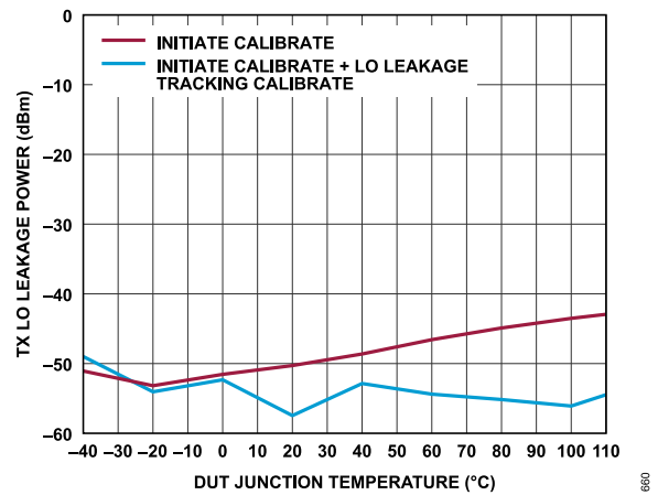
Figure 150. Transmitter LO Leakage Power vs. DUT Junction Temperature (Low to High), Baseband Frequency = 4 MHz, Backoff = 0.5 dBFS, Attenuation Code = 0
