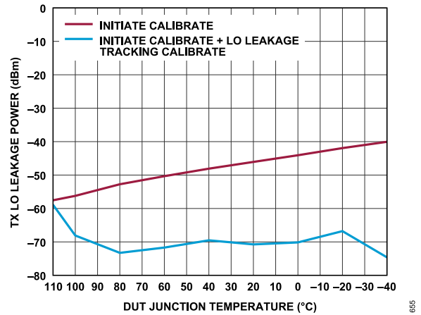
Figure 76. Transmitter LO Leakage Power vs. DUT Junction Temperature (High to Low), Baseband Frequency = 4 MHz, Backoff = 0.5 dBFS, Attenuation Code = 0
