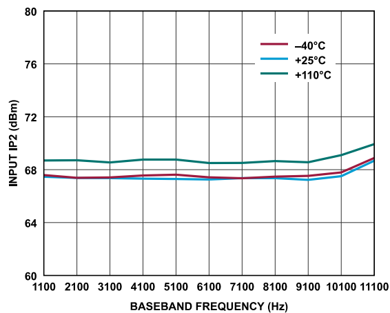
Figure 244. Receiver Input IP2 vs. Baseband Frequency, ADC = Low Power, f_1 = Baseband Frequency + 1 MHz, f_2 = Baseband Frequency + 2 MHz, Gain Index = 255, First-Order TIA with f_{3dB} = 4 MHz, P_{OUT} = -6.6 dBFS
