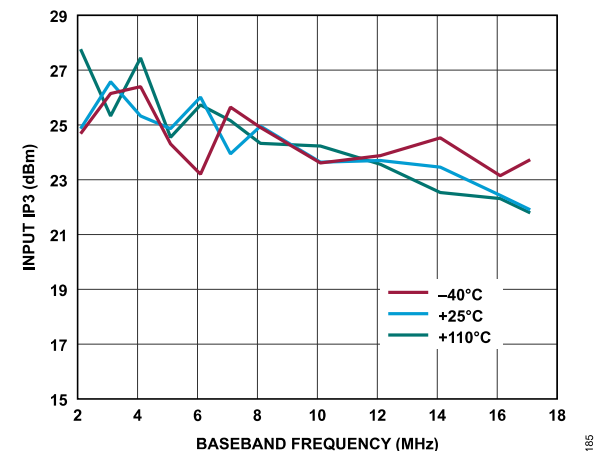
Figure 65. Receiver Input IP3 vs. Baseband Frequency, ADC = Low Power, f_1 = Baseband Frequency, f_2 = Baseband Frequency + 1 MHz, Gain Index = 255
