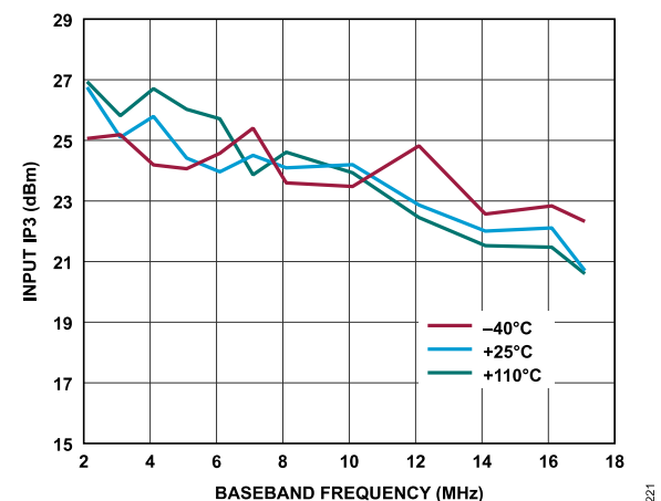
Figure 89. Receiver Input IP3 vs. Baseband Frequency, ADC = Low Power, f_1 = Baseband Frequency, f_2 = Baseband Frequency + 1 MHz, Gain Index = 255
