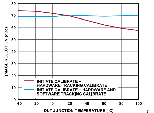
Figure 108. Receiver Image Rejection vs. DUT Junction Temperature (Low to High), Tone 1 Baseband Frequency = -5.1 MHz, Tone 2 Baseband Frequency = 13.9 MHz, ADC = Low Power, P_{OUT} = -11.1 dBFS
