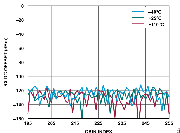
Figure 162. Receiver DC Offset vs. Gain Index, Baseband Frequency = 2.1 kHz, ADC = Low Power
