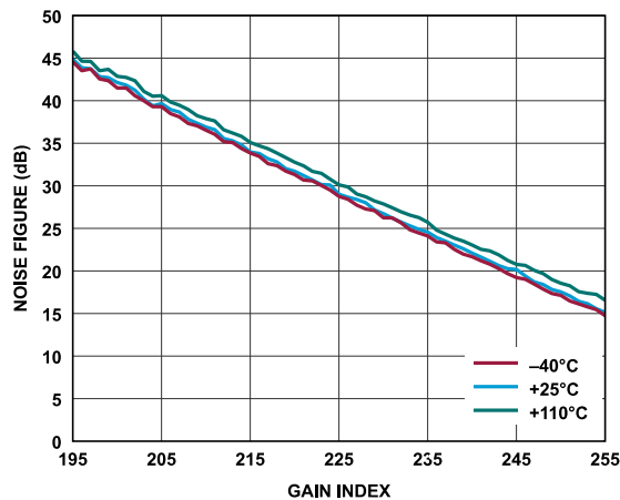
Figure 205. Receiver Noise Figure vs. Gain Index, Baseband Frequency = 2.1 kHz, ADC = Low Power
