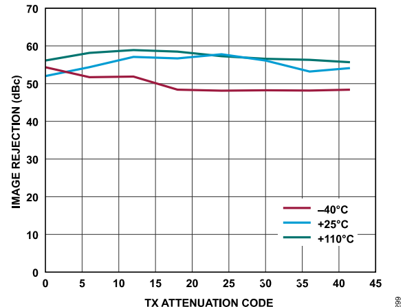
Figure 146. Transmitter Image Rejection vs. Transmitter Attenuation Code, Baseband Frequency = 18 MHz, Backoff = 0.2 dBFS, Initialization Calibration Only
