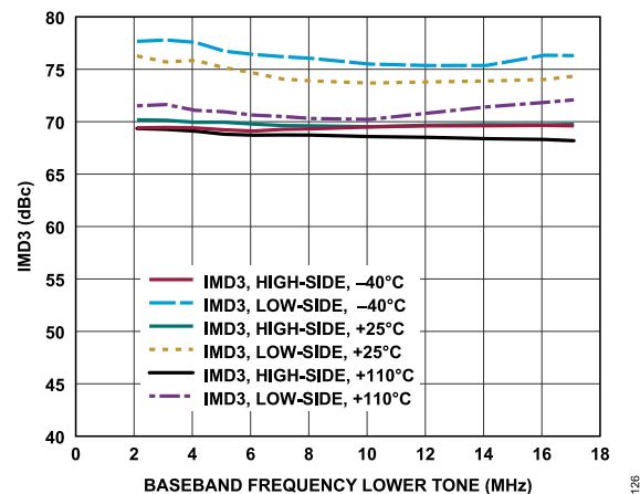
Figure 30. Transmitter Third-Order Intermodulation Distortion (IMD3) vs. Baseband Frequency, Transmitter Attenuation Code = 0, f_1 = Baseband Frequency, f_2 = Baseband Frequency + 1 MHz
