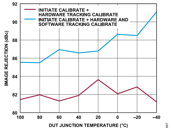
Figure 35. Receiver Image Rejection vs. DUT Junction Temperature (High to Low), Tone 1 Baseband Frequency = -5.1 MHz, Tone 2 Baseband Frequency = 13.9 MHz, ADC = Low Power, P_{OUT} = -11.1 dBFS
