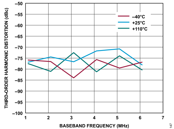
Figure 39. Receiver Third-Order Harmonic Distortion vs. Baseband Frequency, Gain Index = 255, ADC = Low Power
