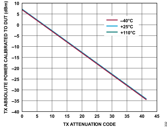
Figure 165. Transmitter Absolute Power Calibrated to DUT vs. Transmitter Attenuation Code, Baseband Frequency = 2.1 kHz, Backoff = 0.2 dBFS
