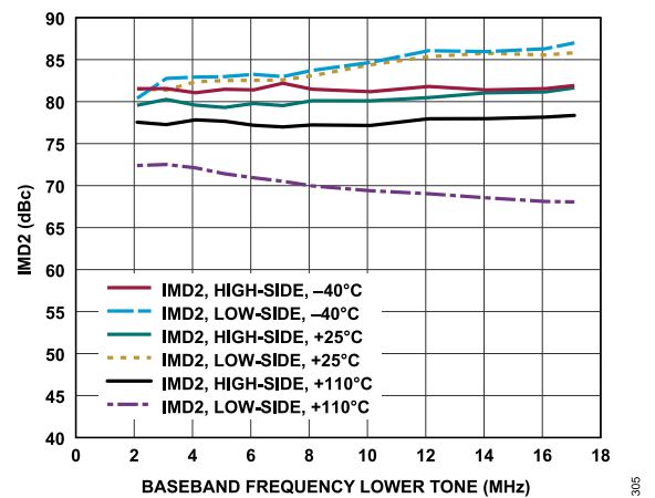
Figure 152. Transmitter IMD2 vs. Baseband Frequency, Transmitter Attenuation Code = 0, f_1 = Baseband Frequency, f_2 = Baseband Frequency + 1 MHz
