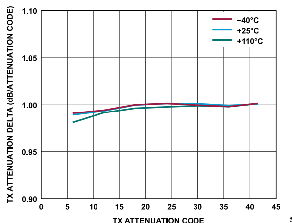
Figure 198. Transmitter Attenuation Delta vs. Transmitter Attenuation Code, Baseband Frequency = 2.1 kHz, Backoff = 0.2 dBFS
