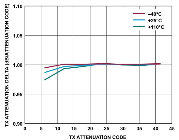
Figure 119. Transmitter Attenuation Delta vs. Transmitter Attenuation Code, Baseband Frequency = 18 MHz, Backoff = 0.2 dBFS
