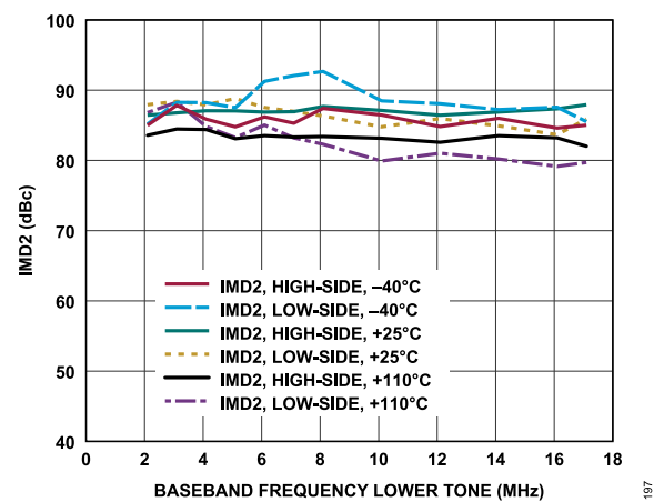
Figure 77. Transmitter IMD2 vs. Baseband Frequency, Transmitter Attenuation Code = 0, f_1 = Baseband Frequency, f_2 = Baseband Frequency + 1 MHz
