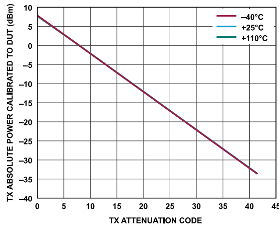
Figure 168. Transmitter Absolute Power Calibrated to DUT vs. Transmitter Attenuation Code, Baseband Frequency = 18 MHz, Backoff = 0.2 dBFS
