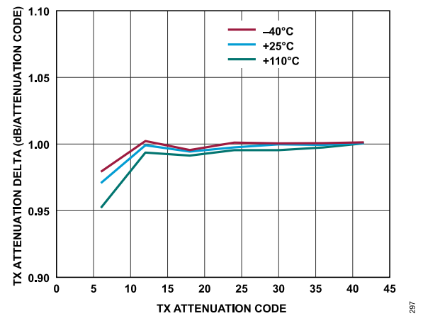
Figure 202. Transmitter Attenuation Delta vs. Transmitter Attenuation Code, Baseband Frequency = 18 MHz, Backoff = 0.2 dBFS
