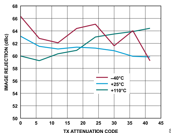
Figure 233. Transmitter Image Rejection vs. Transmitter Attenuation Code, Baseband Frequency = 2.1 kHz, Backoff = 0.2 dBFS
