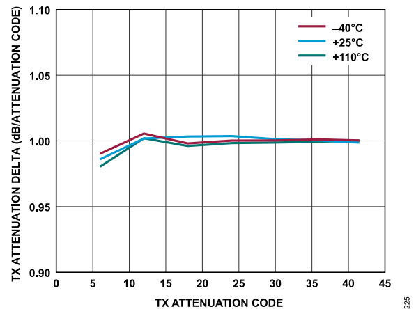
Figure 130. Transmitter Attenuation Delta vs. Transmitter Attenuation Code, Baseband Frequency = 18 MHz, Backoff = 0.2 dBFS
