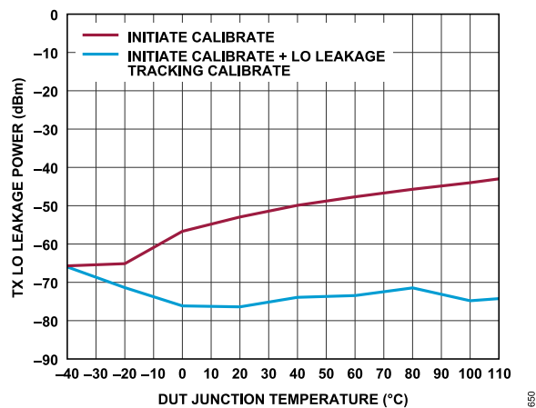
Figure 38. Transmitter LO Leakage Power vs. DUT Junction Temperature (Low to High), Baseband Frequency = 4 MHz, Backoff = 0.5 dBFS, Attenuation Code = 0
