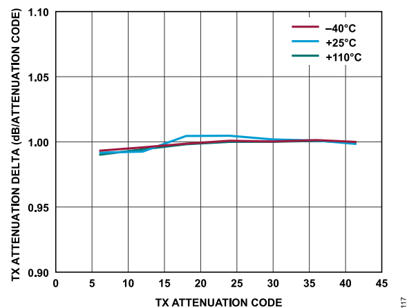
Figure 31. Transmitter Attenuation Delta vs. Transmitter Attenuation Code, Baseband Frequency = 18 MHz, Backoff = 0.2 dBFS
