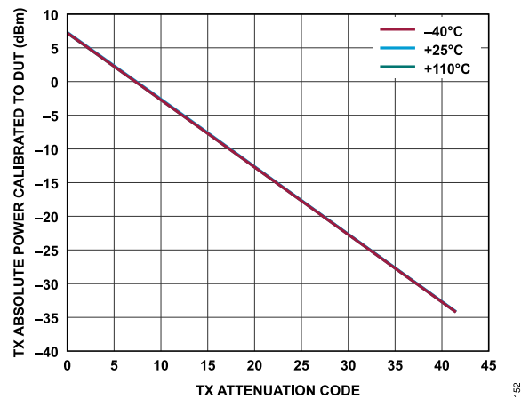
Figure 63. Transmitter Absolute Power Calibrated to DUT vs. Transmitter Attenuation Code, Baseband Frequency = 18 MHz, Backoff = 0.2 dBFS
