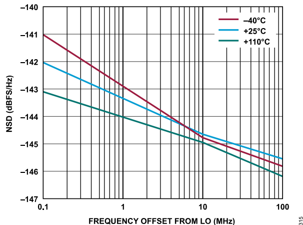
Figure 213. Transmitter NSD vs. Frequency Offset from LO, Baseband Frequency = 5.6 MHz, Transmitter Channel = Channel 1
