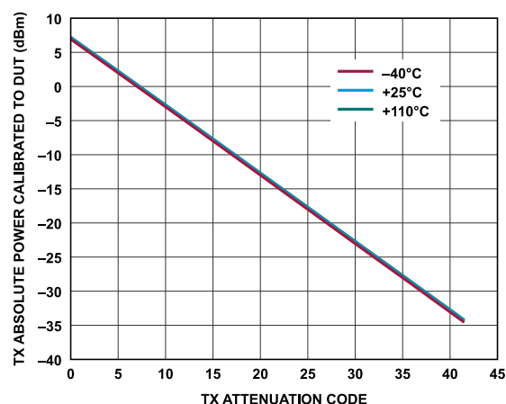
Figure 231. Transmitter Absolute Power Calibrate to DUT vs. Transmitter Attenuation Code, Baseband Frequency = 2.1 kHz, Backoff = 0.2 dBFS
