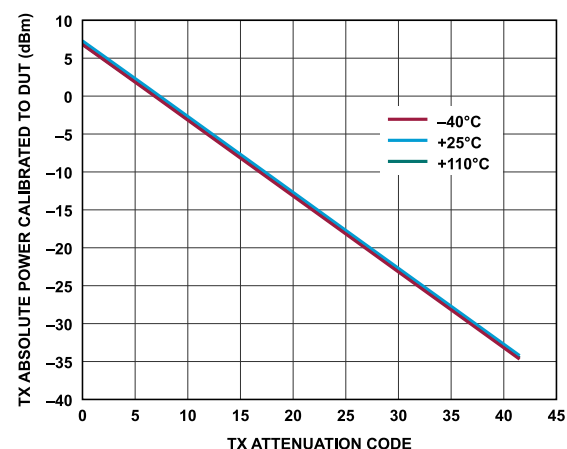
Figure 254. Transmitter Absolute Power Calibrated to DUT vs. Transmitter Attenuation Code, Baseband Frequency = 2.1 kHz, Backoff = 0.2 dBFS
