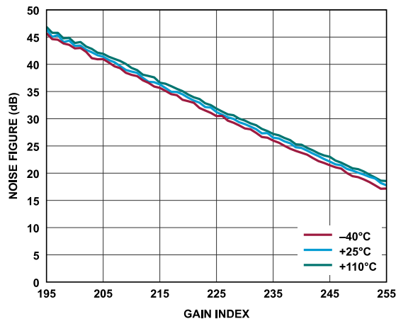
Figure 333. Receiver Noise Figure vs. Gain Index, Baseband Frequency = 2.1 kHz, ADC = Low Power
