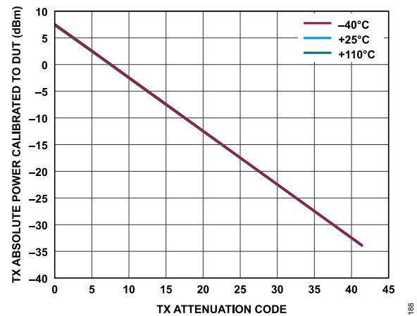
Figure 96. Transmitter Absolute Power Calibrated to DUT vs. Transmitter Attenuation Code, Baseband Frequency = 18 MHz, Backoff = 0.2 dBFS
