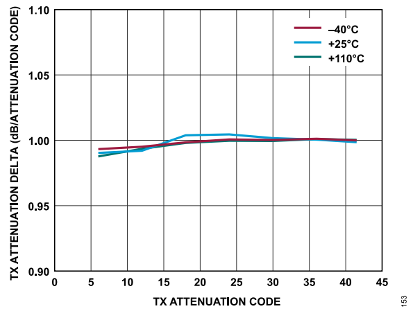
Figure 64. Transmitter Attenuation Delta vs. Transmitter Attenuation Code, Baseband Frequency = 18 MHz, Backoff = 0.2 dBFS
