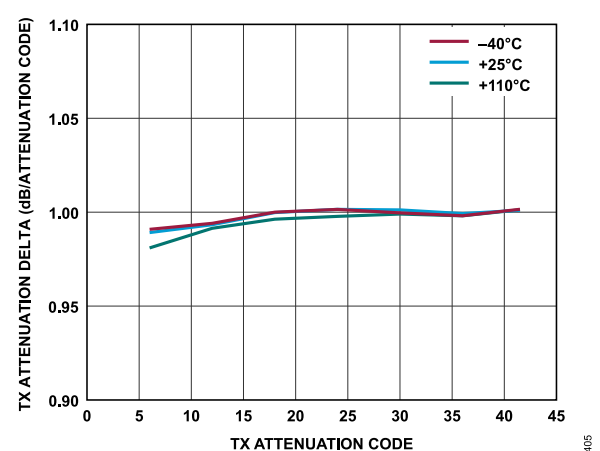
Figure 278. Transmitter Attenuation Delta vs. Transmitter Attenuation Code, Baseband Frequency = 2.1 kHz, Backoff = 0.2 dBFS
