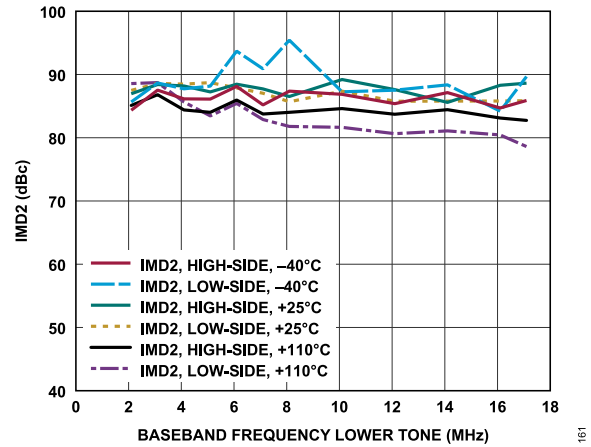
Figure 73. Transmitter IMD2 vs. Baseband Frequency, Transmitter Attenuation Code = 0, f_1 = Baseband Frequency, f_2 = Baseband Frequency + 1 MHz
