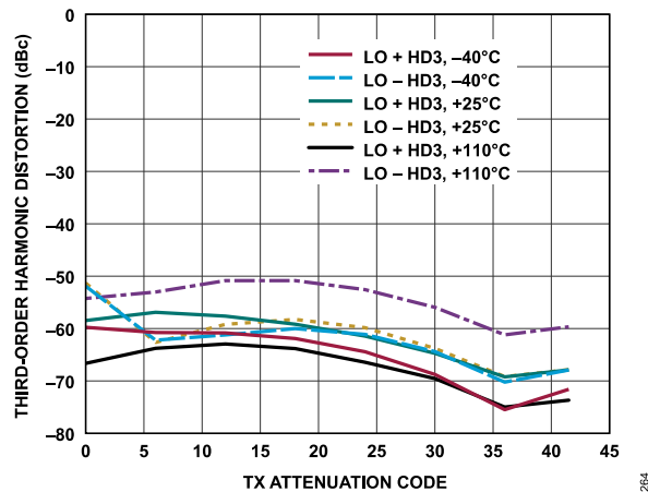
Figure 173. Transmitter Third-Order Harmonic Distortion vs. Transmitter Attenuation Code, Baseband Frequency = 18 MHz, Backoff = 0.2 dBFS
