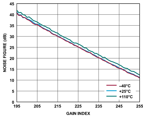
Figure 239. Receiver Noise Figure vs. Gain Index, Baseband Frequency = 2.1 kHz, ADC = High Performance
