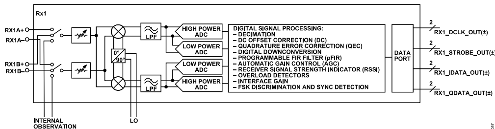
Figure 361. Receiver Architecture
