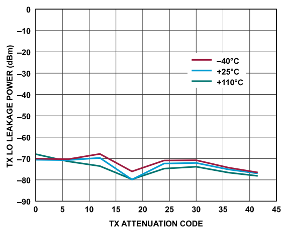
Figure 305. Transmitter LO Leakage Power vs. Transmitter Attenuation Code, Baseband Frequency = 2.1 kHz, Backoff = 6 dBFS, Initialization Calibration Only
