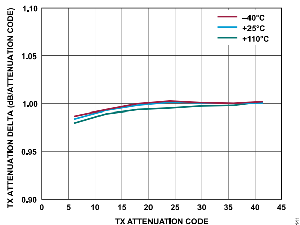
Figure 301. Transmitter Attenuation Delta vs. Transmitter Attenuation Code, Baseband Frequency = 2.1 kHz, Backoff = 0.2 dBFS
