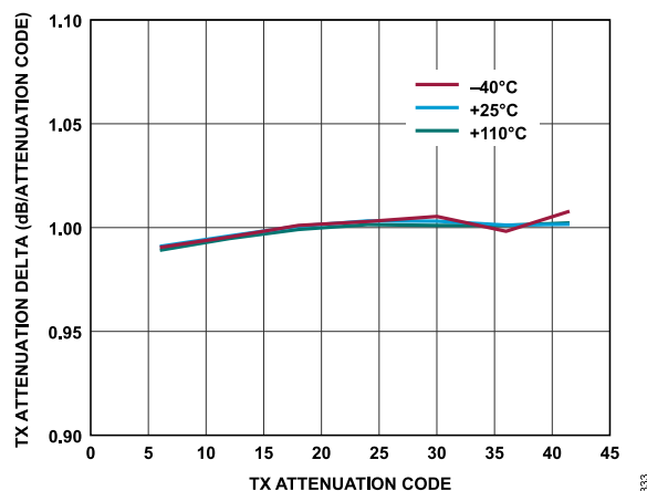
Figure 232. Transmitter Attenuation Delta vs. Transmitter Attenuation Code, Baseband Frequency = 2.1 kHz, Backoff = 0.2 dBFS
