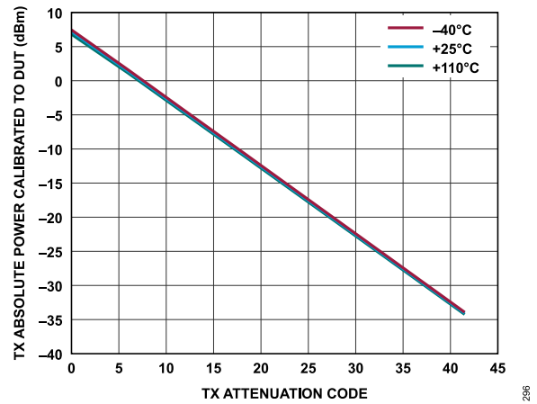
Figure 201. Transmitter Absolute Power Calibrate to DUT vs. Transmitter Attenuation Code, Baseband Frequency = 18 MHz, Backoff = 0.2 dBFS
