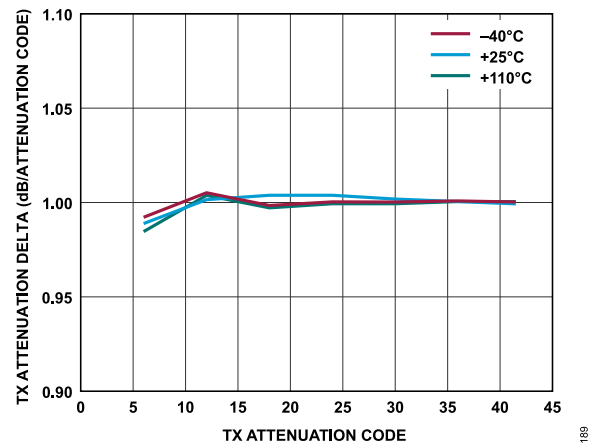
Figure 97. Transmitter Attenuation Delta vs. Transmitter Attenuation Code, Baseband Frequency = 18 MHz, Backoff = 0.2 dBFS
