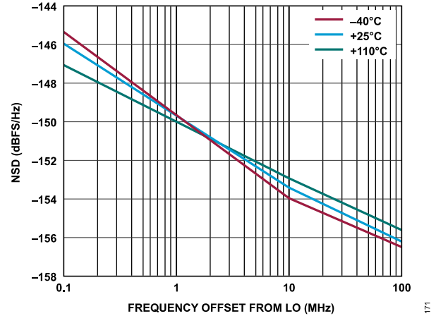
Figure 75. Transmitter NSD vs. Frequency Offset from LO, Baseband Frequency = 5.6 MHz, Transmitter Channel = Channel 1
