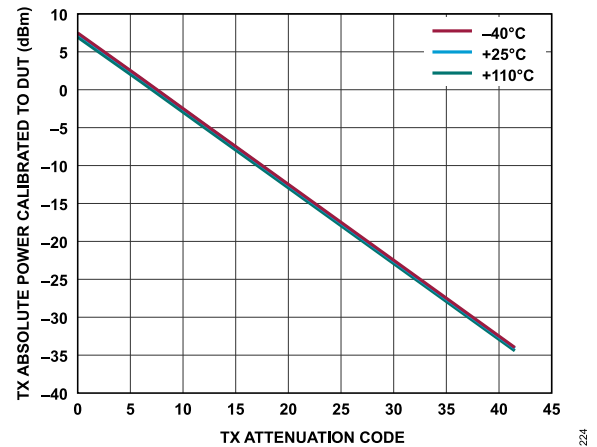
Figure 129. Transmitter Absolute Power Calibrated to DUT vs. Transmitter Attenuation Code, Baseband Frequency = 18 MHz, Backoff = 0.2 dBFS
