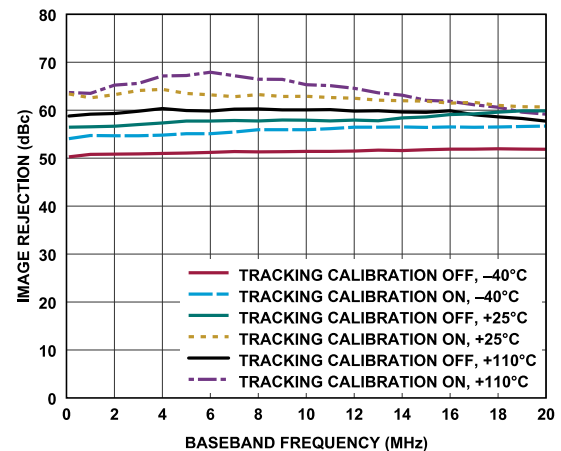
Figure 170. Transmitter Image Rejection vs. Baseband Frequency, Tracking Calibration On vs. Tracking Calibration Off, Transmitter Attenuation Code = 0
