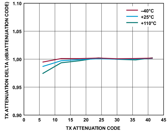
Figure 169. Transmitter Attenuation Delta vs. Transmitter Attenuation Code, Baseband Frequency = 18 MHz, Backoff = 0.2 dBFS
