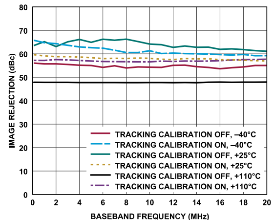
Figure 171. Transmitter Image Rejection vs. Baseband Frequency, Tracking Calibration On vs. Tracking Calibration Off, Transmitter Attenuation Code = 20
