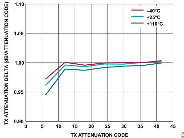
Figure 348. Transmitter Attenuation Delta vs. Transmitter Attenuation Code, Baseband Frequency = 2.1 kHz, Backoff = 0.2 dBFS
