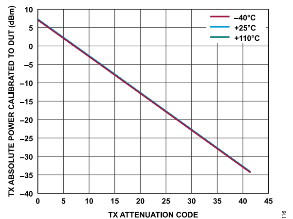
Figure 30. Transmitter Absolute Power Calibrated to DUT vs. Transmitter Attenuation Code, Baseband Frequency = 18 MHz, Backoff = 0.2 dBFS
