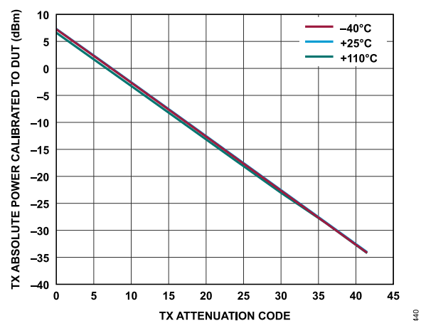
Figure 300. Transmitter Absolute Power Calibrated to DUT vs. Transmitter Attenuation Code, Baseband Frequency = 2.1 kHz, Backoff = 0.2 dBFS
