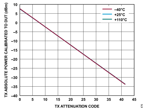
Figure 324. Transmitter Absolute Power Calibrated to DUT vs. Transmitter Attenuation Code, Baseband Frequency = 2.1 kHz, Backoff = 0.2 dBFS
