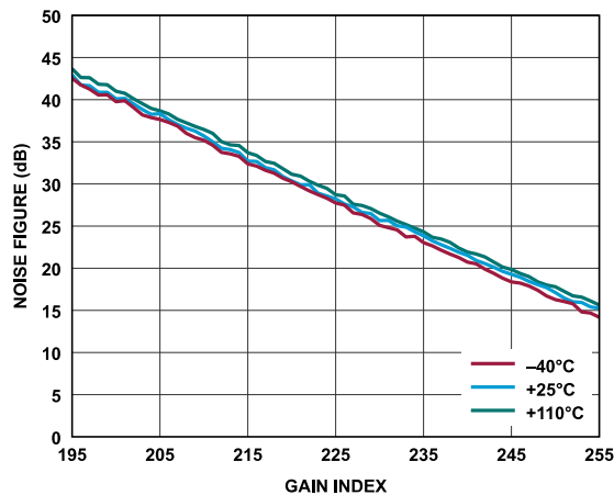
Figure 332. Receiver Noise Figure vs. Gain Index, Baseband Frequency = 2.1 kHz, ADC = High Performance
