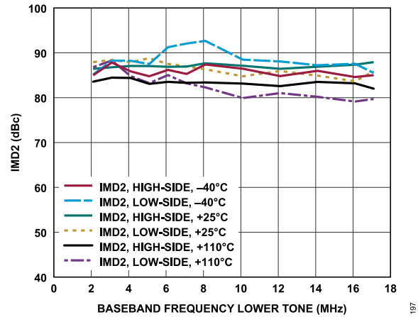
Figure 106. Transmitter IMD2 vs. Baseband Frequency, Transmitter Attenuation Code = 0, f_1 = Baseband Frequency, f_2 = Baseband Frequency + 1 MHz
