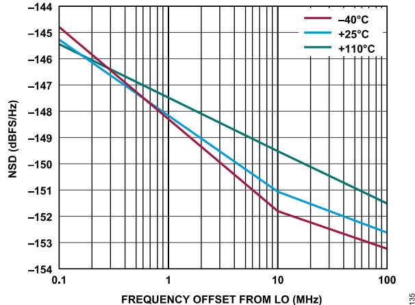
Figure 42. Transmitter NSD vs. Frequency Offset from LO, Baseband Frequency = 5.6 MHz, Transmitter Channel = Channel 1
