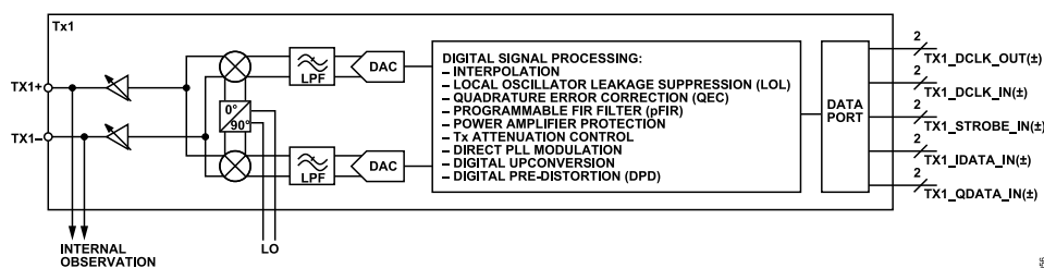
Figure 360. Transmitter Architecture
