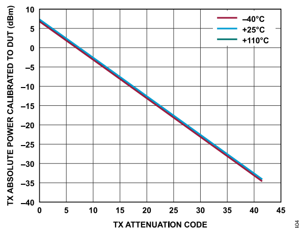
Figure 273. Transmitter Absolute Power Calibrated to DUT vs. Transmitter Attenuation Code, Baseband Frequency = 2.1 kHz, Backoff = 0.2 dBFS
