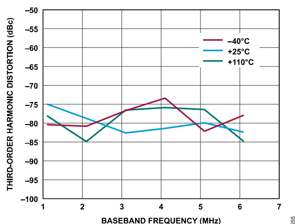
Figure 161. Receiver Third-Order Harmonic Distortion vs. Baseband Frequency, Gain index = 255, ADC = Low Power
