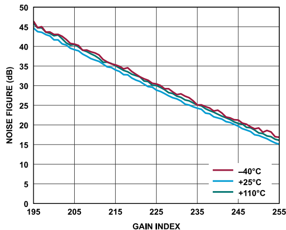
Figure 240. Receiver Noise Figure vs. Gain Index, Baseband Frequency = 2.1 kHz, ADC = Low Power
