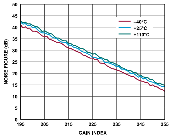
Figure 183. Receiver Noise Figure vs. Gain Index, Baseband Frequency = 5.6 MHz, ADC = Low Power
