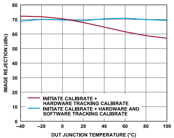
Figure 150. Receiver Image Rejection vs. DUT Junction Temperature (Low to High), Tone 1 Baseband Frequency = -5.1 MHz, Tone 2 Baseband Frequency = 13.9 MHz, ADC = High Performance, P_{OUT} = -11.1 dBFS
