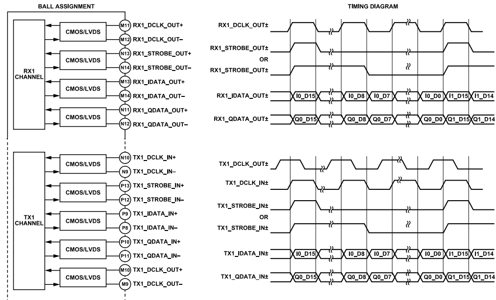
Figure 365. LSSI in 2-Lane Data Mode, DDR
