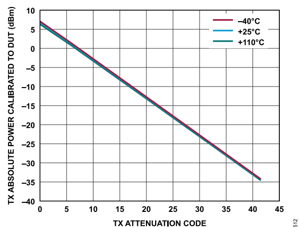
Figure 347. Transmitter Absolute Power Calibrated to DUT vs. Transmitter Attenuation Code, Baseband Frequency = 2.1 kHz, Backoff = 0.2 dBFS
