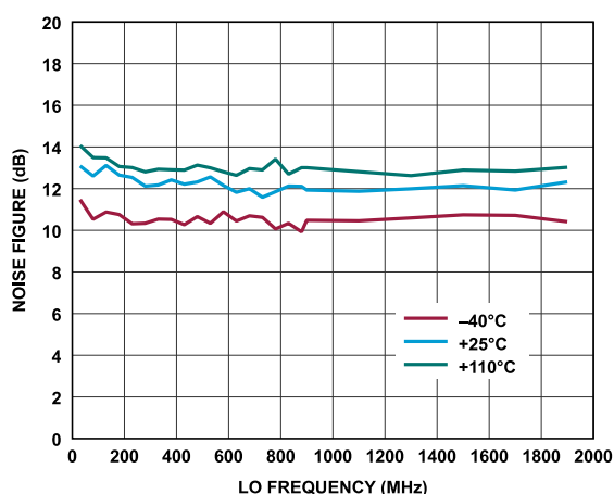
Figure 9. Receiver Noise Figure vs. LO Frequency, Baseband Frequency = 5.6 MHz, ADC = Low Power
