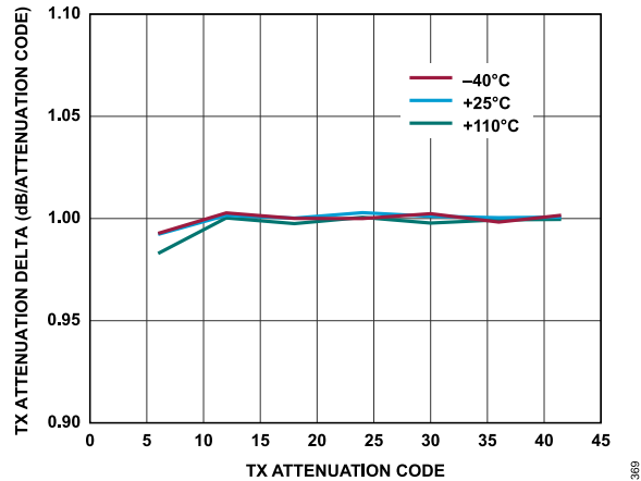
Figure 255. Transmitter Attenuation Delta vs. Transmitter Attenuation Code, Baseband Frequency = 2.1 kHz, Backoff = 0.2 dBFS
