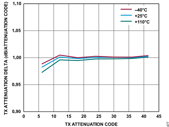
Figure 325. Transmitter Attenuation Delta vs. Transmitter Attenuation Code, Baseband Frequency = 2.1 kHz, Backoff = 0.2 dBFS
