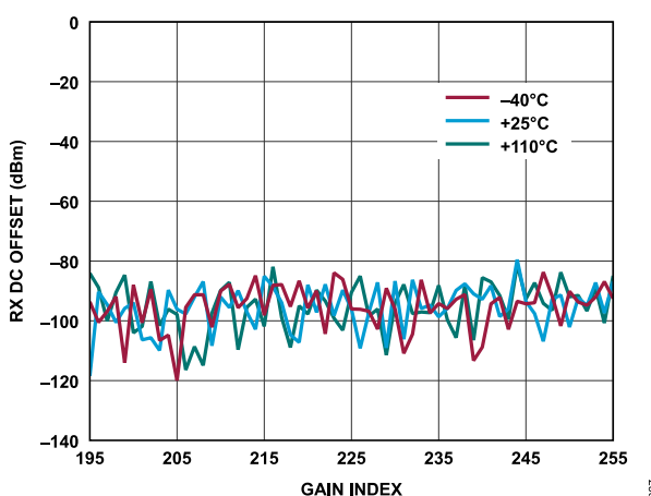
Figure 196. Receiver DC Offset vs. Gain Index, Baseband Frequency = 5.6 MHz, ADC = High Performance
