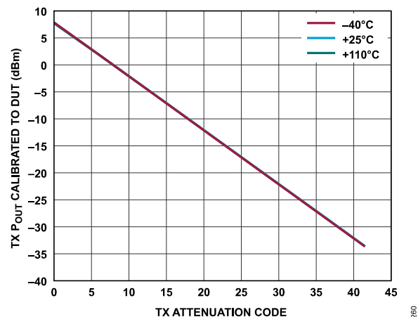
Figure 168. Transmitter Absolute Power vs. Transmitter Attenuation Code, Baseband Frequency = 18 MHz, Backoff = 0.2 dBFS
