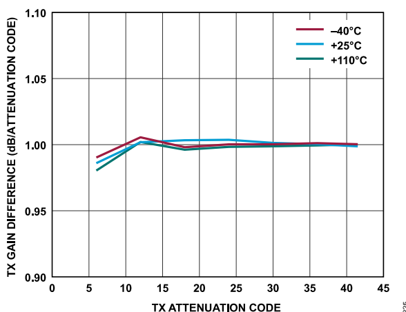
Figure 130. Transmitter Attenuation Delta (Error) vs. Transmitter Attenuation Code, Baseband Frequency = 18 MHz, Backoff = 0.2 dBFS
