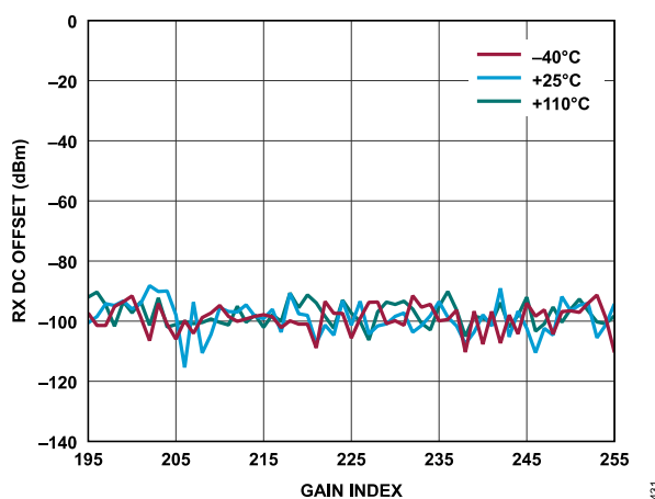
Figure 295. Receiver DC Offset vs. Gain Index, Baseband Frequency = 2.1 kHz, ADC = High Performance
