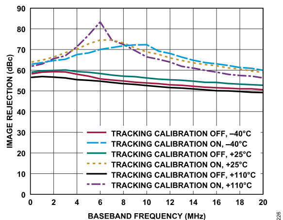
Figure 131. Transmitter Image Rejection vs. Baseband Frequency, Tracking Calibration On vs. Tracking Calibration Off, Transmitter Attenuation Code = 0
