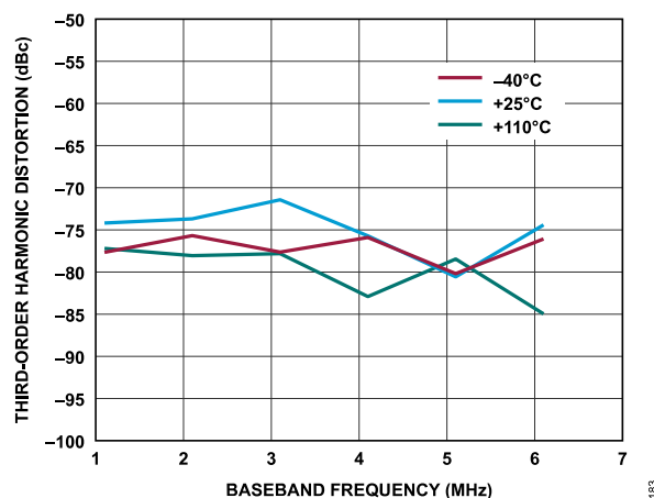
Figure 90. Receiver Third-Order Harmonic Distortion vs. Baseband Frequency, Gain Index = 255, ADC = Low Power
