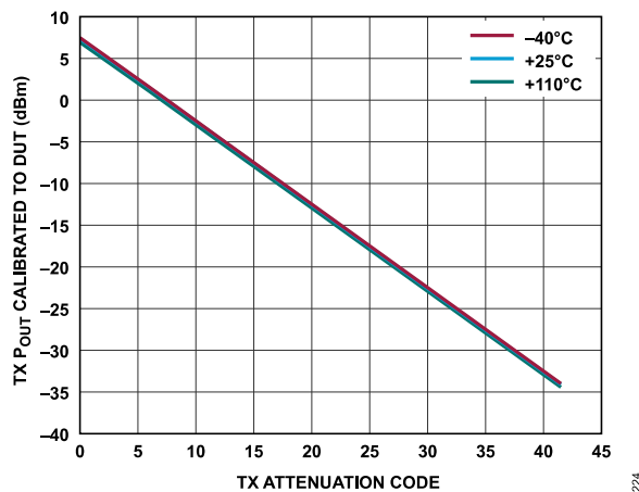
Figure 129. Transmitter Absolute Power vs. Transmitter Attenuation Code, Baseband Frequency = 18 MHz, Backoff = 0.2 dBFS
