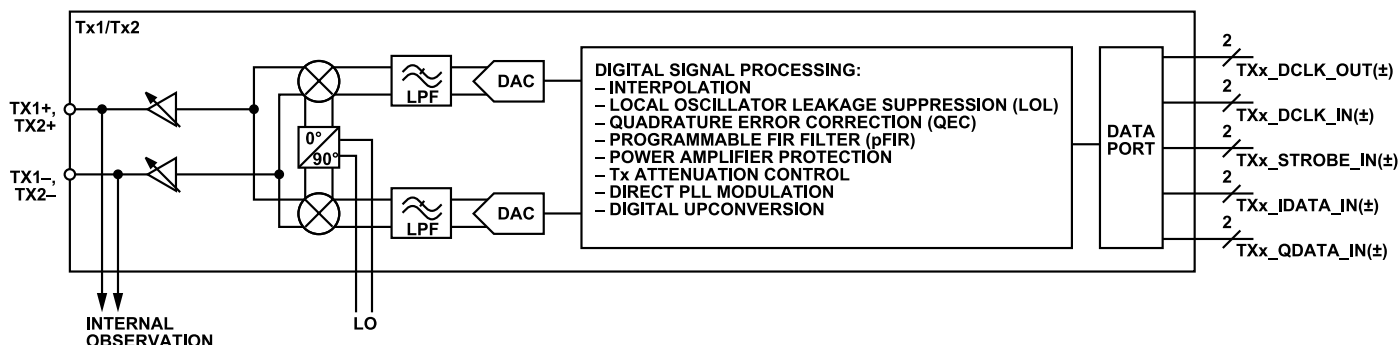
Figure 360. Transmitter Architecture
