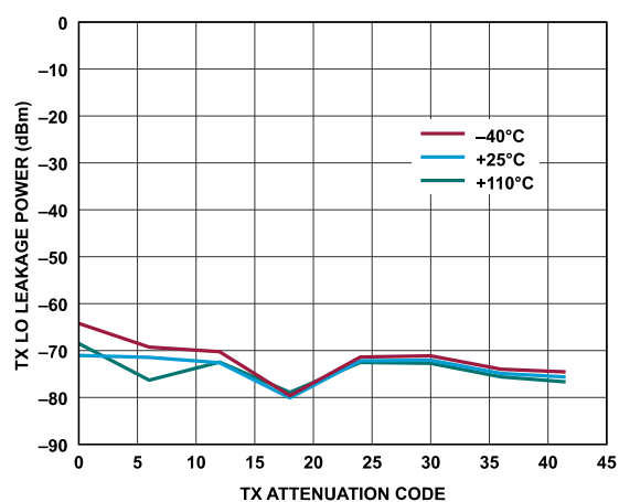
Figure 329. Transmitter LO Leakage Power vs. Transmitter Attenuation Code, Baseband Frequency = 2.1 kHz, Backoff = 6 dBFS, Initialization Calibration Only
