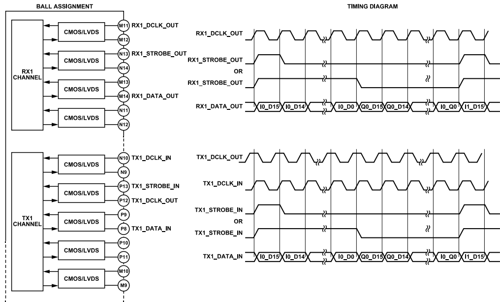
Figure 363. CSSI in 1-Lane Data Mode
