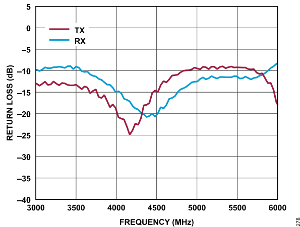
Figure 167. Receiver and Transmitter Return Loss vs. Frequency (For LO = 3 GHz to 6 GHz)
