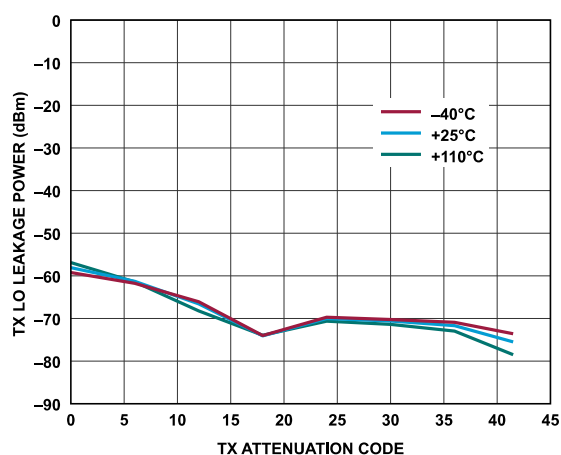
Figure 352. Transmitter LO Leakage Power vs. Transmitter Attenuation Code, Baseband Frequency = 2.1 kHz, Backoff = 6 dBFS, Initialization Calibration Only
