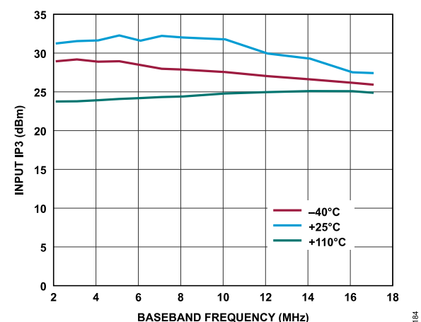
Figure 92. Receiver Input IP3 vs. Baseband Frequency, ADC = High Performance, f_1 = Baseband Frequency, f_2 = Baseband Frequency + 1 MHz, Gain Index = 255
