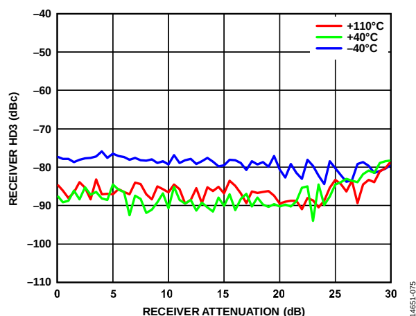
Figure 134. Receiver HD3 vs. Receiver Attenuation, 3500 MHz LO, CW Signal 17 MHz Offset, -14 dBm at 0 dB Attenuation, Input Power Increasing Decibel for Decibel with Attenuation, 100 MHz RF Bandwidth, 153.6 MSPS Sample Rate
