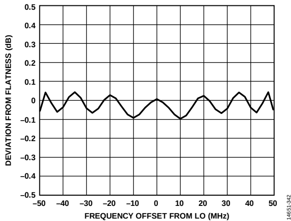
Figure 42. Transmitter Frequency Response Deviation from Flatness vs. Frequency Offset from LO, 800 MHz LO, 20 MHz RF Bandwidth, 6 dB Digital Backoff, 122.88 MSPS Sample Rate
