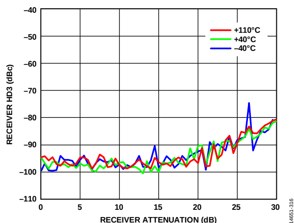
Figure 16. Receiver HD3 vs. Receiver Attenuation, 800 MHz LO, CW Signal 3 MHz Offset, -20 dBm at 0 dB Attenuation, Input Power Increasing Decibel for Decibel with Attenuation, 20 MHz RF Bandwidth, 30.72 MSPS Sample Rate
