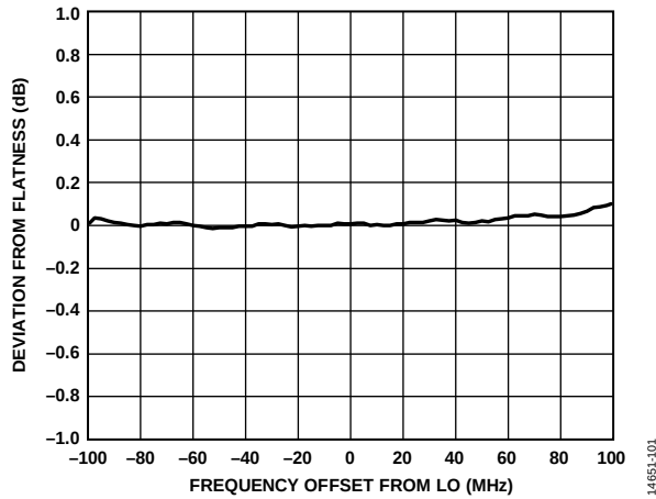
Figure 160. Transmitter Frequency Response Deviation from Flatness vs. Frequency Offset from LO, 3500 MHz LO, 100 MHz RF Bandwidth, 6 dB Digital Backoff, 307.2 MSPS Sample Rate
