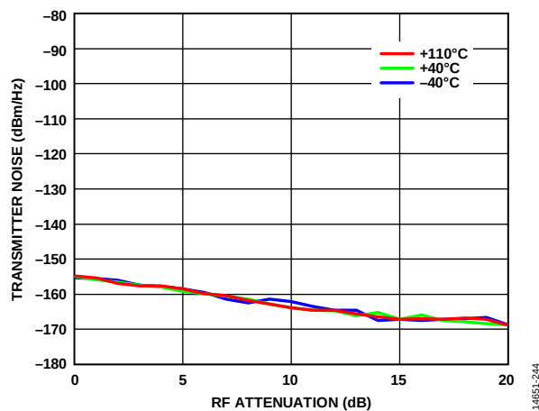
Figure 205. Transmitter Noise vs. RF Attenuation, 5600 MHz LO, 1 MHz Offset Frequency
