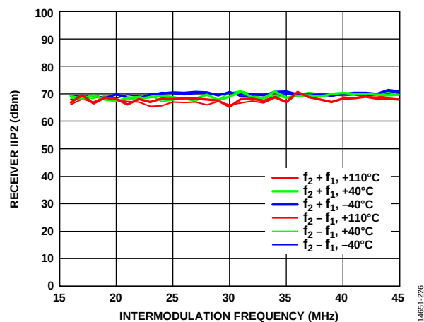
Figure 186. Receiver IIP2 vs. Intermodulation Frequency, 5600 MHz LO, 0 dB Attenuation, 100 MHz RF Bandwidth, 122.88 MSPS Sample Rate
