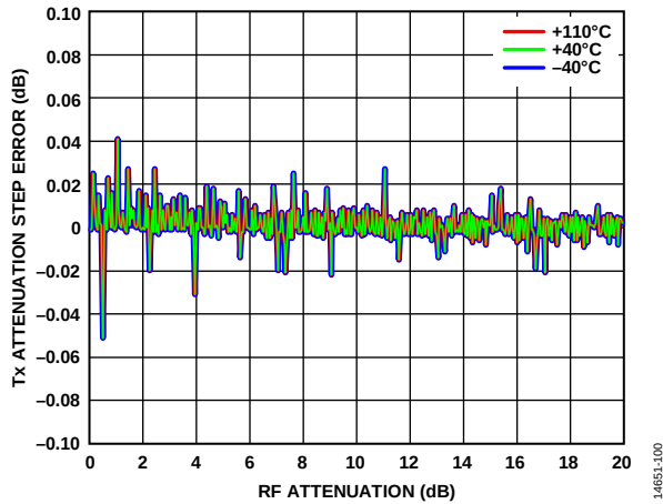
Figure 159. Tx Attenuation Step Error vs. RF Attenuation, 3500 MHz LO, 3510 MHz CW Desired Signal, 100 MHz RF Bandwidth, De-Embedded to Transmitter Port, 307.2 MSPS Sample Rate
