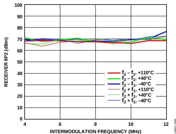
Figure 9. Receiver IIP2 vs. Intermodulation Frequency, 900 MHz LO, 0 dB Attenuation, 20 MHz RF Bandwidth, 30.72 MSPS Sample Rate
