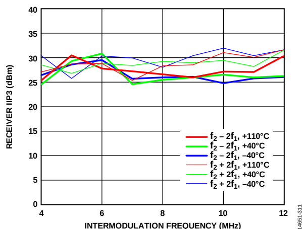
Figure 11. Receiver IIP3 vs. Intermodulation Frequency, 900 MHz LO, 0 dB Attenuation, 20 MHz RF Bandwidth, 30.72 MSPS Sample Rate
