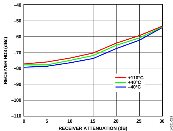
Figure 193. Receiver HD3 vs. Receiver Attenuation, 5600 MHz LO, CW Signal 10 MHz Offset, -20 dBm at 0 dB Attenuation, Input Power Increasing Decibel for Decibel with Attenuation, 100 MHz RF Bandwidth, 122.88 MSPS Sample Rate
