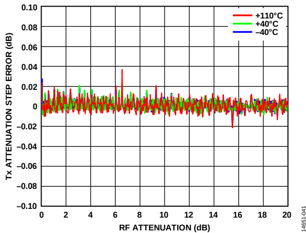
Figure 100. Tx Attenuation Step Error vs. RF Attenuation, 2600 MHz LO, 2610 MHz CW Desired Signal, 40 MHz RF Bandwidth, 245.76 MSPS Sample Rate
