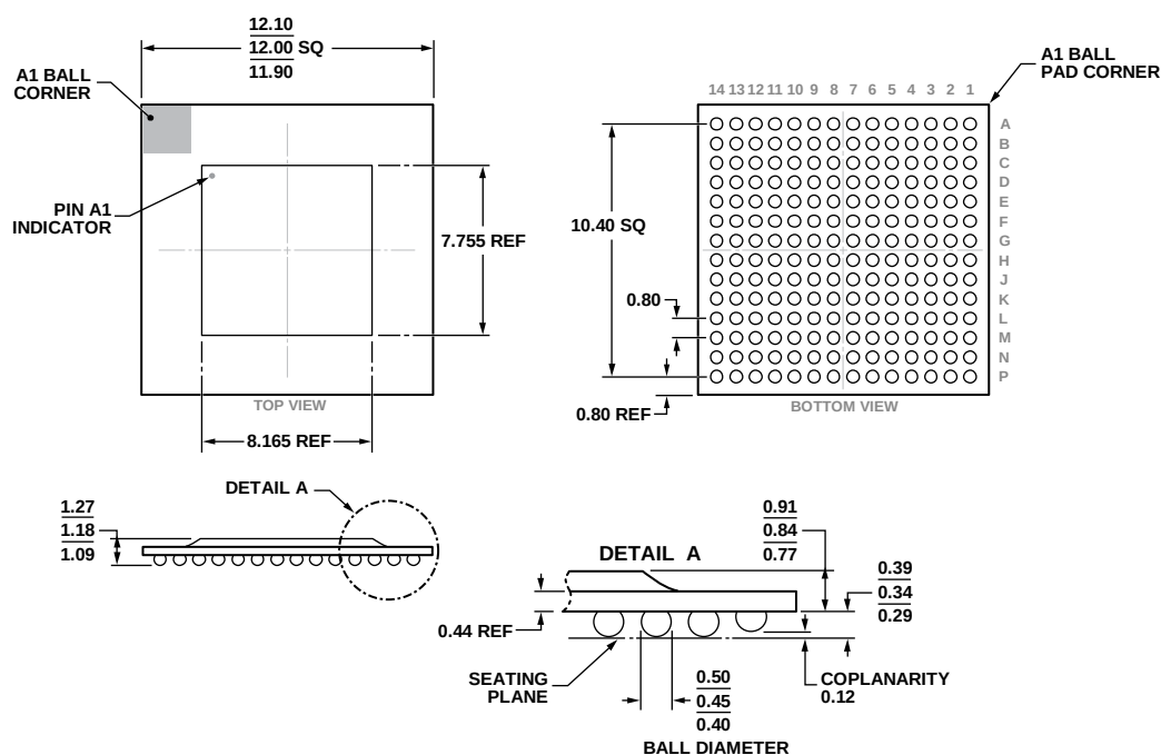
COMPLIANT TO JEDEC STANDARDS MO-275-GGAB-1. Figure 232. 196-Ball Chip Scale Package Ball Grid Array [CSP_BGA] (BC-196-12) Dimensions shown in millimeters
