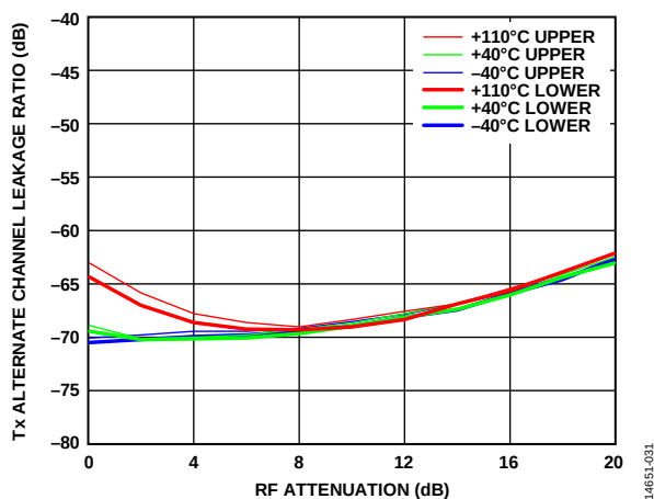
Figure 90. Tx Alternate Channel Leakage Ratio vs. RF Attenuation, 2600 MHz LO, 40 MHz RF Bandwidth, Four-Carrier W-CDMA Desired Signal, 2 dB Digital Backoff, Transmitter QEC and LO Leakage Tracking Active
