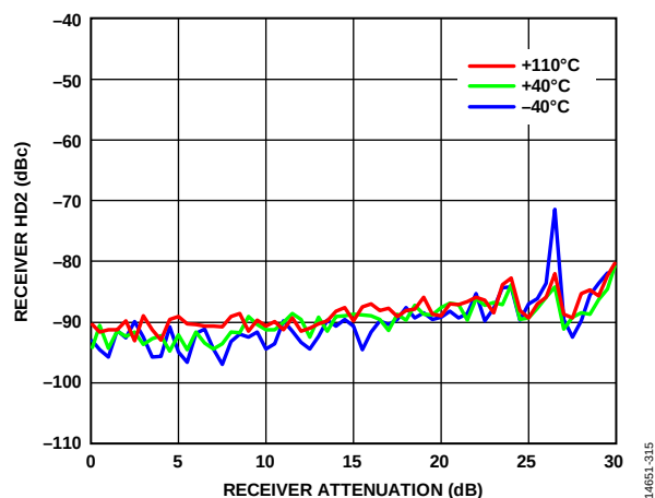
Figure 15. Receiver HD2 vs. Receiver Attenuation, 800 MHz LO, CW Signal 3 MHz Offset, -20 dBm at 0 dB Attenuation, Input Power Increasing Decibel for Decibel with Attenuation, 20 MHz RF Bandwidth, 30.72 MSPS Sample Rate
