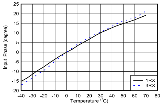
Figure 4-308. RX Input Phase vs Temperature and DSA at f_{\text{IN}} = 1.75 \text{ GHz}
