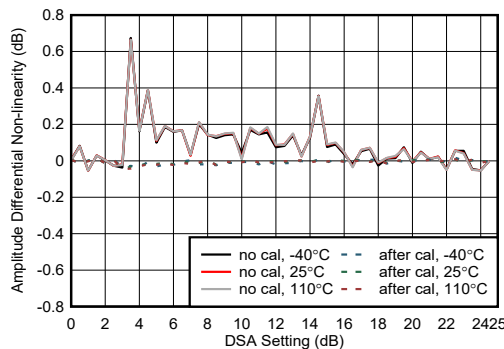
Figure 4-414. RX Amplitude Differential Nonlinearity at 8.1 GHz
