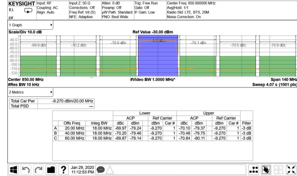
Figure 4-30. TX 20-MHz LTE Output Spectrum at 0.85 GHz
