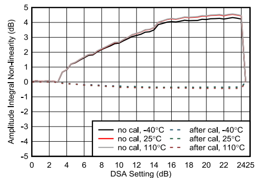
Figure 4-415. RX Amplitude Integrated Nonlinearity at 8.1 GHz
