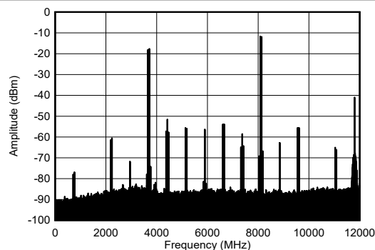
Figure 4-207. TX Dual Tone Output Spectrum at 8.11 GHz
