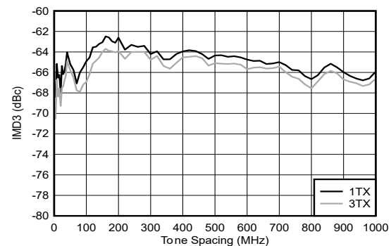
Figure 4-250. TX IMD3 vs Tone Spacing at 9.61 GHz
