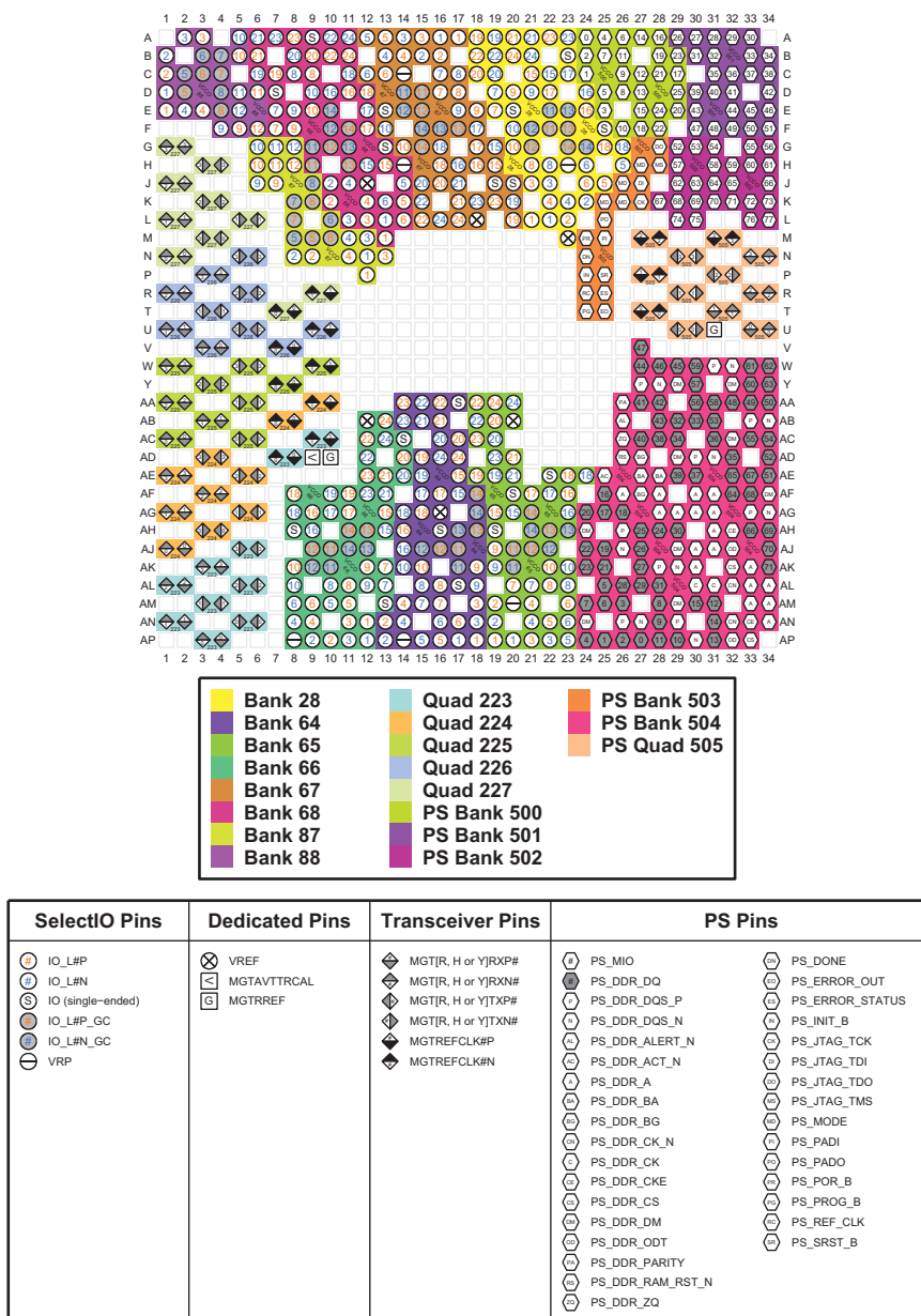
Figure 4-41: FFVC1156 Package—I/O Bank Diagram
