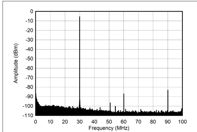
Figure 4-245. Single Tone Spectrum at 30 MHz and -12 dBFS (0 - 100 MHz)
