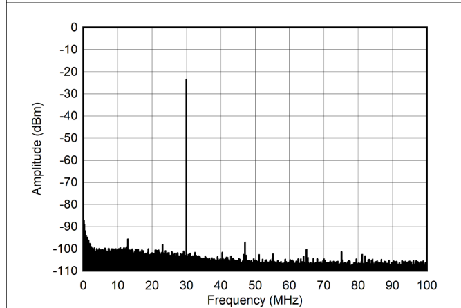
Figure 4-247. Single Tone Spectrum at 30 MHz and -30 dBFS (0 - 100 MHz)
