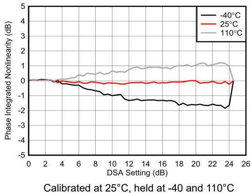
Figure 4-210. RX Calibrated Integrated Phase Error at 6.851 GHz
