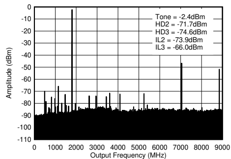
f_{\text{DAC}} = 8847.36\text{ MSPS} , straight mode, 1.8 GHz matching, includes PCB and cable losses. IL_n = f_{\text{S}}/n \pm f_{\text{OUT}} and is due to mixing with digital clocks.
