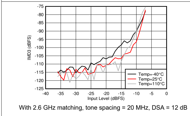
Figure 4-121. RX IMD3 vs Input Level and Temperature at 2.6 GHz
