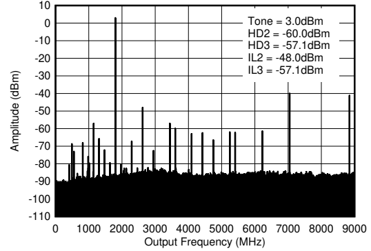
f_{\text{DAC}} = 8847.36\text{ MSPS} , interleave mode, 1.8 GHz matching, includes PCB and cable losses. IL_n = f_{\text{S}}/n \pm f_{\text{OUT}} .
