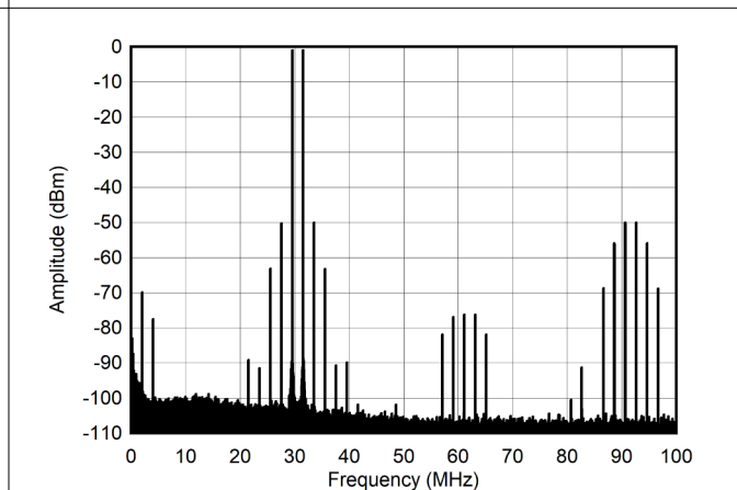
Figure 4-250. Dual Tone Spectrum at 30 MHz and -7 dBFS (0 - 100 MHz)
