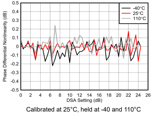
Figure 4-208. RX Calibrated Differential Phase Error at 6.851 GHz
