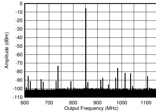
f_{DAC} = 5898.24 MSPS, interleave mode, 0.8 GHz matching, includes PCB and cable losses
