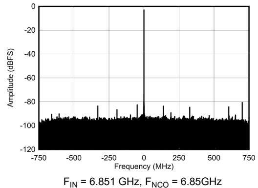
Figure 4-211. RX Output FFT at 6.851 GHz and -3 dBFS
