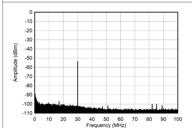
Figure 4-249. Single Tone Spectrum at 30 MHz and -60 dBFS (0 - 100 MHz)
