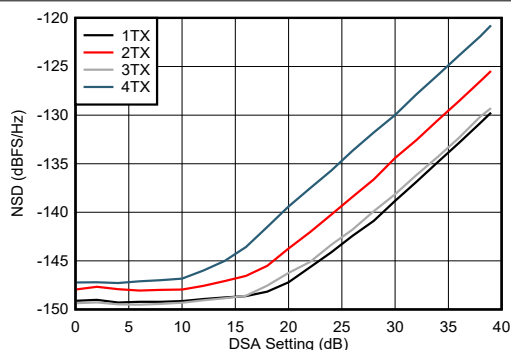
Figure 5-259. TX NSD vs DSA Setting at 9.61 GHz
