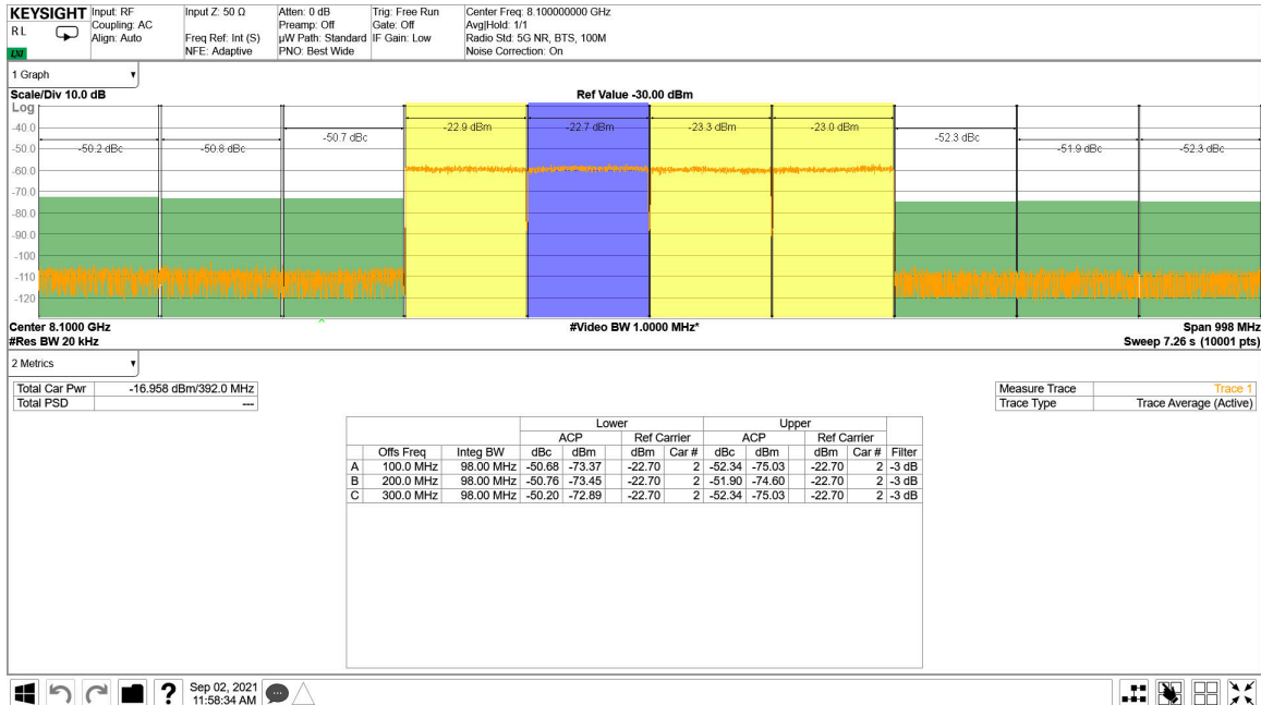
Figure 5-227. TX 4x100 MHz NR Output Spectrum 8.11 GHz
