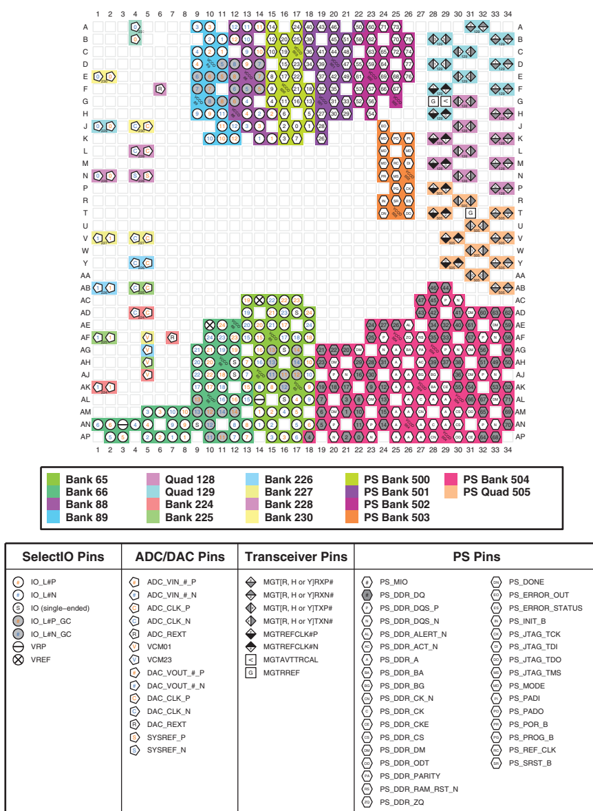
Figure 4-55: FFVE1156 and FSVE1156 Packages—XCZU43DR I/O Bank Diagram
