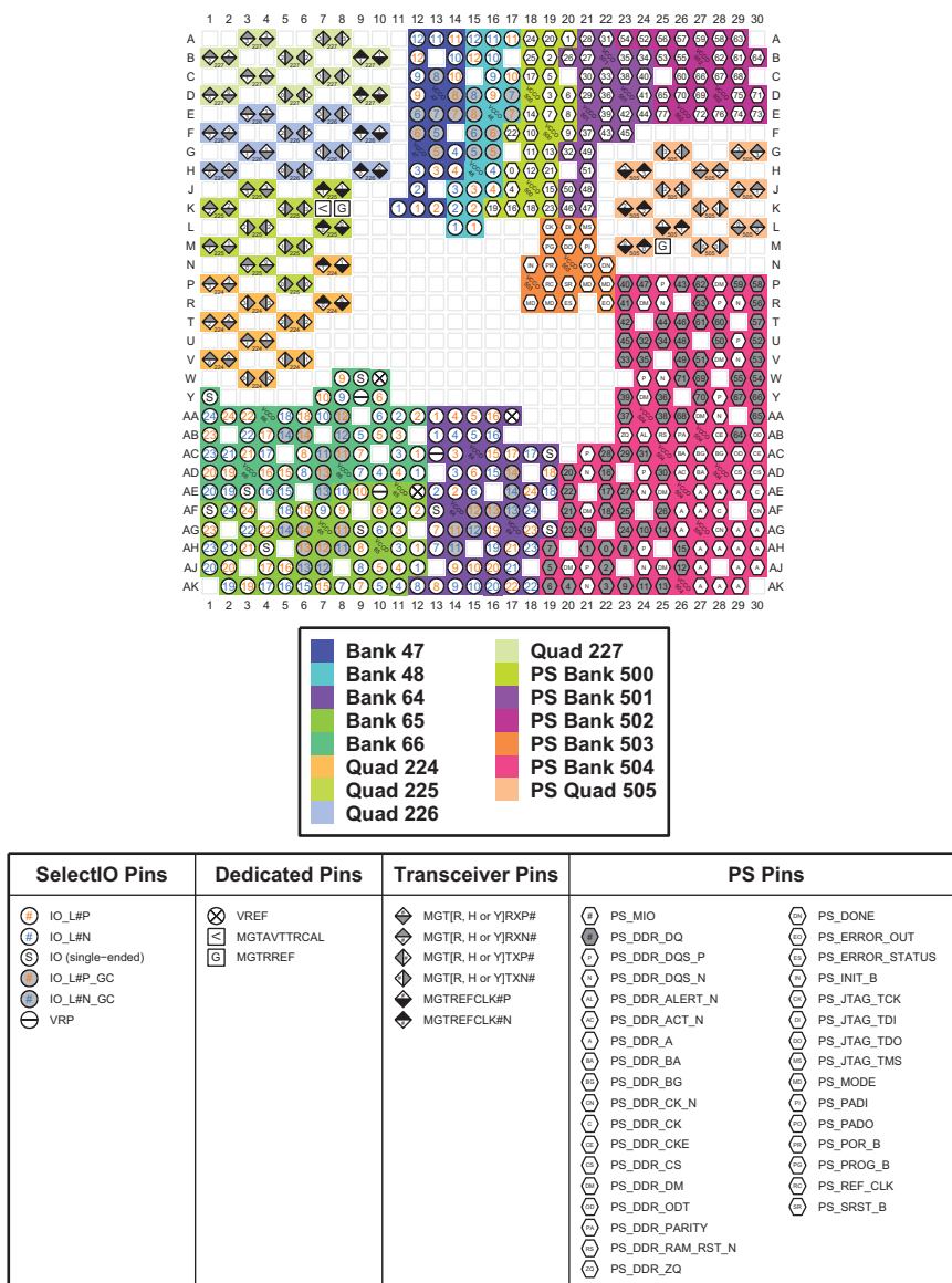
Figure 4-35: FBVB900 Package—XCZU7EV I/O Bank Diagram
