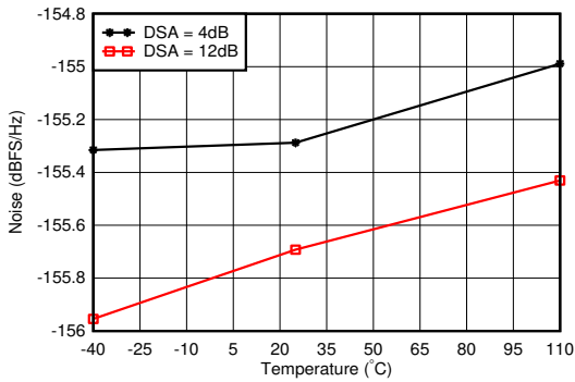
With 4.9 GHz matching, 12.5-MHz offset from tone
