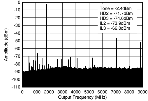
f_{\text{DAC}} = 8847.36 MSPS, straight mode, 1.8 GHz matching, includes PCB and cable losses. IL_n = f_S/n \pm f_{\text{OUT}} and is due to mixing with digital clocks.
