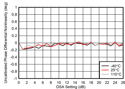
Figure 4-246. TX DSA Uncalibrated Phase Differential Nonlinearity
