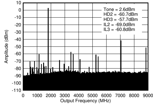
Figure 4-75. TX Single Tone (-12 dBFS) Output Spectrum at 1.8 GHz ( 0-f_{DAC} )
