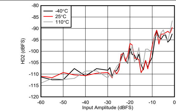
Figure 4-461. RX HD2 vs Digital Level at 9.6 GHz
