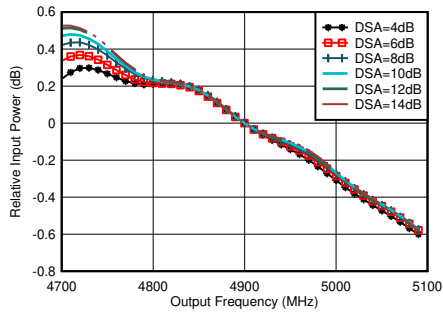
Figure 4-393. RX Inband Gain Flatness, f_{IN} = 4900\text{ MHz}
