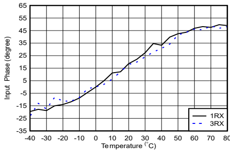
Figure 4-395. RX Input Phase vs Temperature and DSA at f_{OUT} = 4.9\text{ GHz}
