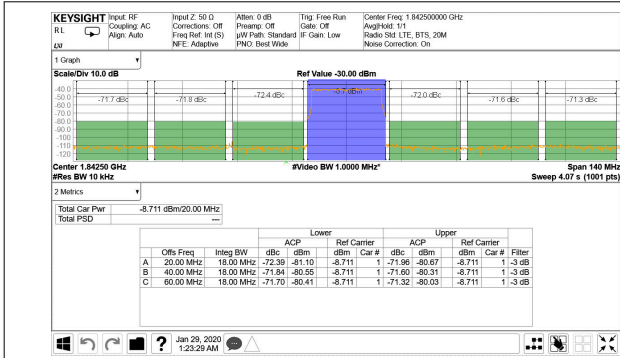
TM1.1, P_{\text{OUT,RMS}} = -13 dBFS
