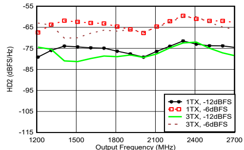
Matching at 1.8 GHz, f_{\text{DAC}} = 11.79648 GSPS, interleave mode, normalized to output power at harmonic frequency
