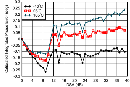
f_{\text{DAC}} = 8847.36 MSPS, straight mode, matching at 2.6 GHz, channel with the median variation over DSA setting at 25^\circ\text{C} Integrated Phase Error = Phase(DSA Setting) – Phase(DSA Setting = 0)
