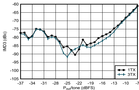
f_{DAC} = 11796.48 MSPS, interleave mode, f_{CENTER} = 1.8 GHz, f_{SPACING} = 20 MHz, matching at 1.8 GHz
