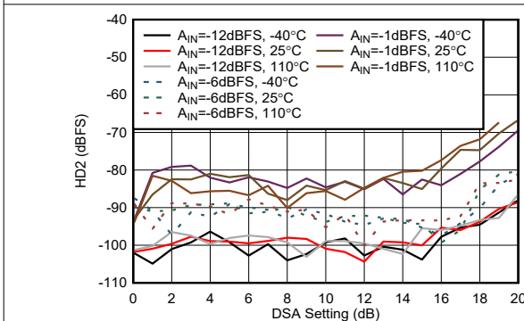
Figure 4-462. RX HD2 vs DSA Setting at 9.6 GHz
