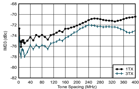
f_{DAC} = 11796.48 MSPS, interleave mode, f_{CENTER} = 1.8 GHz, matching at 1.8 GHz, -13 dBFS each tone
