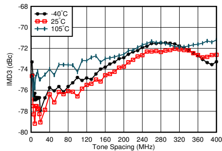
f_{DAC} = 11796.48 MSPS, interleave mode, f_{CENTER} = 1.8 GHz, matching at 1.8 GHz, -13 dBFS each tone, worst channel
