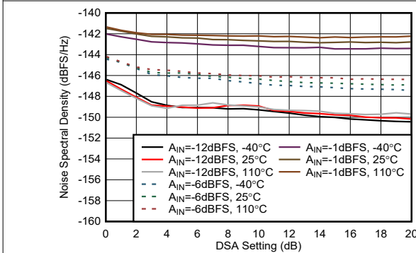
Figure 4-460. RX NSD vs DSA Setting at 9.6 GHz
