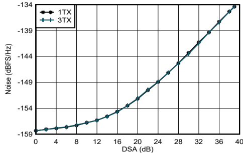
f_{DAC} = 5898.24 MSPS, interleave mode, matching at 1.8 GHz, P_{OUT} = -13 dBFS
