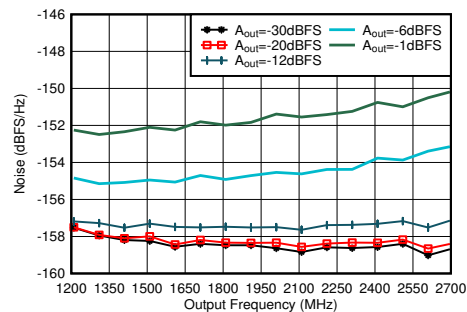
Matching at 2.6 GHz, Single tone, f_{DAC} = 11.79648 MSPS, interleave mode, 40-MHz offset
