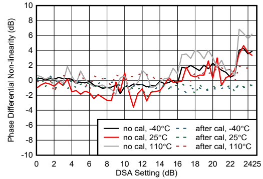
Figure 4-453. RX Phase Integrated Non-linearity at 9.6 GHz
