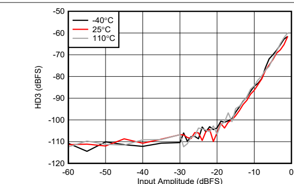
Figure 4-463. RX HD3 vs Digital Level at 9.6 GHz
