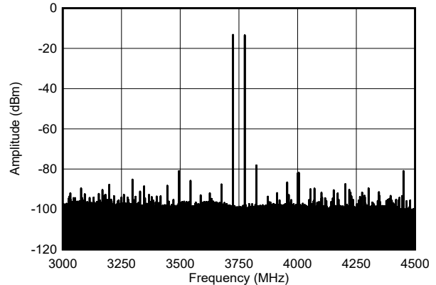
Figure 5-471. TX Dual Tone Output Spectrum at 3.75 GHz, -13dBFS each ( \pm 600\text{ MHz} )
