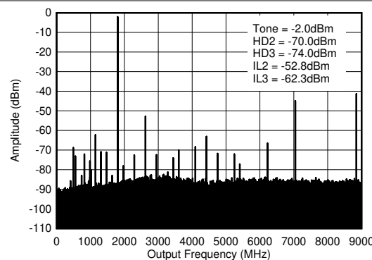
f_{\text{DAC}} = 8847.36\text{MSPS} , interleave mode, 1.8 GHz matching, includes PCB and cable losses. \text{ILn} = f_{\text{S}}/\text{n} \pm f_{\text{OUT}} . Figure 5-343. TX Single Tone (-6 dBFS) Output Spectrum at 1.8 GHz ( 0-f_{\text{DAC}} )
