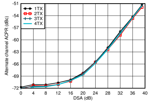
Figure 5-388. TX 20-MHz LTE alt-ACPR vs DSA at 2.6 GHz
