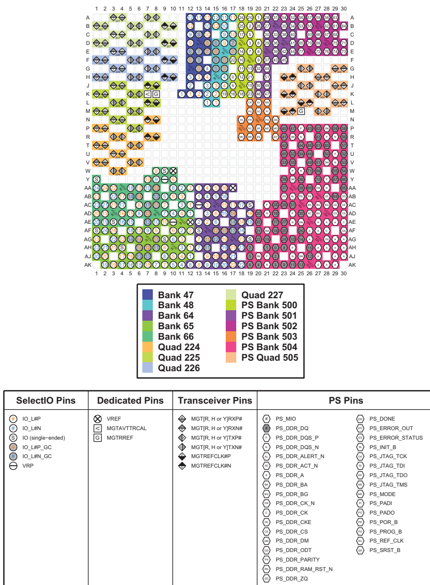
Figure 4-33: FBVB900 Package—I/O Bank Diagram
