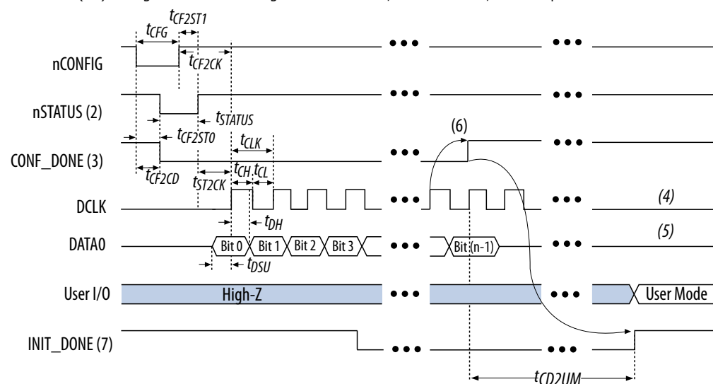
Figure 32. PS Configuration Timing Waveform
