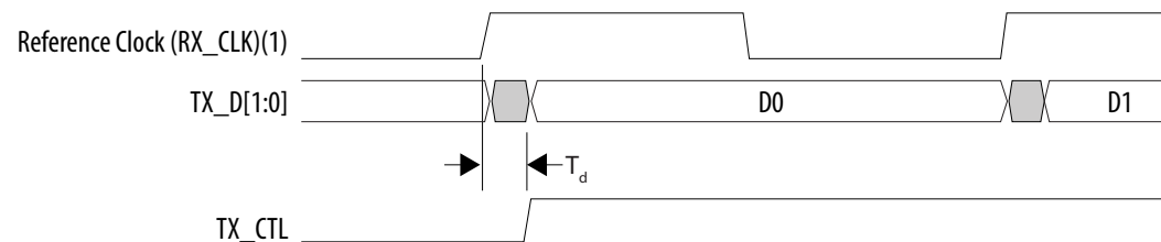
Figure 14. RMII TX Timing Diagram
