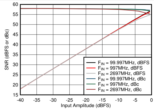
Figure 5-32. SNR vs Input Amplitude
