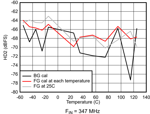
Figure 5-45. HD2 vs Temperature
