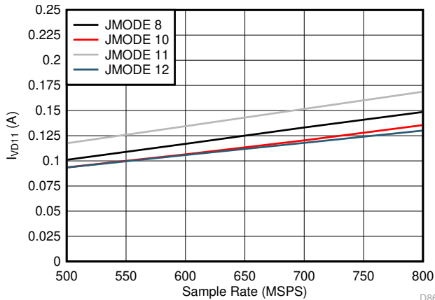
Figure 5-109. Single Channel, I_{VD11} vs F_S for JMODES 8 - 12
