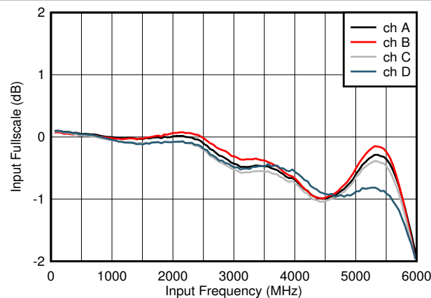
Figure 5-3. Input Fullscale vs Input Frequency
