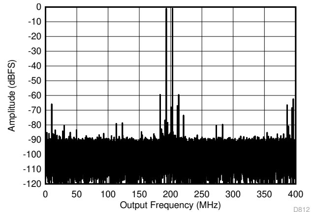
Figure 5-70. Two Tone FFT at 1798 MHz in Low Power Mode
