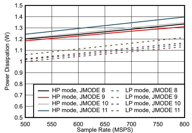
Figure 5-90. Dual Channel, Power Dissipation vs F_S for JMODES 8 - 11
