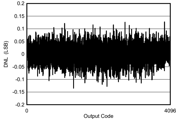
Figure 5-1. DNL vs Code
