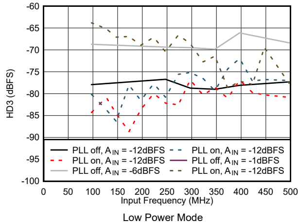
Figure 5-51. HD3 vs Input Frequency in Low Power Mode
