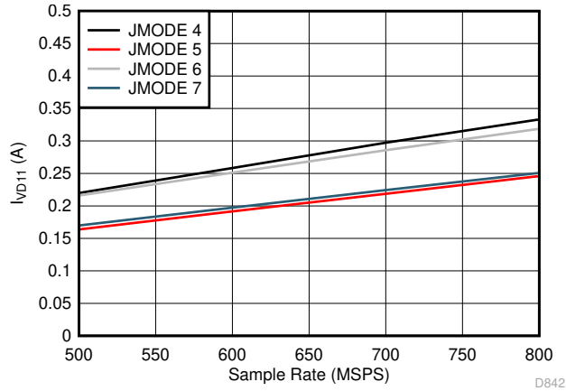
Figure 5-81. Quad Channel, I_{VD11} vs F_S for JMODES 4 - 7
