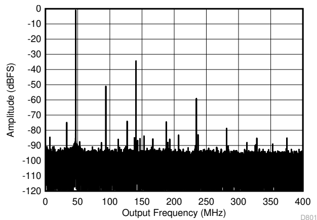
Figure 5-13. Single Tone FFT at 3247 MHz and -1dBFS
