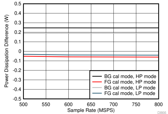
Figure 5-98. Dual Channel, Power Dissipation vs F_S over Modes
