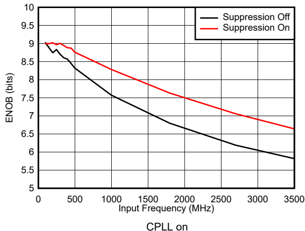
Figure 5-37. ENOB vs Input Frequency and Suppression
