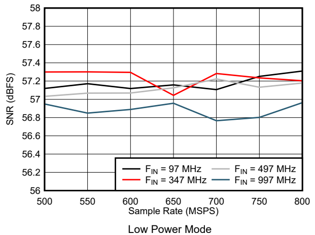
Figure 5-54. SNR vs Sample Rate in Low Power Mode
