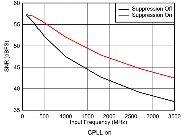
Figure 5-34. SNR vs Input Frequency and Suppression
