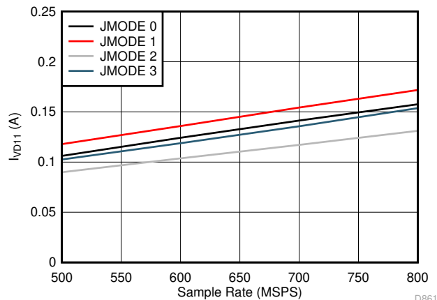
Figure 5-107. Single Channel, I_{VD11} vs F_S for JMODES 0 - 3
