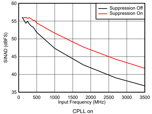
Figure 5-36. SINAD vs Input Frequency and Suppression
