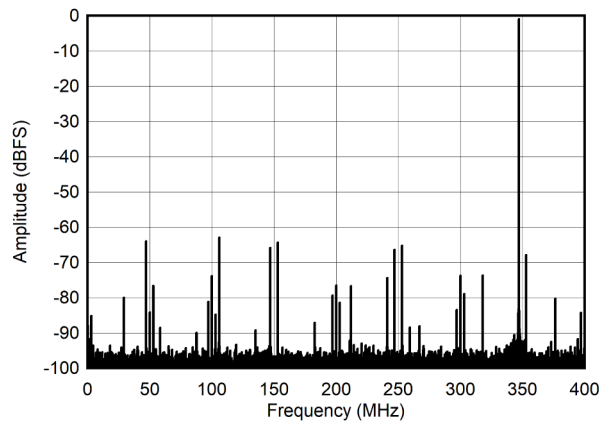
Figure 5-18. Single Tone FFT at 347 MHz and -1dBFS
