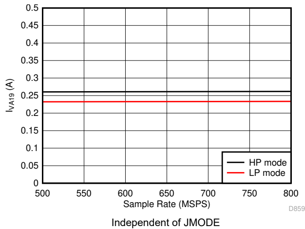
Figure 5-105. Single Channel, I_{VA19} vs F_S
