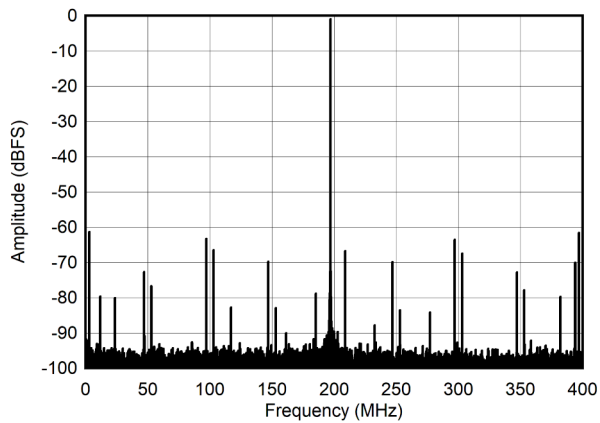
Figure 5-17. Single Tone FFT at 997 MHz and -1dBFS
