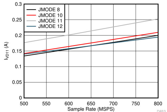
Figure 5-96. Dual Channel, I_{VD11} vs F_S for JMODES 8 - 12
