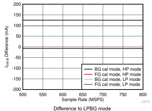
Figure 5-112. Single Channel, I_{VA19} vs F_S over Modes
