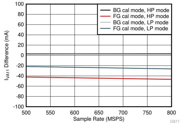
Figure 5-86. Quad Channel, I_{VA11} vs F_S over Modes
