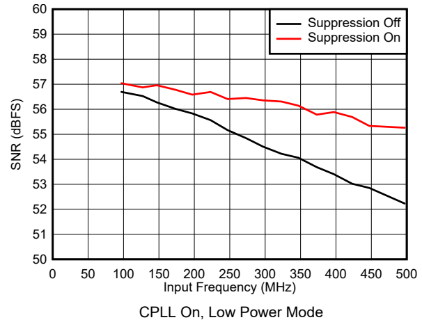
Figure 5-60. SNR vs Input Frequency
