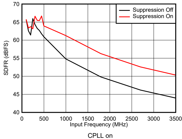
Figure 5-35. SFDR vs Input Frequency and Suppression
