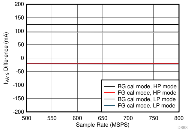
Figure 5-85. Quad Channel, I_{VA19} vs F_S over Modes
