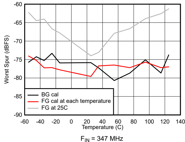
Figure 5-47. worst non-HD spur vs Temperature
