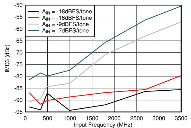
Figure 5-72. IMD3 vs Input Frequency
