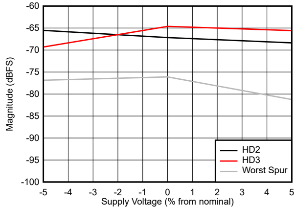
Figure 5-39. HD2, HD3 and worst non-HD vs Supply Voltage
