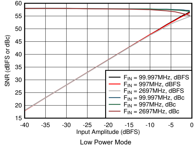
Figure 5-58. SNR vs Input Amplitude in Low Power Mode
