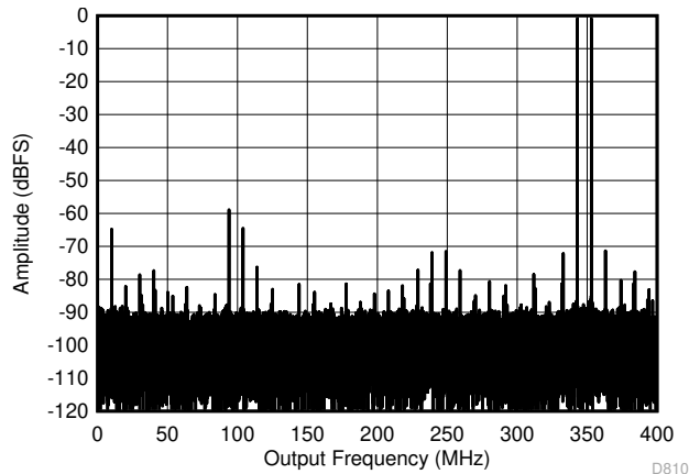
Figure 5-69. Two Tone FFT at 347 MHz in Low Power Mode
