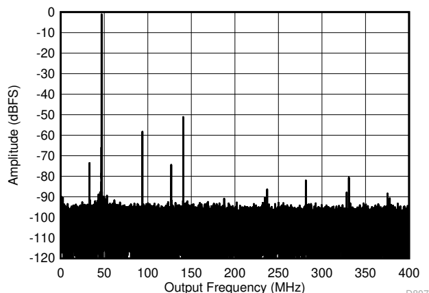
Figure 5-9. Single Tone FFT at 3247 MHz and -1dBFS
