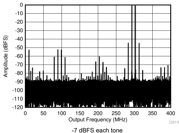
Figure 5-71. Two Tone FFT at 3498 MHz in Low Power Mode
