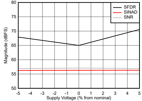
Figure 5-64. SNR, SFDR and SINAD vs Supply Voltage
