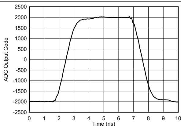
Figure 7-2. Measured Pulse using Sub-Sampling Technique for Equivalent 25.6 GSPS Measurement
