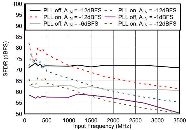
Figure 5-23. SFDR vs Input Frequency
