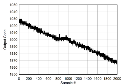
Figure 5-116. Background Calibration Core Transition (voltage offset)
