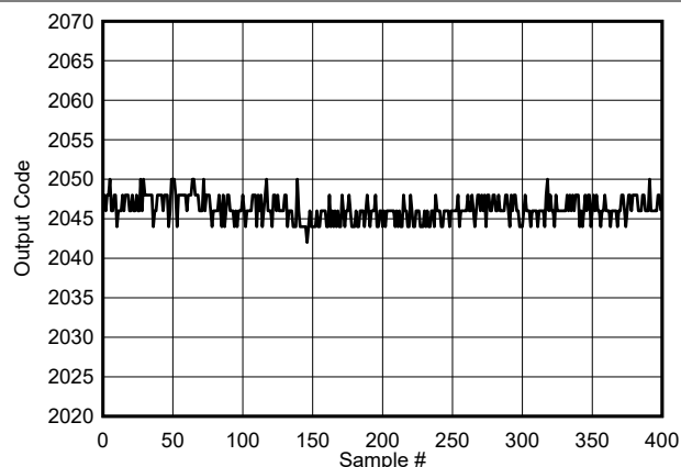
Figure 5-115. Background Calibration Core Transition (midscale)
