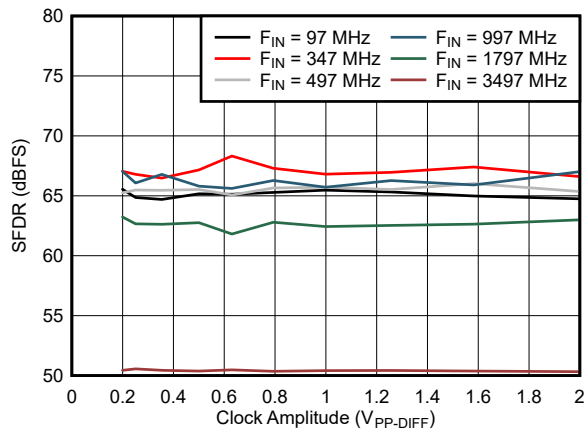
Figure 5-41. SFDR vs Clock Amplitude
