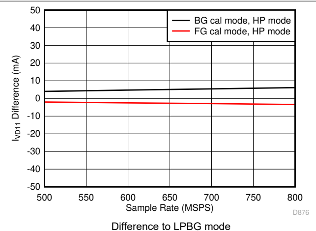
Figure 5-114. Single Channel, I_{VD11} vs F_S over Modes
