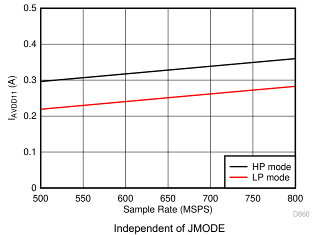
Figure 5-106. Single Channel, I_{VA11} vs F_S
