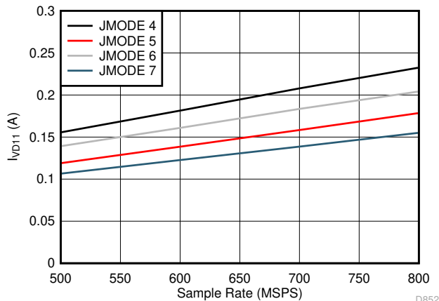
Figure 5-95. Dual Channel, I_{VD11} vs F_S for JMODES 4 - 7
