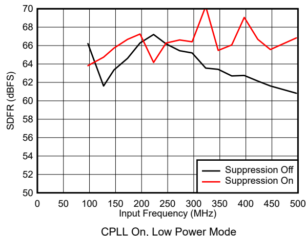
Figure 5-61. SFDR vs Input Frequency
