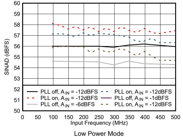
Figure 5-52. SINAD vs Input Frequency in Low Power Mode
