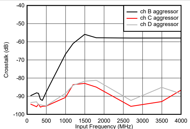
Figure 5-4. Crosstalk vs Input Frequency, Channel A victim
