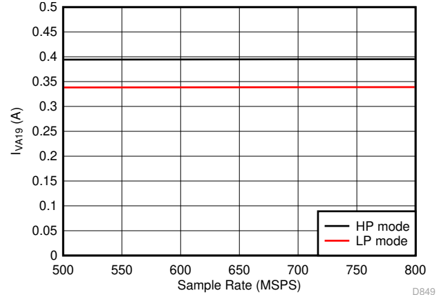
Figure 5-92. Dual Channel, I_{VA19} vs F_S Independent of JMODE
