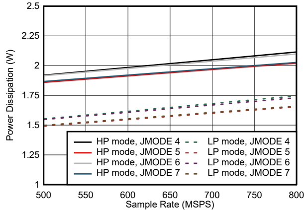
Figure 5-75. Quad Channel, Power Dissipation vs F_S for JMODES 4 - 7
