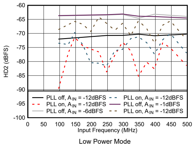
Figure 5-50. HD2 vs Input Frequency in Low Power Mode
