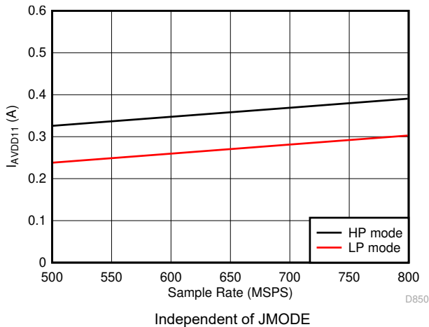
Figure 5-93. Dual Channel, I_{VA11} vs F_S Independent of JMODE
