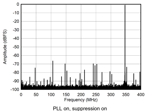
Figure 5-15. Single Tone FFT at 347 MHz and -1dBFS
