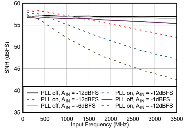
Figure 5-22. SNR vs Input Frequency
