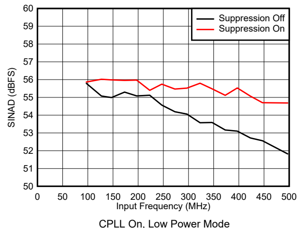
Figure 5-62. SINAD vs Input Frequency
