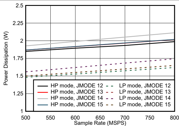
Figure 5-77. Quad Channel, Power Dissipation vs F_S for JMODES 12 - 15
