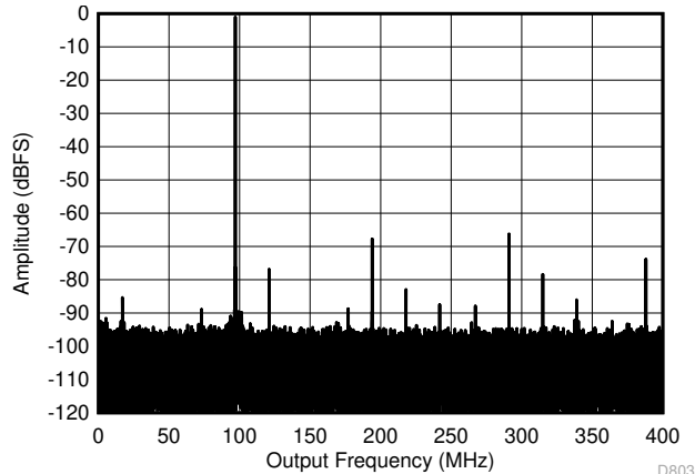
Figure 5-7. Single Tone FFT at 897 MHz and -1dBFS
