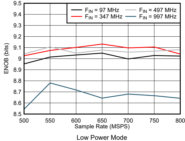
Figure 5-57. ENOB vs Sample Rate in Low Power Mode
