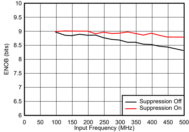
Figure 5-63. ENOB vs Input Frequency
