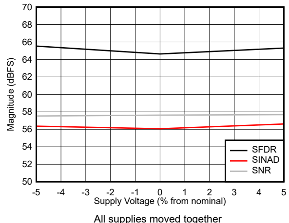
Figure 5-38. SNR, SFDR and SINAD vs Supply Voltage
