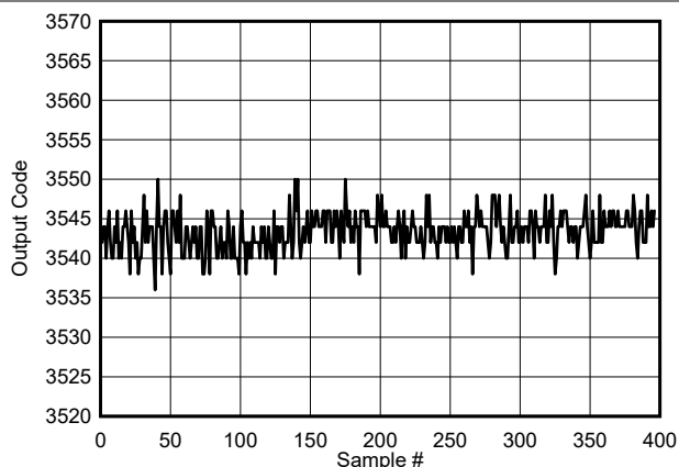
Figure 5-116. Background Calibration Core Transition (voltage offset)
