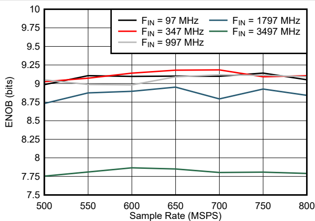
Figure 5-31. ENOB vs Sample Rate
