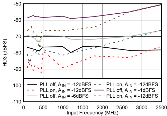
Figure 5-25. HD3 vs Input Frequency
