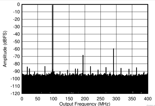
Figure 5-11. Single Tone FFT at 897 MHz and -1dBFS
