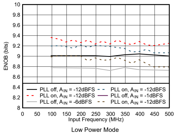
Figure 5-53. ENOB vs Input Frequency in Low Power Mode
