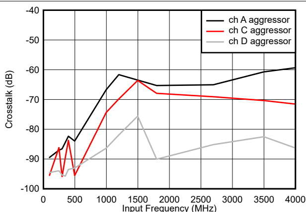
Figure 5-5. Crosstalk vs Input Frequency, Channel B victim
