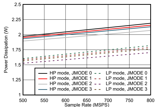
Figure 5-74. Quad Channel, Power Dissipation vs F_S for JMODES 0 - 3
