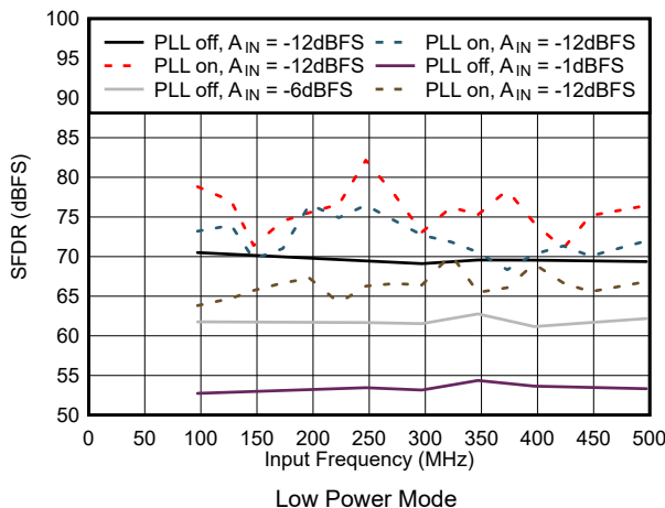
Figure 5-49. SFDR vs Input Frequency in Low Power Mode
