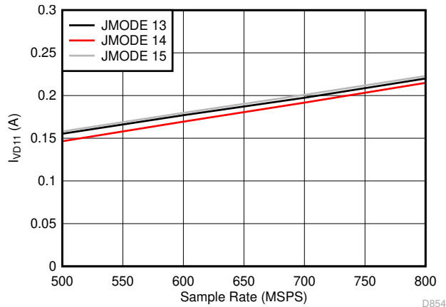
Figure 5-97. Dual Channel, I_{VD11} vs F_S for JMODES 13 - 15
