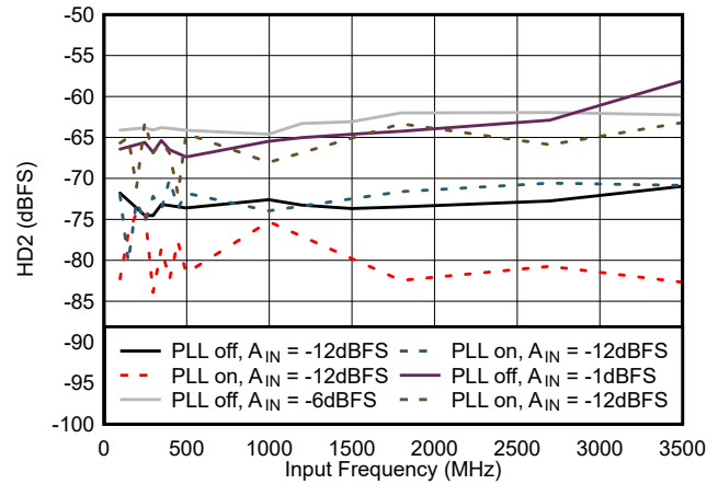
Figure 5-24. HD2 vs Input Frequency
