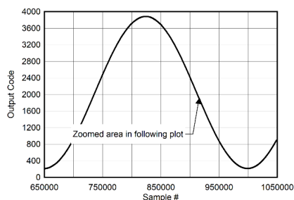
Figure 5-115. Background Calibration Core Transition (midscale)
