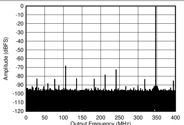
Figure 5-6. Single Tone FFT at 347 MHz and -1dBFS
