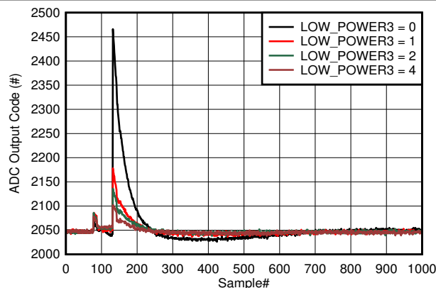
Figure 6-12. Background Calibration Core Transition In Low Power Mode
