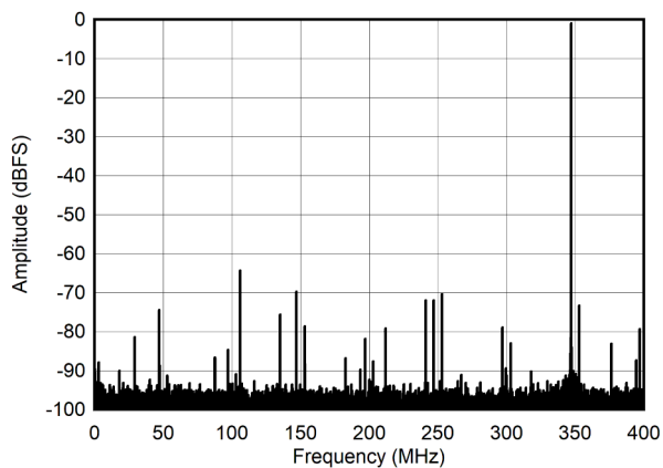
Figure 5-19. Single Tone FFT at 347 MHz and -1dBFS
