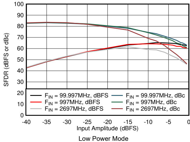
Figure 5-59. SFDR vs Input Amplitude in Low Power Mode
