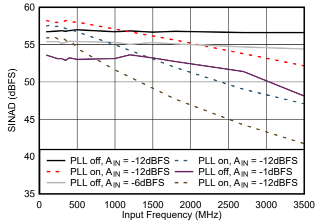
Figure 5-26. SINAD vs Input Frequency
