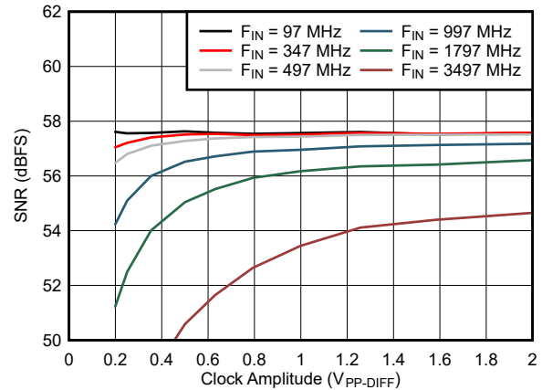
Figure 5-40. SNR vs Clock Amplitude
