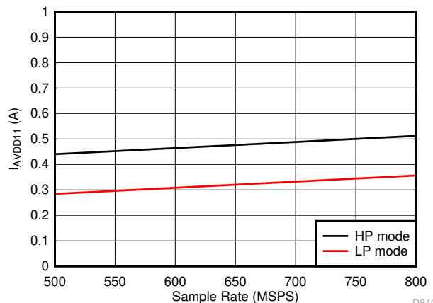
Figure 5-79. Quad Channel, I_{VA11} vs F_S
