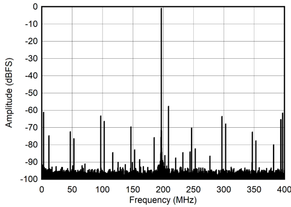
Figure 5-21. Single Tone FFT at 997 MHz and -1dBFS
