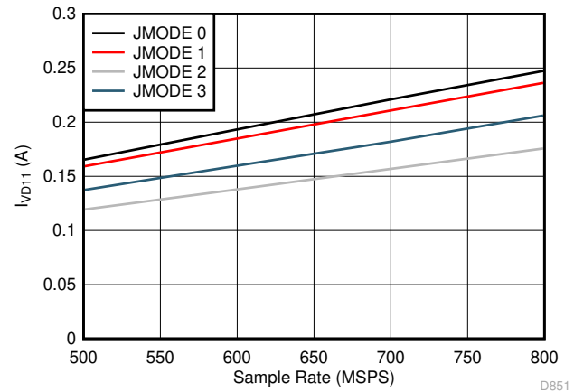
Figure 5-94. Dual Channel, I_{VD11} vs F_S for JMODES 0 - 3
