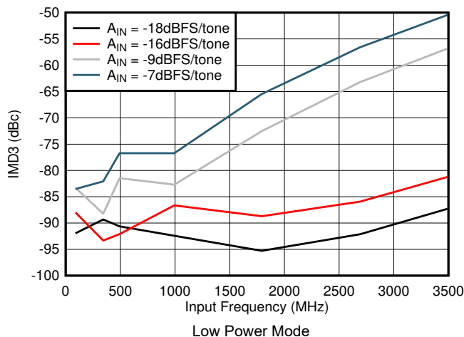
Figure 5-73. IMD3 vs Input Frequency in Low Power Mode
