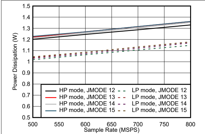
Figure 5-91. Dual Channel, Power Dissipation vs F_S for JMODES 12 - 15
