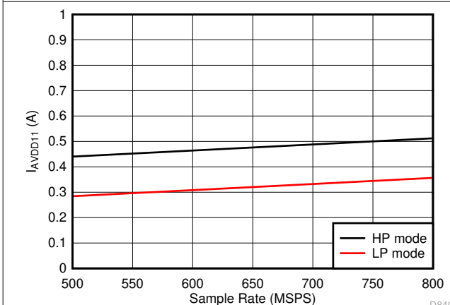
Figure 5-79. Quad Channel, I_{VA11} vs F_S
