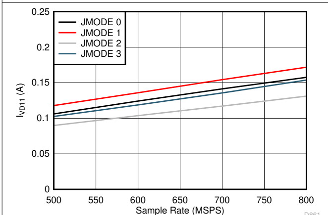
Figure 5-107. Single Channel, I_{VD11} vs F_S for JMODES 0 - 3
