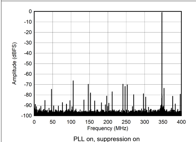
Figure 5-15. Single Tone FFT at 347 MHz and -1dBFS
