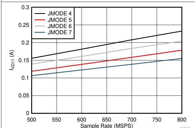
Figure 5-95. Dual Channel, I_{VD11} vs F_S for JMODES 4 - 7
