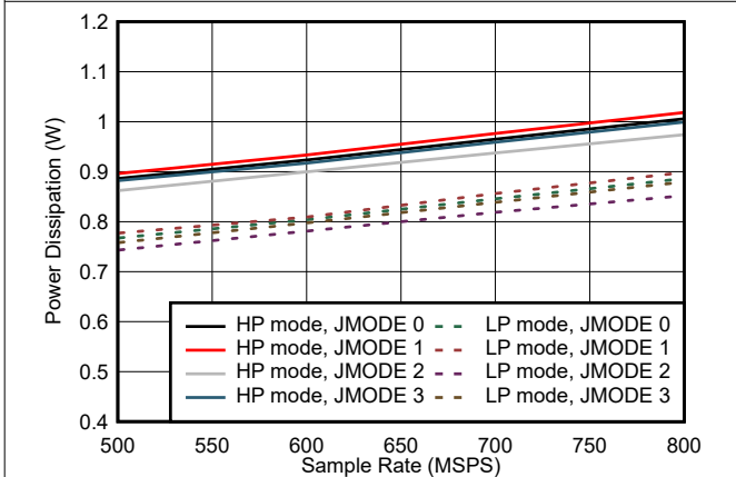
Figure 5-101. Dual Channel, Power Dissipation vs F_S for JMODES 0 - 3
