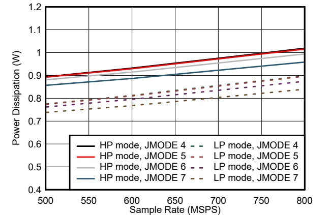
Figure 5-102. Single Channel, Power Dissipation vs F_S for JMODES 4 - 7
