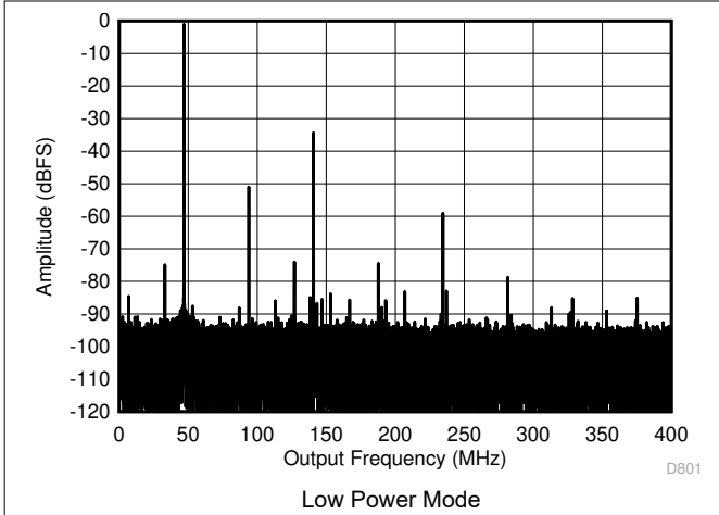
Figure 5-13. Single Tone FFT at 3247 MHz and -1dBFS
