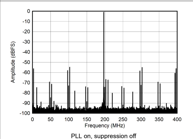
Figure 5-16. Single Tone FFT at 997 MHz and -1dBFS
