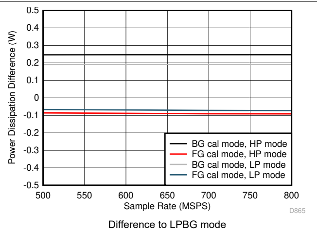
Figure 5-84. Quad Channel, Power Dissipation vs F_S over Modes
