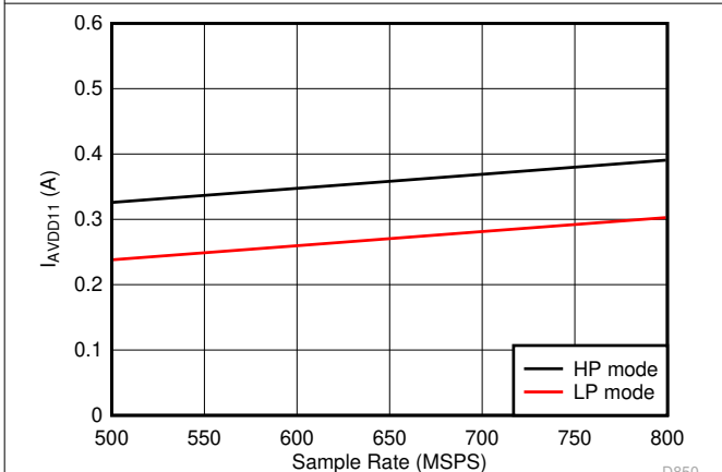
Figure 5-93. Dual Channel, I_{VA11} vs F_S Independent of JMODE
