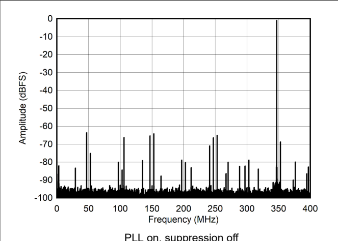
Figure 5-14. Single Tone FFT at 347 MHz and -1dBFS
