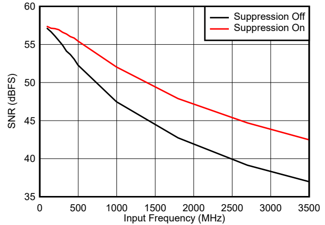
Figure 5-34. SNR vs Input Frequency and Suppression
