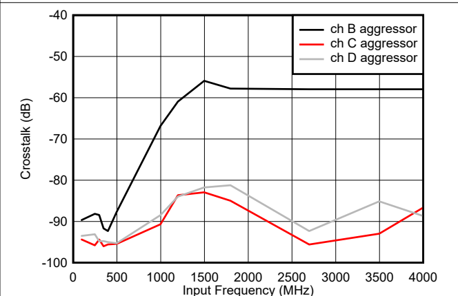
Figure 5-4. Crosstalk vs Input Frequency, Channel A victim
