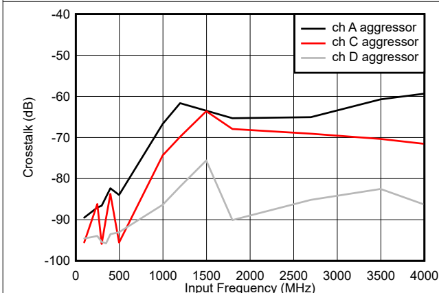
Figure 5-5. Crosstalk vs Input Frequency, Channel B victim
