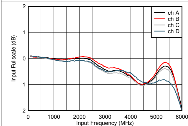
Figure 5-3. Input Fullscale vs Input Frequency
