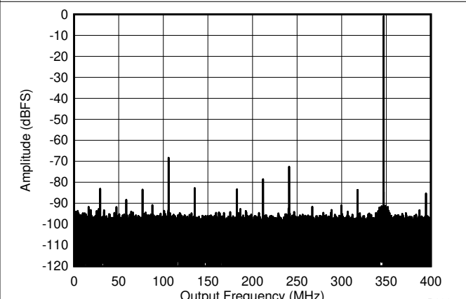
Figure 5-6. Single Tone FFT at 347 MHz and -1dBFS
