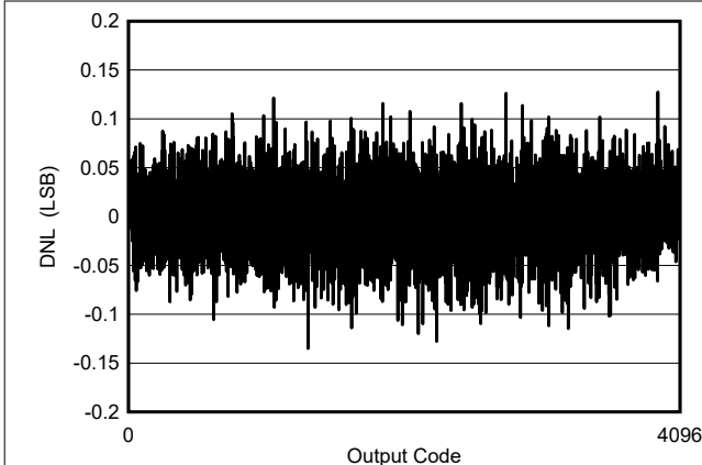
Figure 5-1. DNL vs Code
