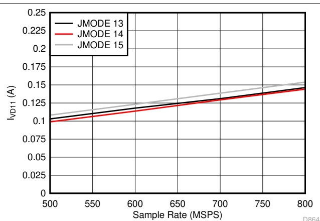
Figure 5-110. Single Channel, I_{VD11} vs F_S for JMODES 13 - 15
