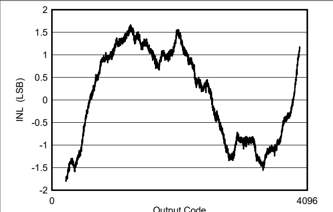
Figure 5-2. INL vs Code
