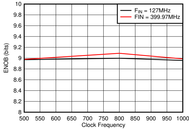
Figure 6-31. ENOB vs Sample Rate
