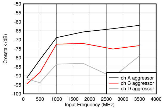
Figure 6-78. Crosstalk to Channel B vs F_{IN}
