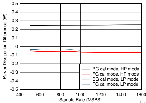
Figure 6-111. Single Channel, Power Dissipation Change with Calibration Mode
