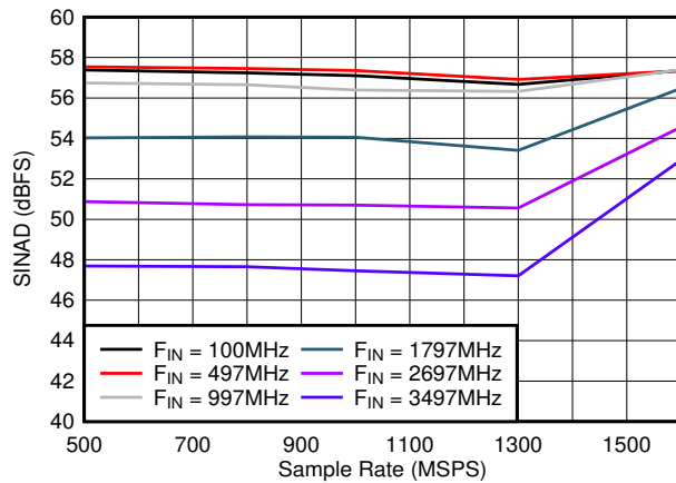
Figure 6-25. SINAD vs Sample Rate
