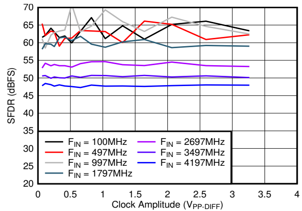
Figure 6-36. SFDR vs A_{CLK}
