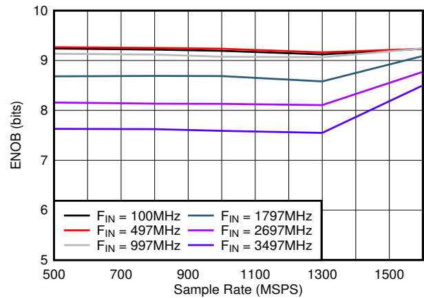
Figure 6-26. ENOB vs Sample Rate
