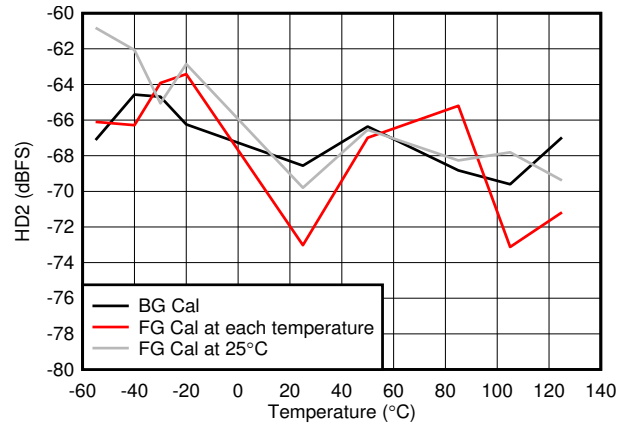
Figure 6-66. HD2 vs Temperature
