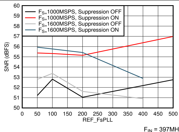
Figure 6-38. SNR vs F_{REF} and Suppression
