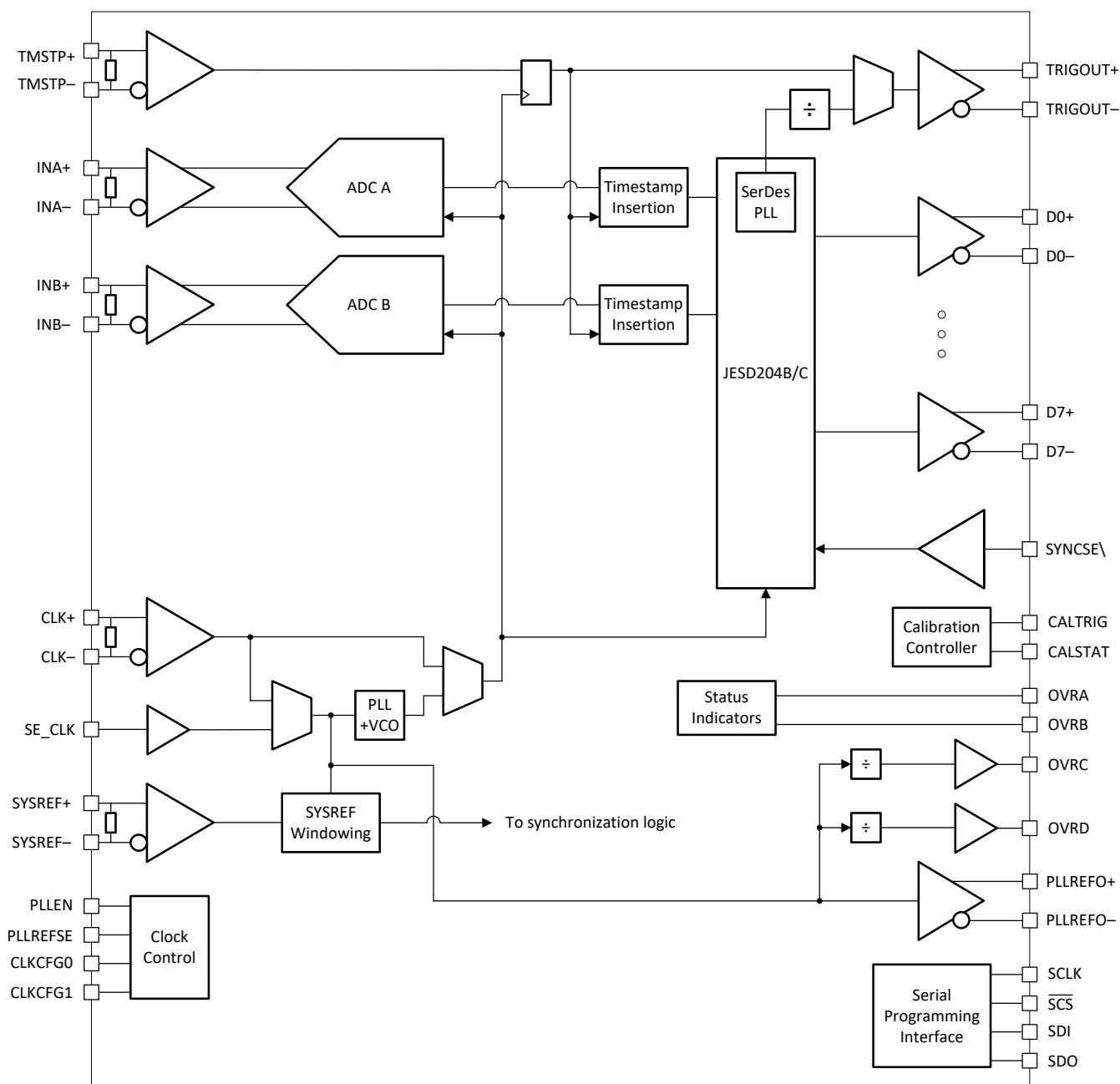
Figure 7-2. Dual Channel Functional Block Diagram
