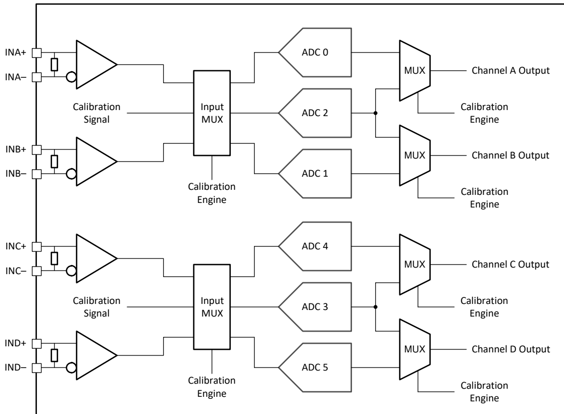
Figure 7-15. Quad Channel Calibration System Block Diagram
