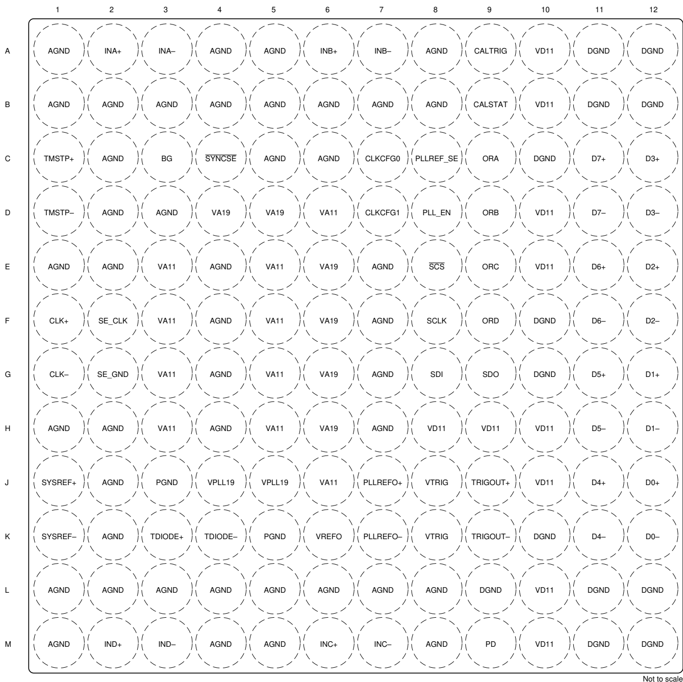
Figure 5-1. Quad Channel AAV Package, 144-Ball Flip Chip BGA (Top View)
