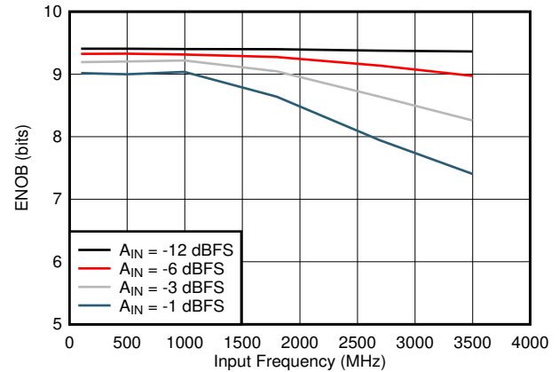
Figure 6-20. ENOB vs Input Frequency
