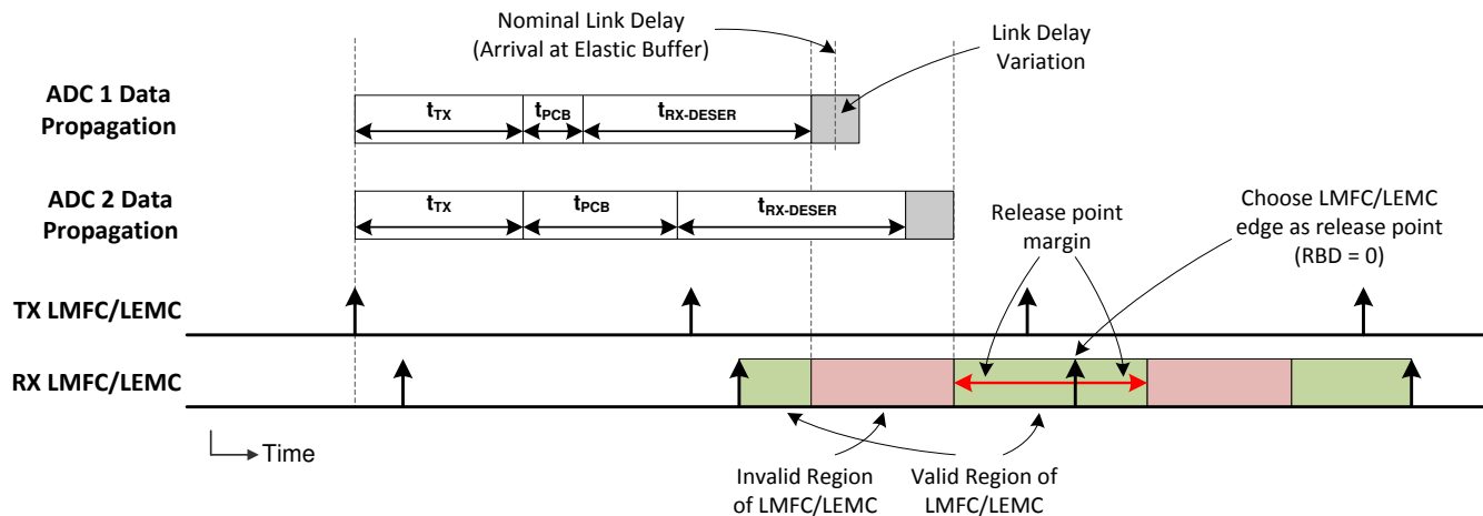
Figure 7-11. LMFC/LEMC Valid Region Definition for Elastic Buffer Release Point Selection
