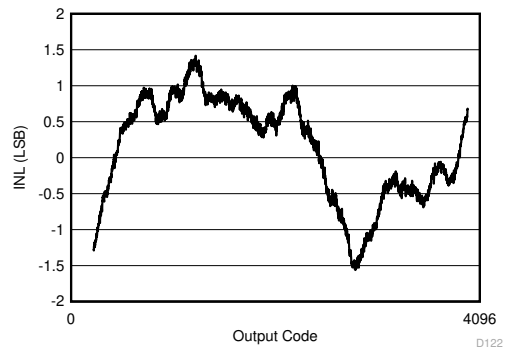
Figure 6-2. INL vs Code
