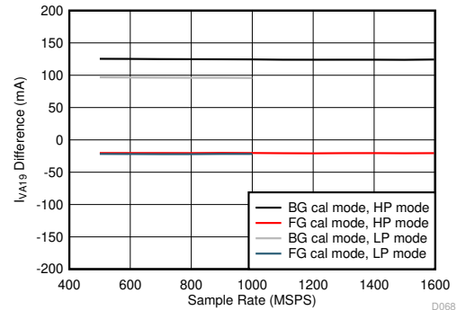
Figure 6-112. Quad Channel, I_{VA19} Change with Calibration Mode
