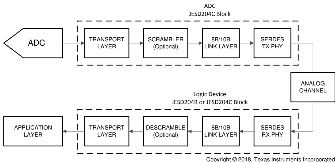
Figure 7-7. Simplified 8B/10B Encoded JESD204C Interface Diagram
