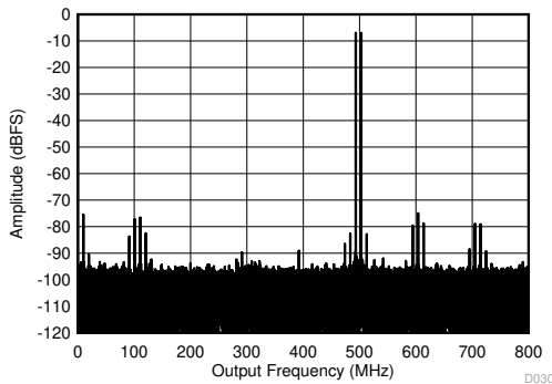
10MHz tone spacing Figure 6-69. Two Tone FFT at 498MHz
