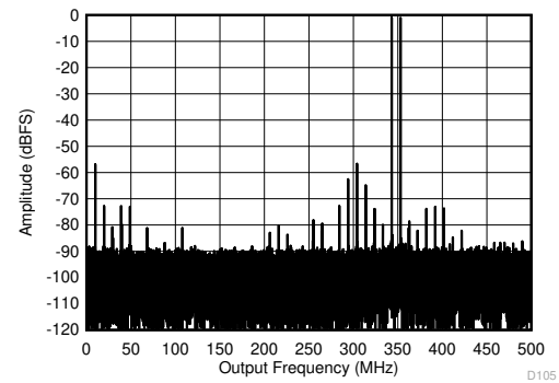
Figure 6-72. Two Tone FFT at 348 MHz 10 MHz tone spacing, -7 dBFS per tone, Low power mode, 1000MSPS
