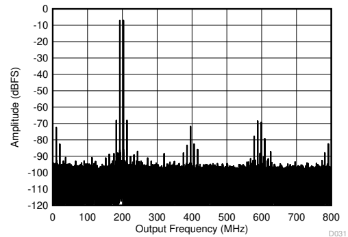
10MHz tone spacing Figure 6-70. Two Tone FFT at 1798MHz
