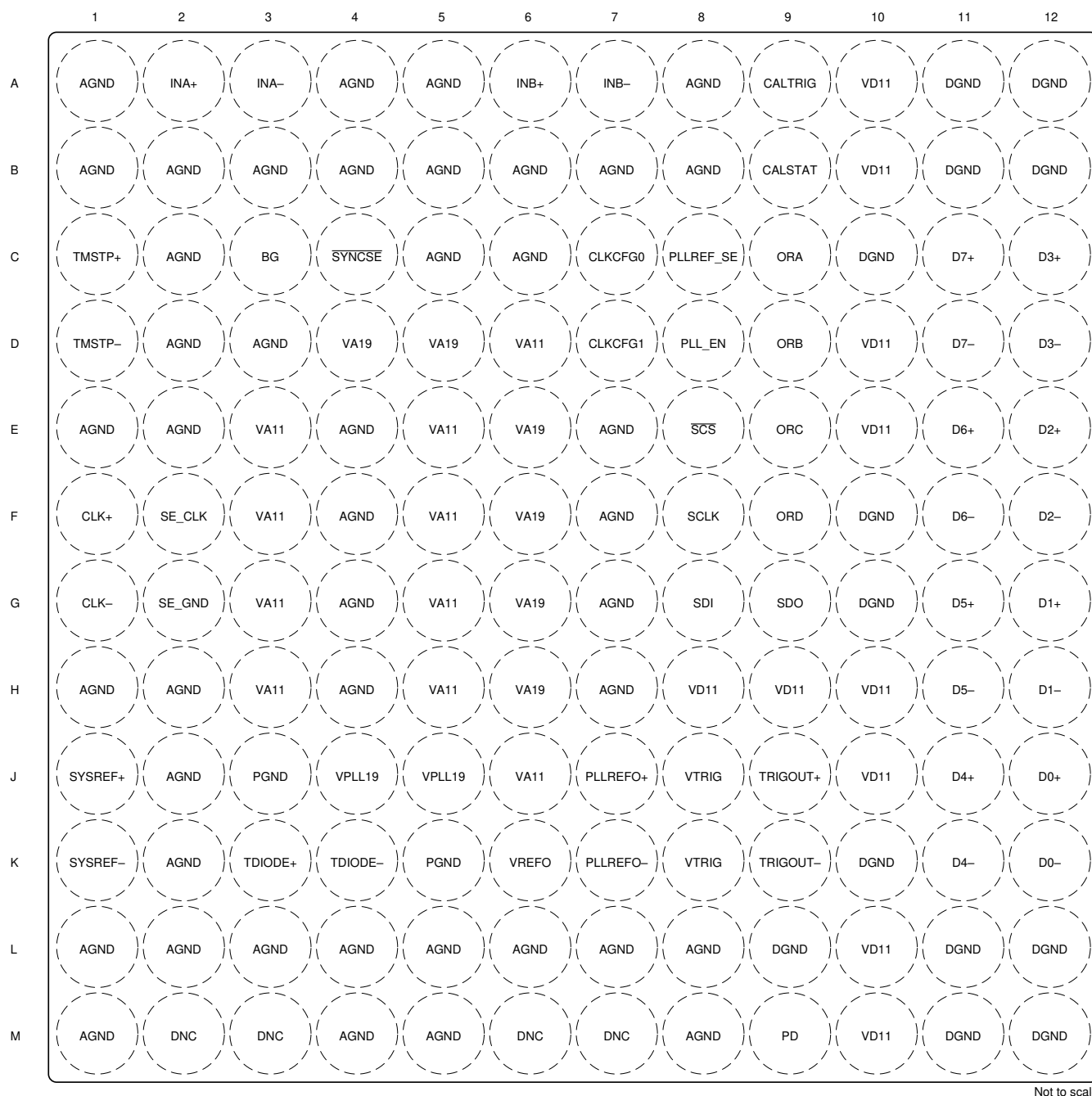
Figure 5-2. Dual Channel AAV Package, 144-Ball Flip Chip BGA (Top View)
