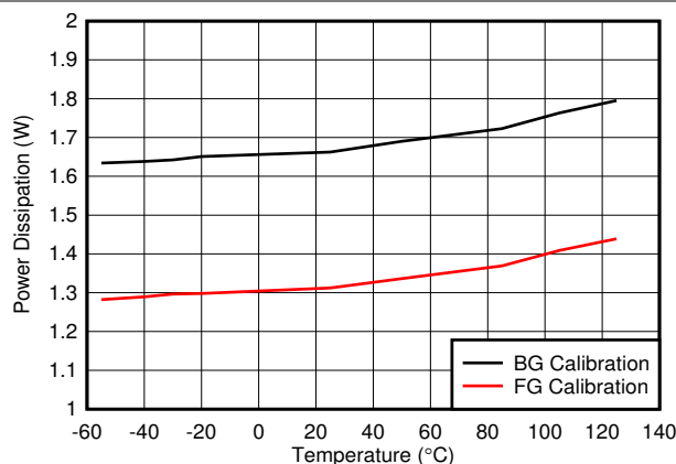
Figure 6-123. Single Channel, Power Dissipation vs Temperature
