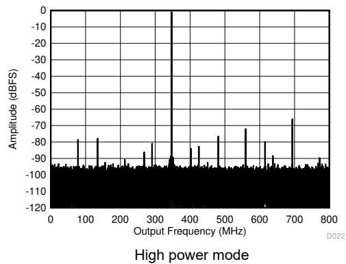
Figure 6-4. Single Tone FFT at 347 MHz and -1 dBFS
