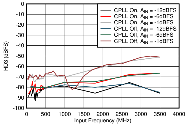
Figure 6-53. HD3 vs A_{IN} and C-PLL
