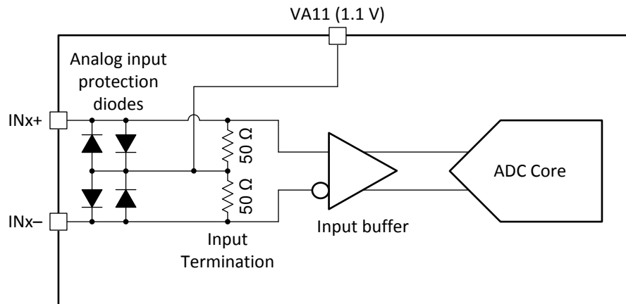
Figure 7-4. Analog Input Internal Termination and Protection Diagram
