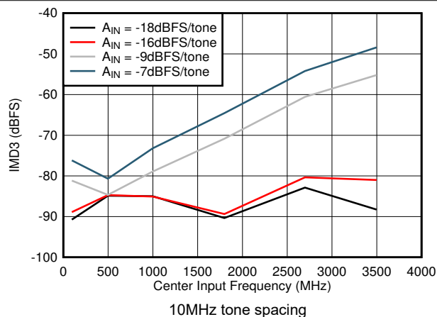
Figure 6-75. IMD3 vs F_{IN} 10MHz tone spacing
