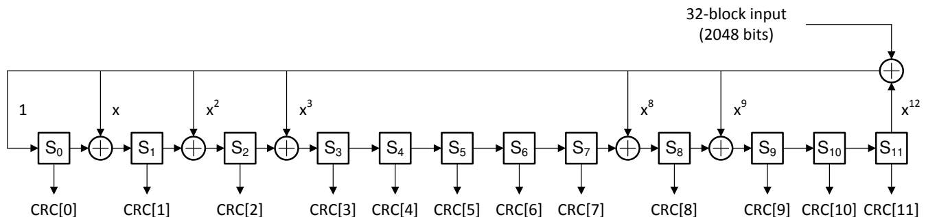
Figure 7-9. CRC-12 Parity Bit Generator
