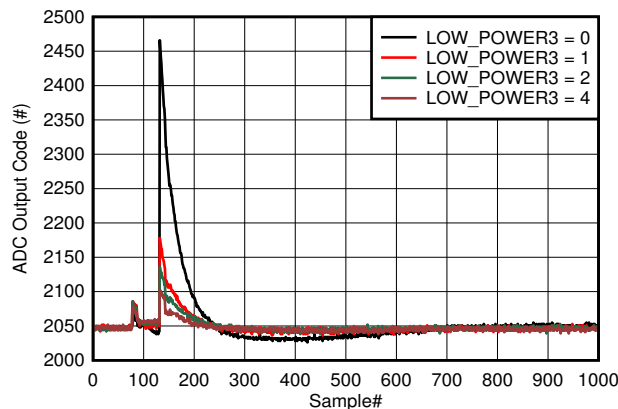
Figure 7-12. Background Calibration Core Transition In Low Power Mode
