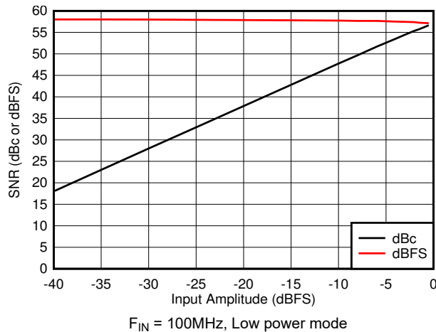
Figure 6-35. SNR vs A_{IN}
