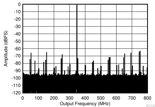
Figure 6-6. Single Tone FFT at 347 MHz and -1 dBFS
