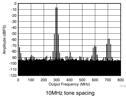
Figure 6-71. Two Tone FFT at 3498MHz
