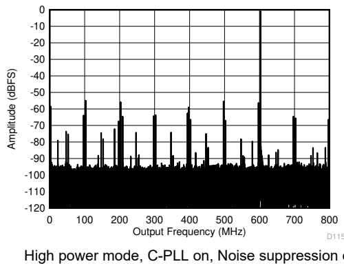
Figure 6-9. Single Tone FFT at 997 MHz and -1 dBFS
