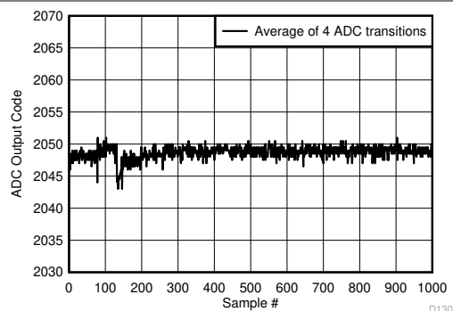
Figure 6-124. Background Calibration Core Transition (midscale voltage)
