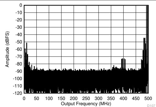
Figure 6-74. Two Tone FFT at 3498 MHz 10 MHz tone spacing, -7 dBFS per tone, Low power mode, 1000MSPS
