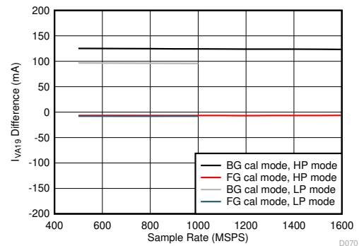
Figure 6-112. Quad Channel, I_{VA19} Change with Calibration Mode
