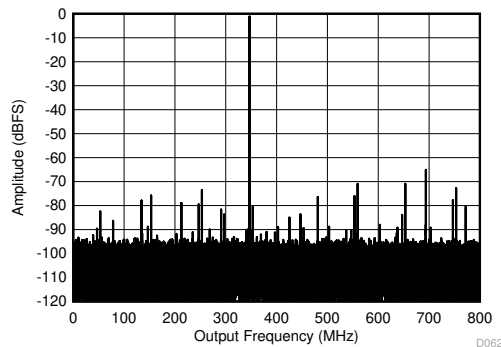
Figure 6-5. Single Tone FFT at 347 MHz and -1 dBFS
