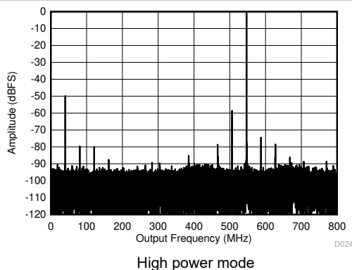
Figure 6-11. Single Tone FFT at 3797 MHz and -1 dBFS
