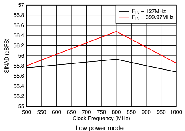
Figure 6-30. SINAD vs Sample Rate
