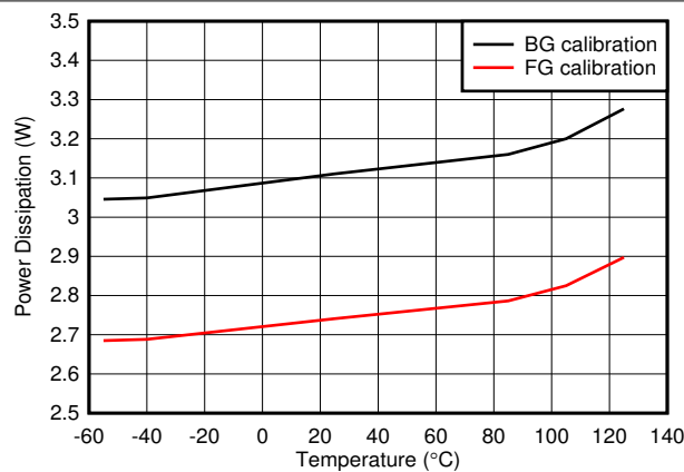
Figure 6-121. Quad Channel, Power Dissipation vs Temperature
