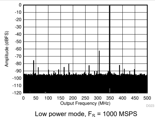
Figure 6-12. Single Tone FFT at 347 MHz and -1 dBFS
