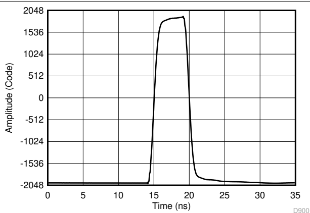
Figure 8-2. Measured Pulse using Sub-Sampling Technique for Equivalent 32 GSPS Measurement
