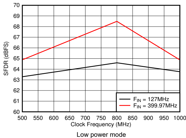
Figure 6-27. SFDR vs Sample Rate
