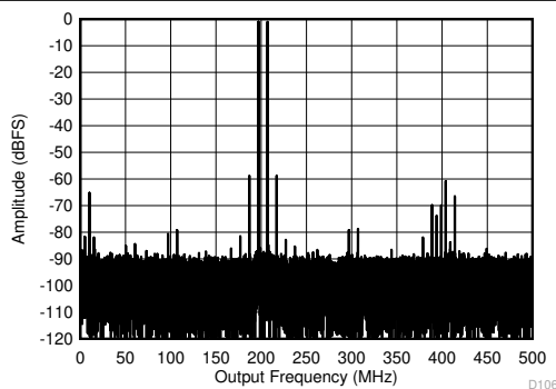
Figure 6-73. Two Tone FFT at 1798 MHz 10 MHz tone spacing, -7 dBFS per tone, Low power mode, 1000MSPS
