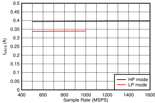
Figure 6-93. Dual Channel, I_{VA19} vs F_S
