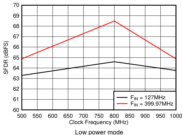
Figure 6-29. SFDR vs Sample Rate
