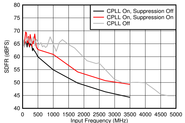
Figure 6-40. SFDR vs F_{IN} and C-PLL modes
