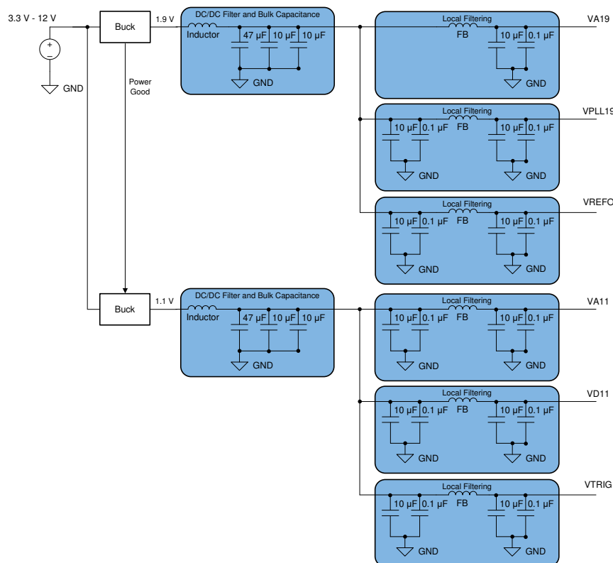
Figure 8-4. Switcher-Only Approach Example
