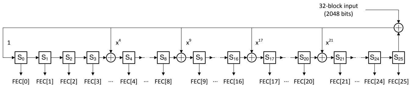
Figure 7-10. FEC Parity Bit Generator
