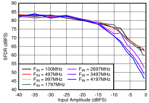
Figure 6-32. SFDR vs A_{IN}
