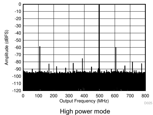
Figure 6-10. Single Tone FFT at 1797 MHz and -1 dBFS
