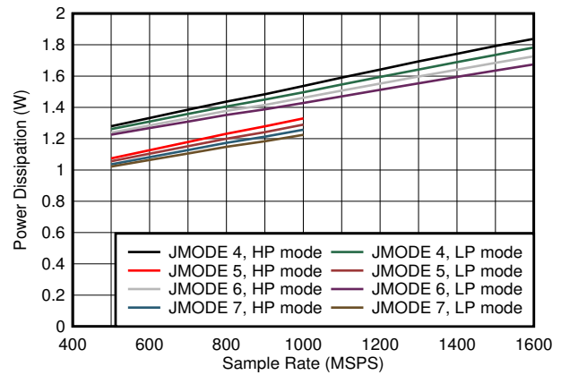
Figure 6-90. Dual Channel, Power Dissipation vs F_S and JMODE 4 - 7
