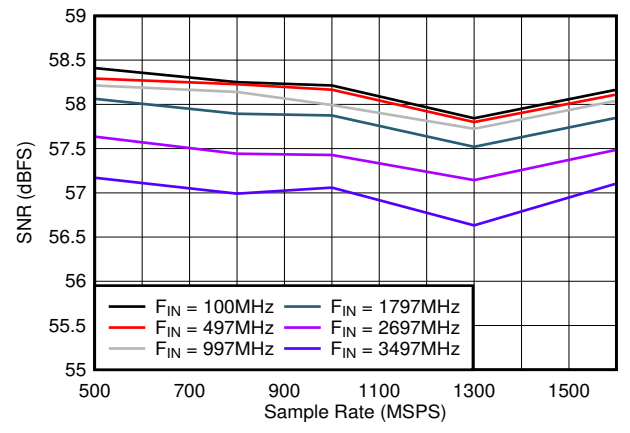
Figure 6-24. SNR vs Sample Rate
