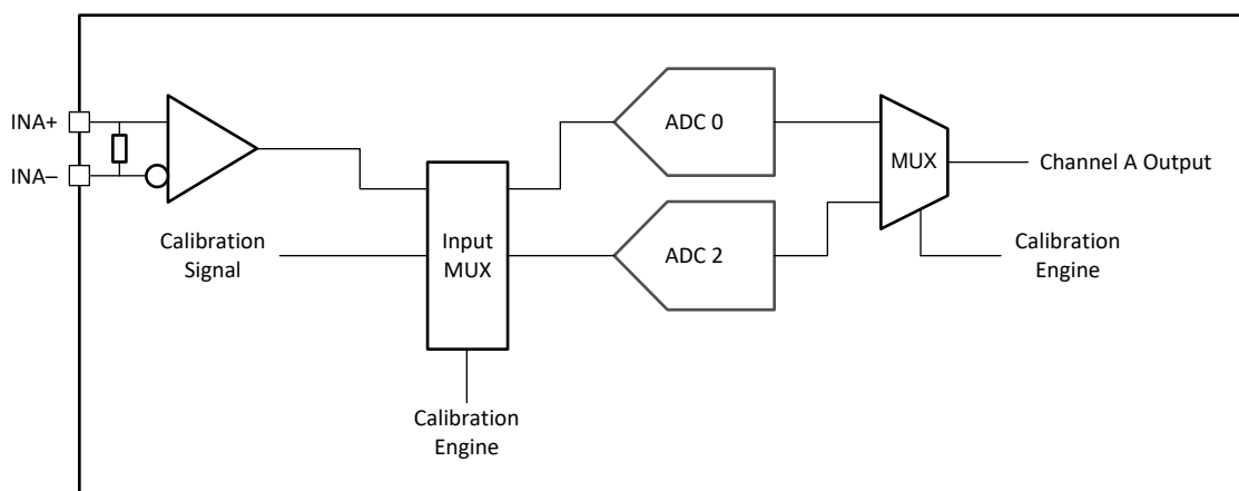
Figure 7-17. Single Channel Calibration System Block Diagram
