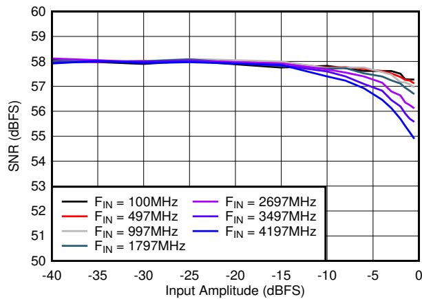
Figure 6-33. SNR vs A_{IN}
