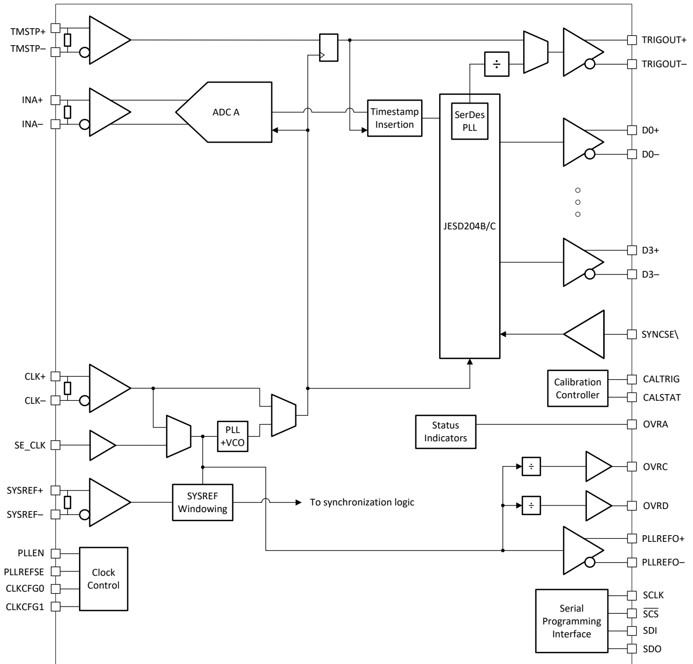
Figure 7-3. Single Channel Functional Block Diagram
