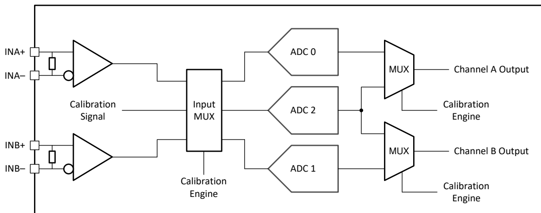
Figure 7-16. DualChannel Calibration System Block Diagram
