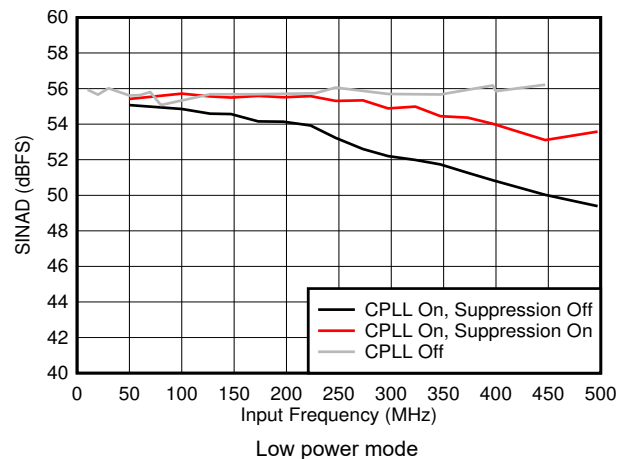
Figure 6-46. SINAD vs F_{IN} and C-PLL modes
