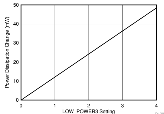
Figure 7-13. Power Dissipation Change vs LOW_POWER3 register setting
