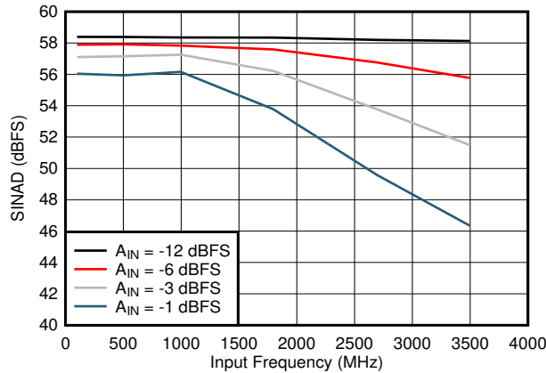
Figure 6-19. SINAD vs Input Frequency
