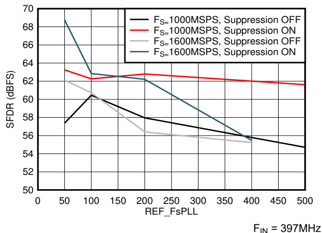
Figure 6-39. SFDR vs F_{REF} and Suppression
