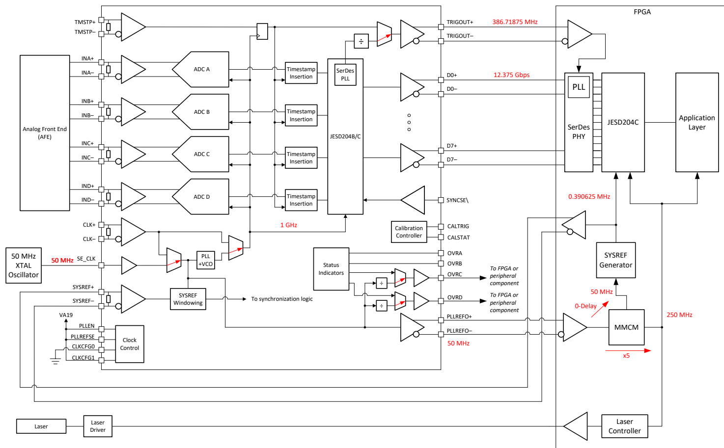
Figure 8-1. Typical Configuration for a LiDAR Digitizer
