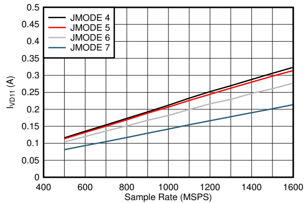
Figure 6-106. Single Channel, I_{VD11} vs F_S and JMODE 4 - 7
