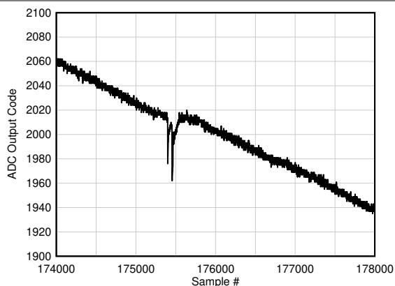
Figure 6-127. Background Calibration Core Transition (AC Signal Zoomed)
