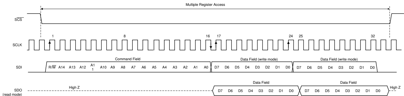
Figure 7-19. Serial Interface Protocol: Streaming Read/Write
