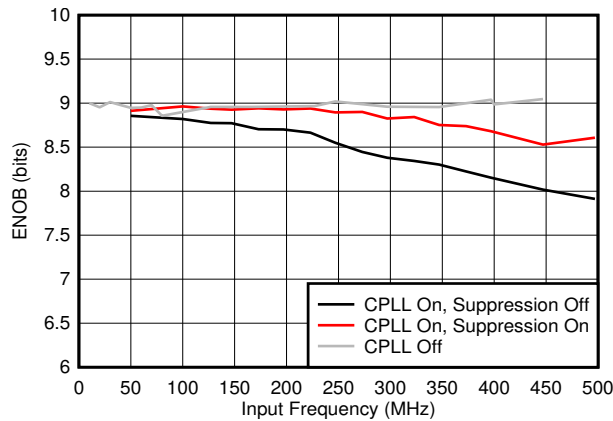
Figure 6-47. ENOB vs F_{IN} and C-PLL modes
