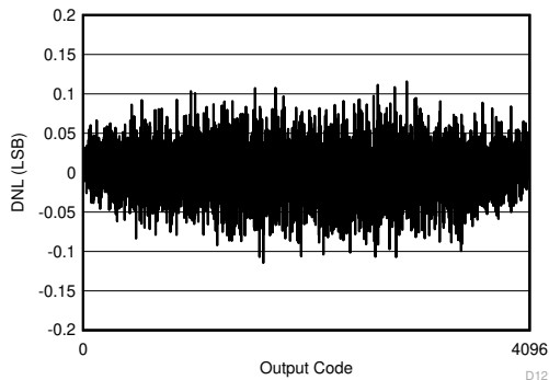
Figure 6-1. DNL vs Code
