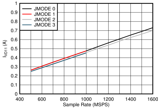
Figure 6-85. Quad Channel, I_{VD11} vs F_S and JMODE 0 - 3
