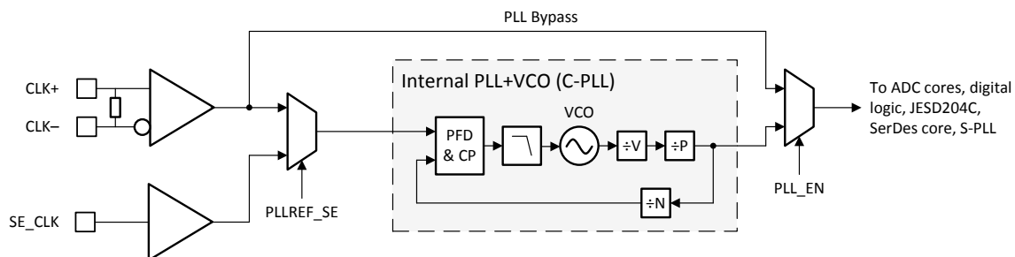
Figure 7-6. Converter PLL (C-PLL) Architecture
