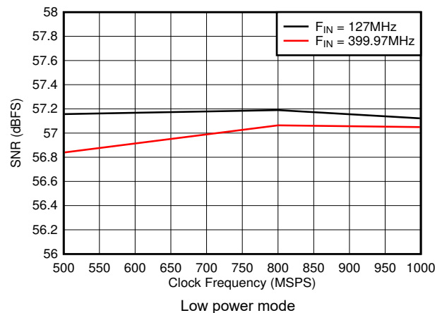
Figure 6-28. SNR vs Sample Rate
