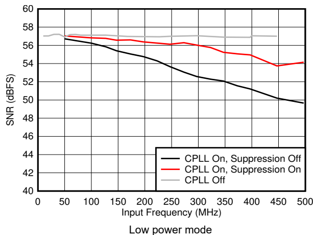
Figure 6-45. SNR vs F_{IN} and C-PLL modes
