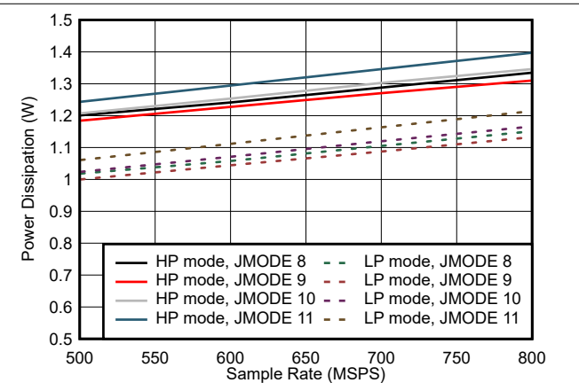
Figure 5-90. Dual Channel, Power Dissipation vs F_S for JMODES 8 - 11
