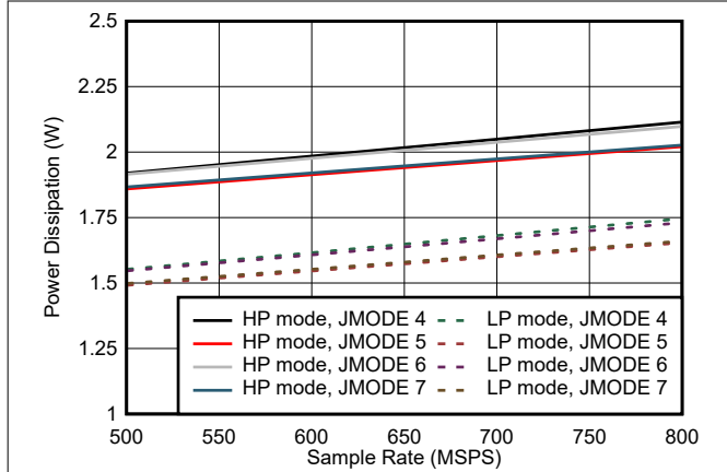
Figure 5-75. Quad Channel, Power Dissipation vs F_S for JMODES 4 - 7
