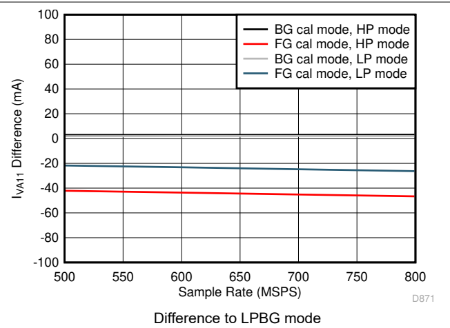
Figure 5-86. Quad Channel, I_{VA11} vs F_S over Modes
