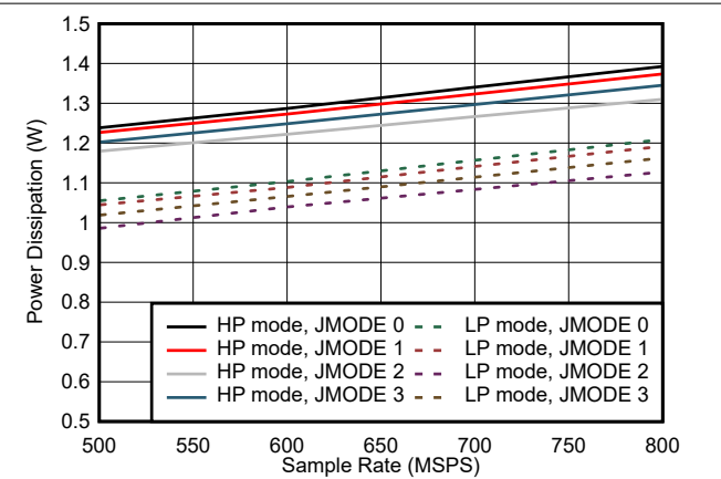
Figure 5-88. Dual Channel, Power Dissipation vs F_S for JMODES 0 - 3
