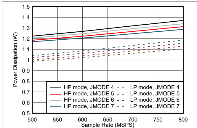
Figure 5-89. Dual Channel, Power Dissipation vs F_S for JMODES 4 - 7
