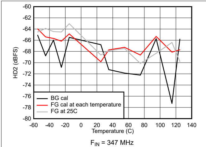
Figure 5-45. HD2 vs Temperature
